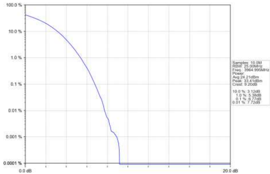
n77a_15kHz_SISO_NTNV_30MHz_DFT-s-OFDM_64_QAM_3964.995MHz_Outer_Full_Ant1
