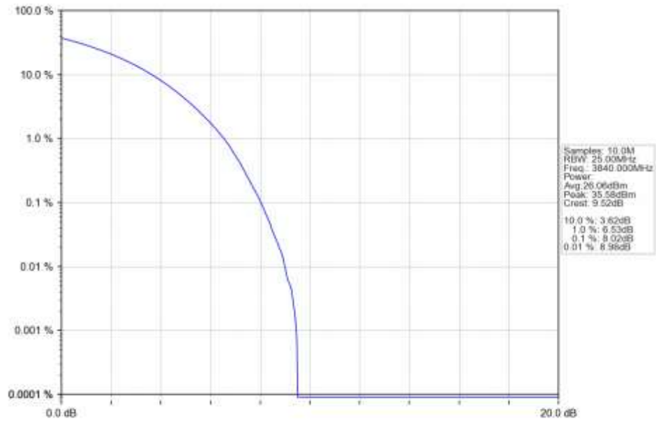
n77a_15kHz_SISO_NTNV_30MHz_CP-OFDM_16_QAM_3840MHz_Outer_Full_Ant1
