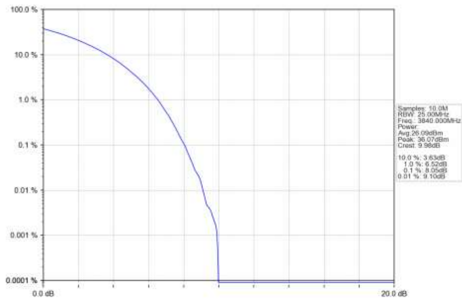
n77a_15kHz_SISO_NTNV_30MHz_CP-OFDM_QPSK_3840MHz_Outer_Full_Ant1
