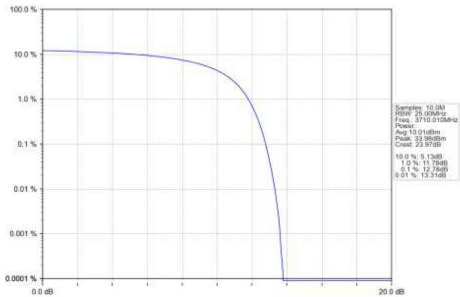
n77a 30kHz SISO NTN 20MHz CP-OFDM 16 QAM 3710.01MHz Outer Full Ant1
