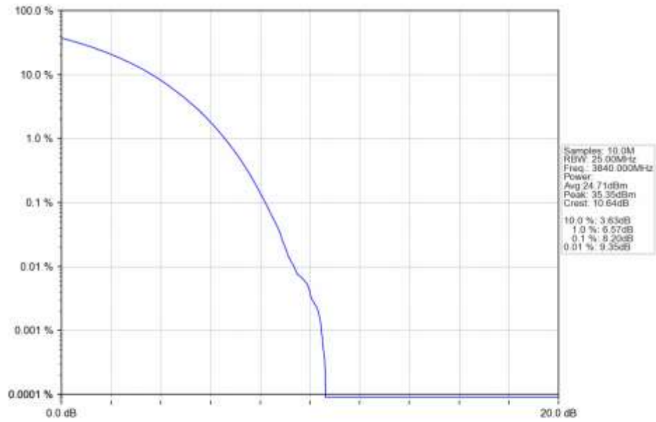
n77a_15kHz_SISO_NTNV_40MHz_CP-OFDM_16_QAM_3840MHz_Outer_Full_Ant1
