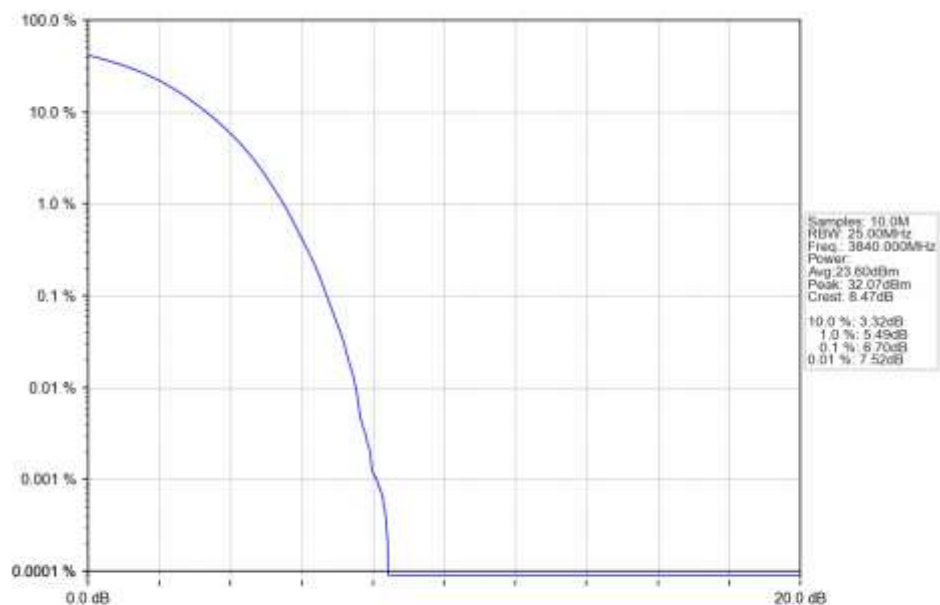
n77a_15kHz_SISO_NTNV_50MHz_DFT-s-OFDM_QPSK_3840MHz_Outer_Full_Ant1
