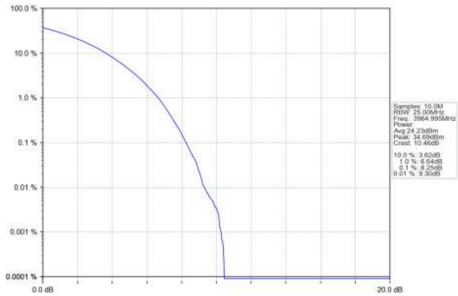
n77a_15kHz_SISO_NTNV_30MHz_CP-OFDM_16_QAM_3964.995MHz_Outer_Full_Ant1
