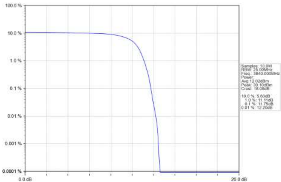
n77a_30kHz_SISO_NTNV_15MHz_DFT-s-OFDM QPSK_3840MHz_Outer_Full_Ant1
