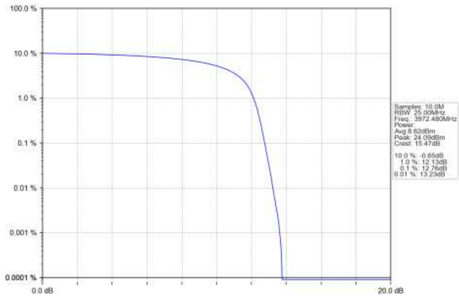
n77a 30kHz SISO NTN 15MHz CP-OFDM QPSK 3972.48MHz Outer Full Ant1
