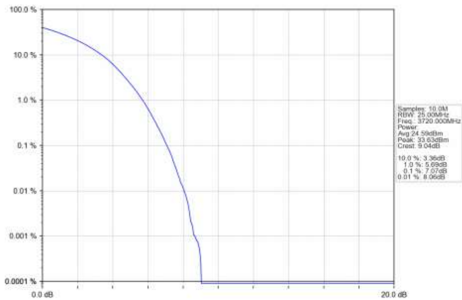
n77a_15kHz_SISO_NTNV_40MHz_DFT-s-OFDM_256_QAM_3720MHz_Outer_Full_Ant1
