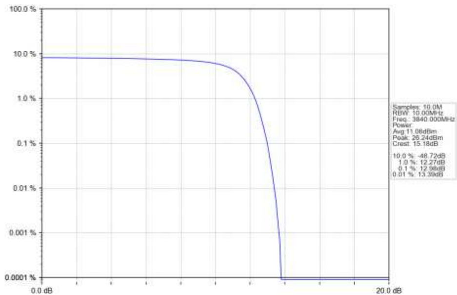
n77a_30kHz_SISO_NTNV_10MHz_DFT-s-OFDM QPSK_3840MHz_Outer_Full_Ant1
