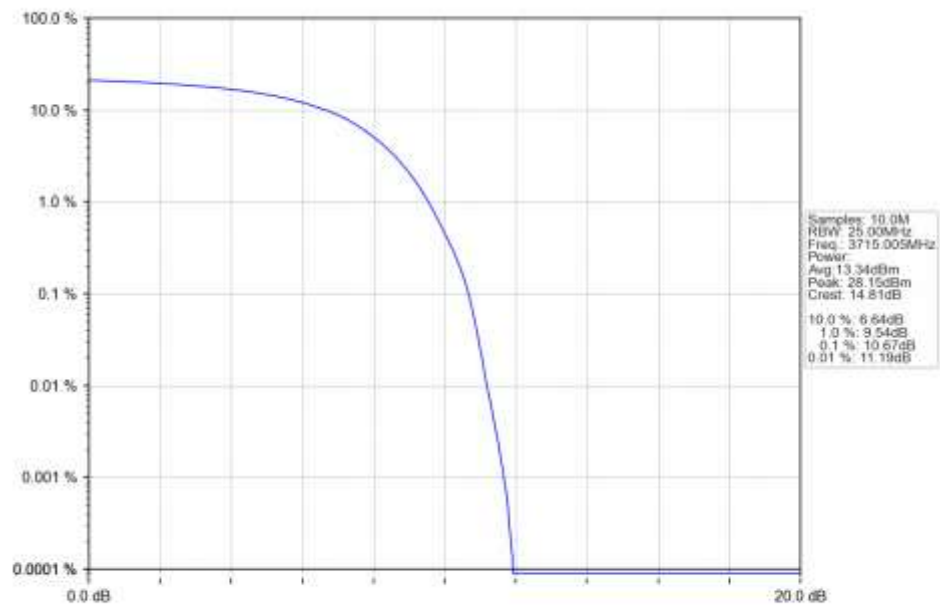
n77a_15kHz_SISO_NTNV_30MHz_DFT-s-OFDM QPSK_3715.005MHz_Outer_Full_Ant1
