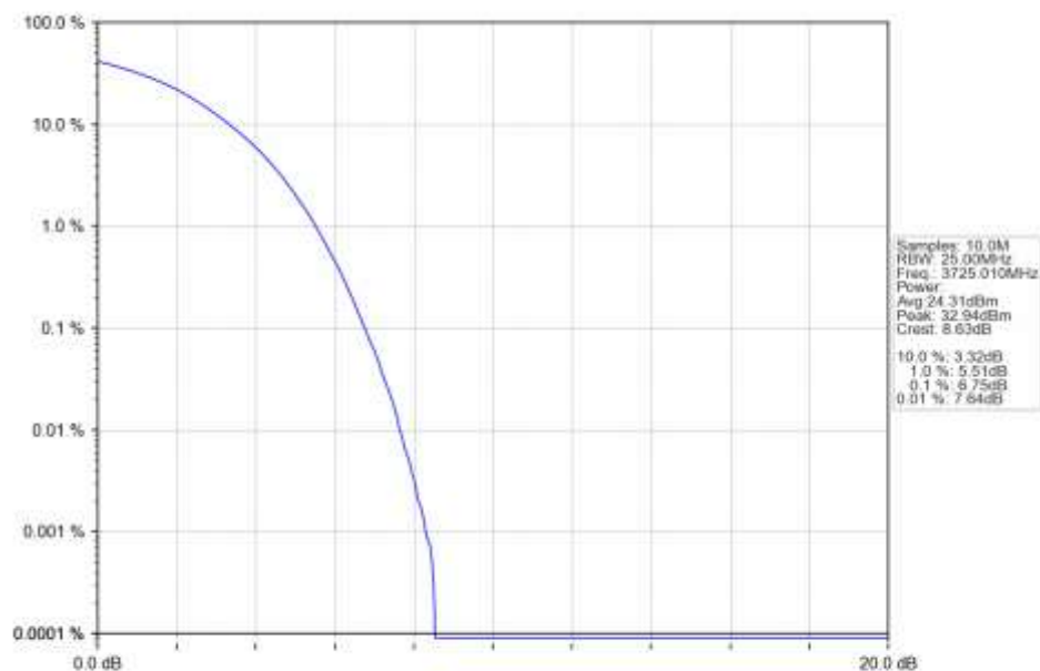
n77a_15kHz_SISO_NTNV_50MHz_DFT-s-OFDM_QPSK_3725.01MHz_Outer_Full_Ant1
