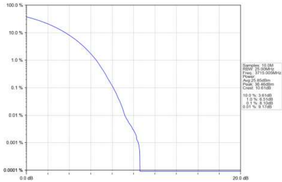
n77a_15kHz_SISO_NTNV_30MHz_CP-OFDM_64_QAM_3715.005MHz_Outer_Full_Ant1
