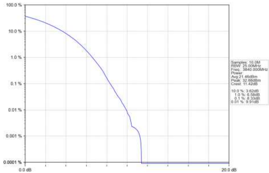
n77a_15kHz_SISO_NTNV_40MHz_CP-OFDM_256_QAM_3840MHz_Outer_Full_Ant1
