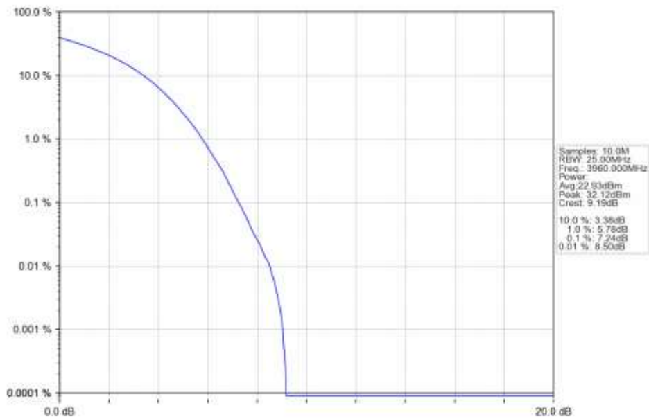
n77a_15kHz_SISO_NTNV_40MHz_DFT-s-OFDM_64_QAM_3960MHz_Outer_Full_Ant1
