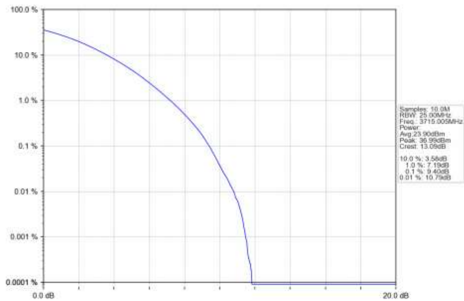
n77a_15kHz_SISO_NTNV_30MHz_CP-OFDM_16_QAM_3715.005MHz_Outer_Full_Ant1
