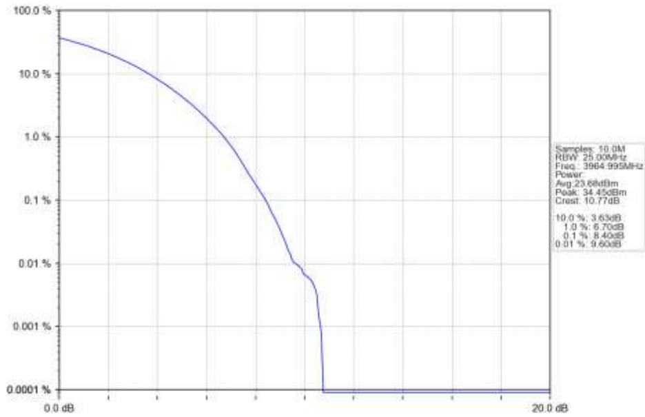
n77a_15kHz_SISO_NTNV_30MHz_CP-OFDM_64_QAM_3964.995MHz_Outer_Full_Ant1
