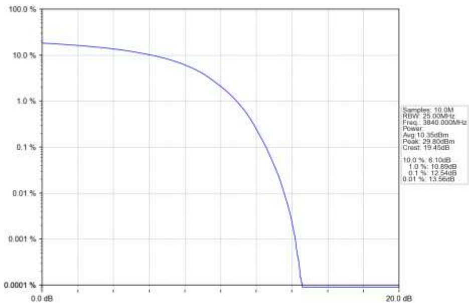
n77a_15kHz_SISO_NTNV_50MHz_DFT-s-OFDM QPSK_3840MHz_Outer_Full_Ant1
