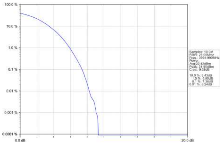
n77a_15kHz_SISO_NTNV_50MHz_DFT-s-OFDM_16_QAM_3954.99MHz_Outer_Full_Ant1
