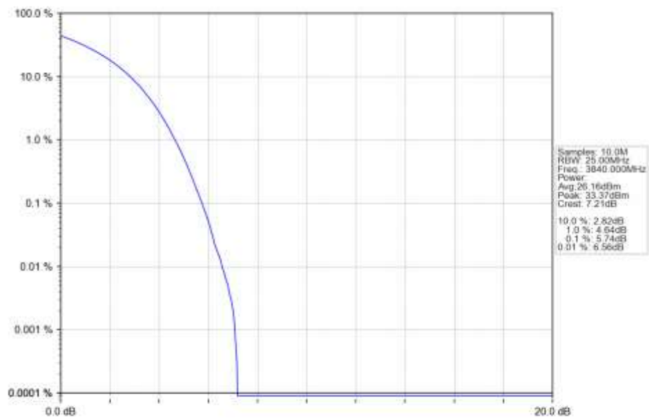
n77a_15kHz_SISO_NTNV_30MHz_DFT-s-OFDM_QPSK_3840MHz_Outer_Full_Ant1
