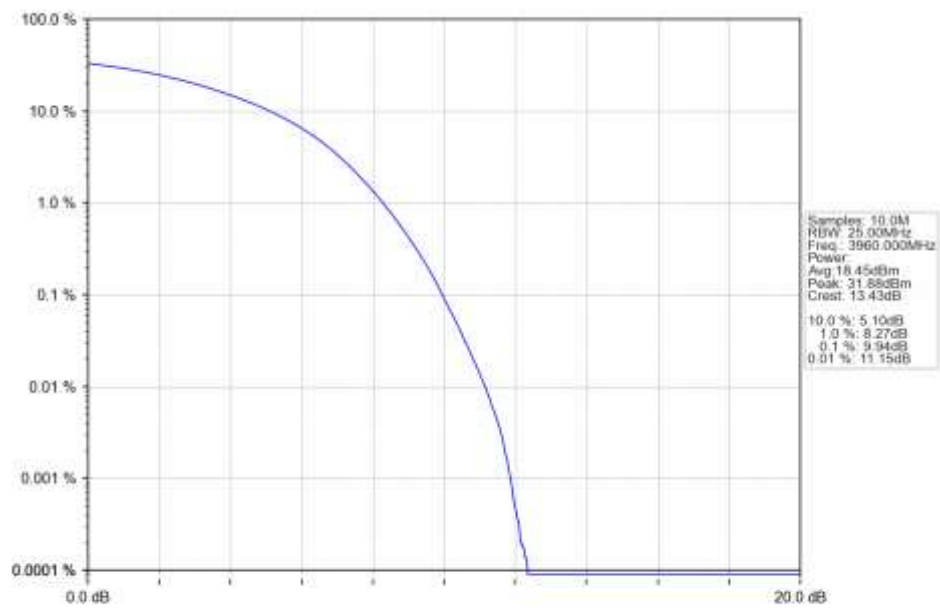
n77a_15kHz_SISO_NTNV_40MHz_DFT-s-OFDM_256_QAM_3960MHz_Outer_Full_Ant1
