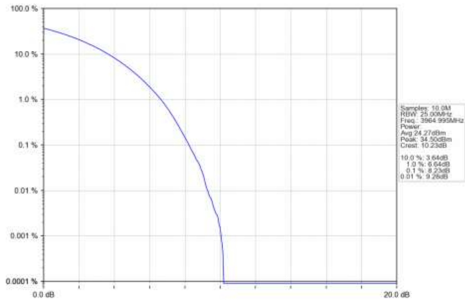
n77a_15kHz_SISO_NTNV_30MHz_CP-OFDM_QPSK_3964.995MHz_Outer_Full_Ant1
