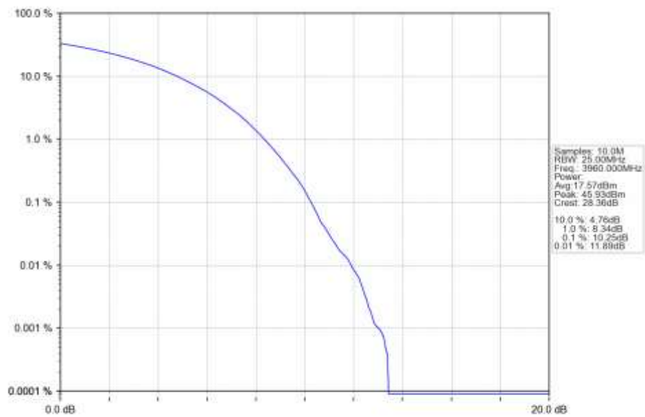
n77a_15kHz_SISO_NTNV_40MHz_CP-OFDM_256_QAM_3960MHz_Outer_Full_Ant1
