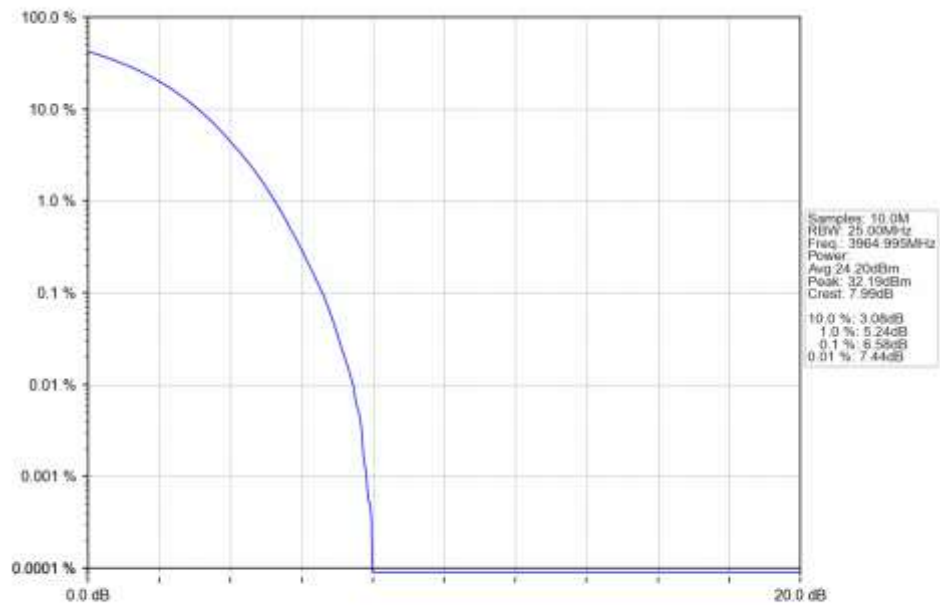
n77a 15kHz SISO NTN 30MHz DFT-s-OFDM 16 QAM 3964.995MHz Outer Full Ant1
