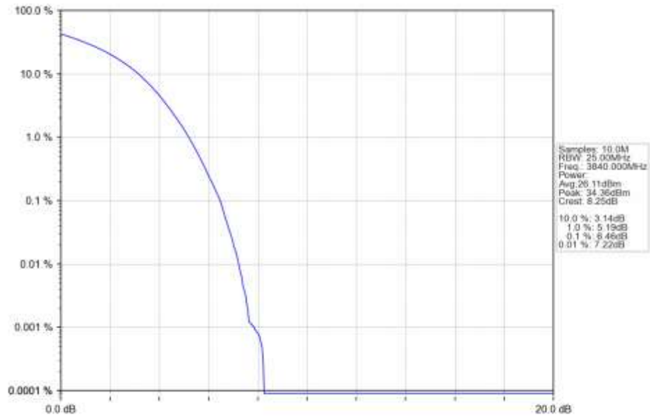
n77a 15kHz SISO NTN 30MHz DFT-s-OFDM 16 QAM 3840MHz Outer Full Ant1
