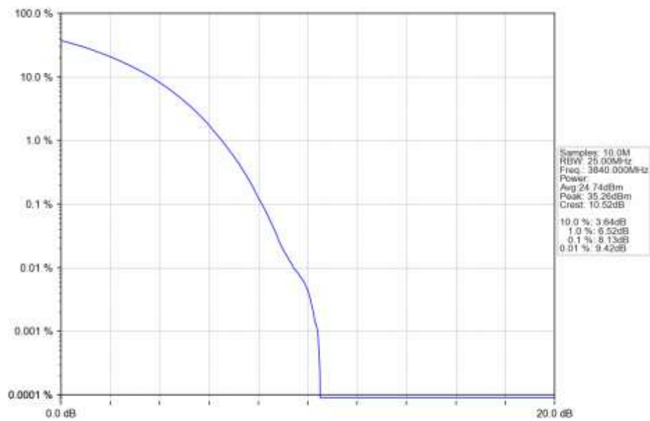
n77a_15kHz_SISO_NTNV_40MHz_CP-OFDM_QPSK_3840MHz_Outer_Full_Ant1
