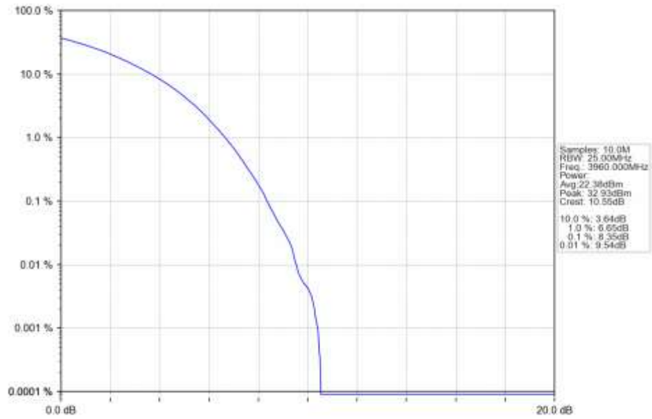
n77a_15kHz_SISO_NTNV_40MHz_CP-OFDM_64_QAM_3960MHz_Outer_Full_Ant1
