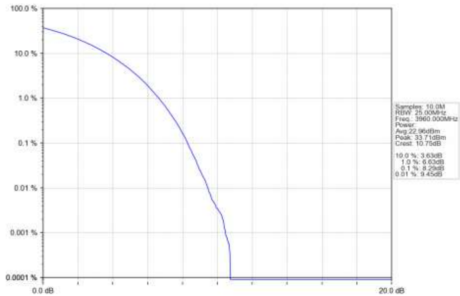
n77a_15kHz_SISO_NTNV_40MHz_CP-OFDM_16_QAM_3960MHz_Outer_Full_Ant1
