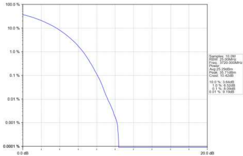
n77a_15kHz_SISO_NTNV_40MHz_CP-OFDM_QPSK_3720MHz_Outer_Full_Ant1
