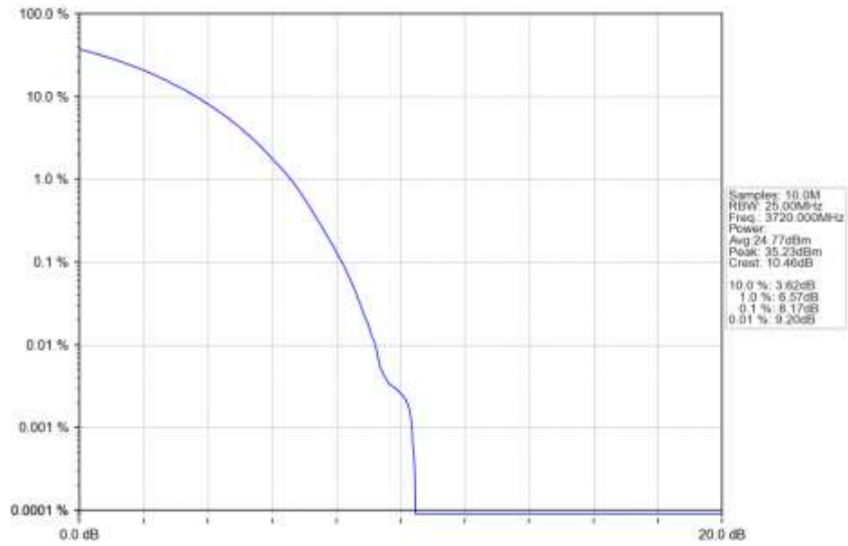
n77a_15kHz_SISO_NTNV_40MHz_CP-OFDM_64_QAM_3720MHz_Outer_Full_Ant1
