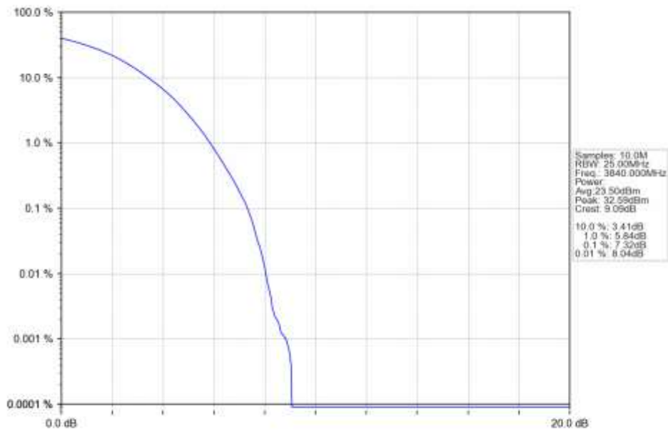
n77a_15kHz_SISO_NTNV_50MHz_DFT-s-OFDM_16_QAM_3840MHz_Outer_Full_Ant1
