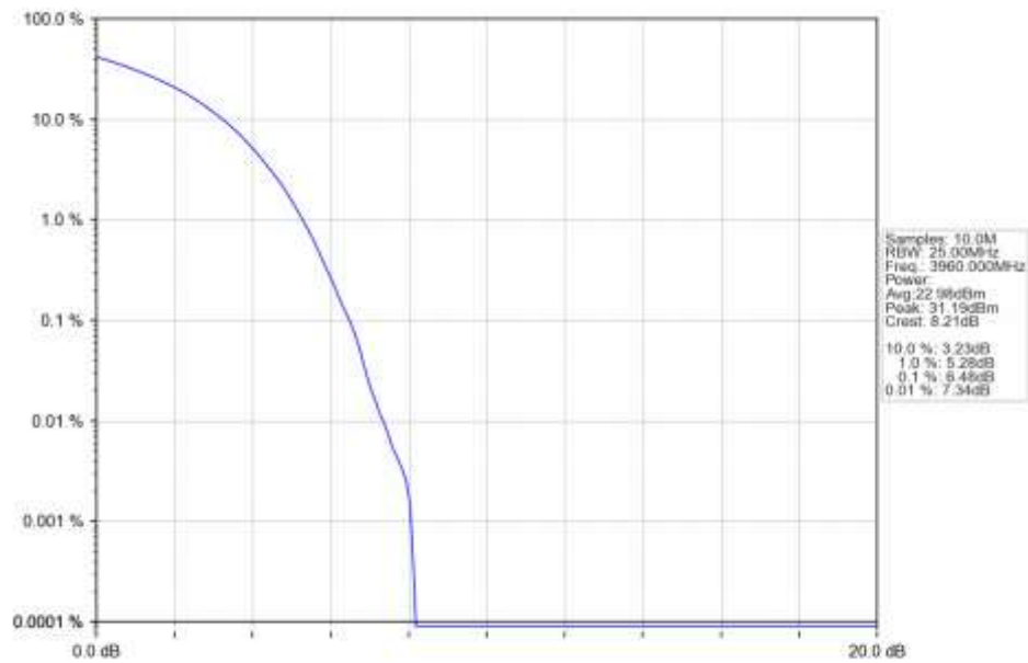
n77a_15kHz_SISO_NTNV_40MHz_DFT-s-OFDM_QPSK_3960MHz_Outer_Full_Ant1
