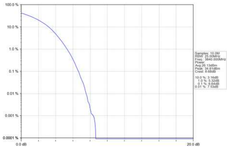
n77a_15kHz_SISO_NTNV_30MHz_DFT-s-OFDM_64_QAM_3840MHz_Outer_Full_Ant1
