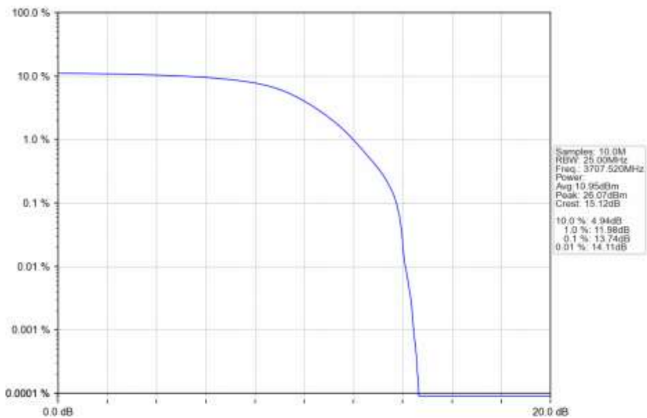
n77a_30kHz_SISO_NTNV_15MHz_DFT-s-OFDM QPSK_3707.52MHz_Outer_Full_Ant1
