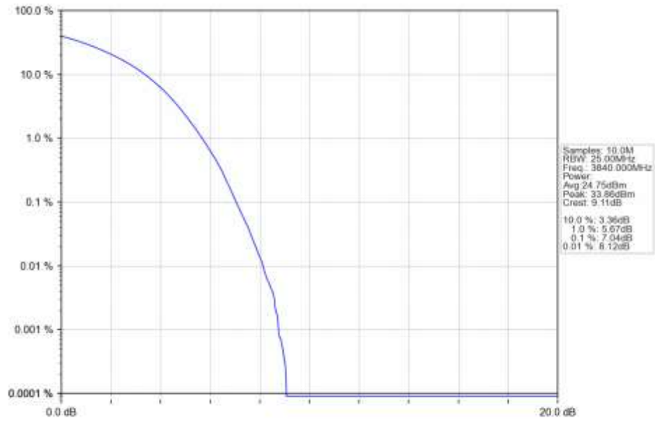
n77a_15kHz_SISO_NTNV_40MHz_DFT-s-OFDM_16_QAM_3840MHz_Outer_Full_Ant1
