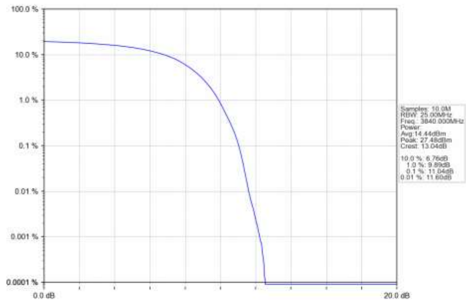
n77a_15kHz_SISO_NTNV_30MHz_DFT-s-OFDM QPSK_3840MHz_Outer_Full_Ant1
