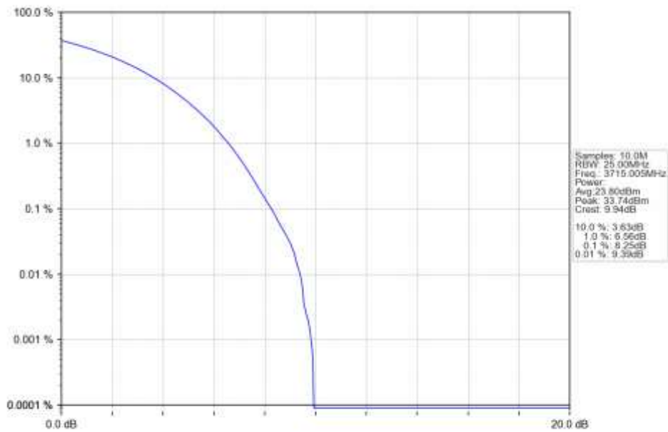
n77a_15kHz_SISO_NTNV_30MHz_CP-OFDM_256_QAM_3715.005MHz_Outer_Full_Ant1
