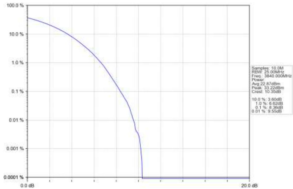
n77a_15kHz_SISO_NTNV_30MHz_CP-OFDM_256_QAM_3840MHz_Outer_Full_Ant1
