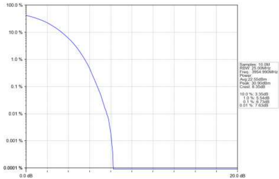
n77a_15kHz_SISO_NTNV_50MHz_DFT-s-OFDM_QPSK_3954.99MHz_Outer_Full_Ant1
