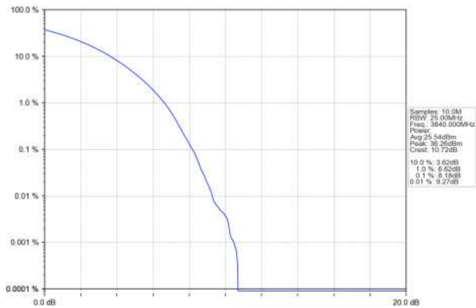
n77a_15kHz_SISO_NTNV_30MHz_CP-OFDM_64_QAM_3840MHz_Outer_Full_Ant1
