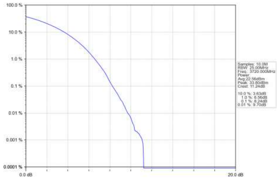
n77a_15kHz_SISO_NTNV_40MHz_CP-OFDM_256_QAM_3720MHz_Outer_Full_Ant1
