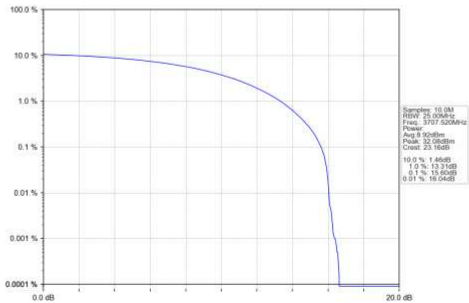
n77a 30kHz SISO NTN 15MHz CP-OFDM 16 QAM 3707.52MHz Outer Full Ant1
