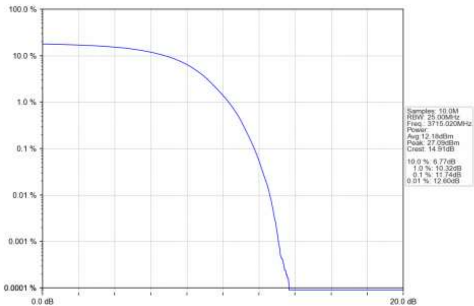
n77a_30kHz_SISO_NTNV_30MHz_DFT-s-OFDM QPSK_3715.02MHz_Outer_Full_Ant1
