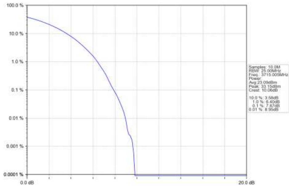
n77a_15kHz_SISO_NTNV_30MHz_CP-OFDM_QPSK_3715.005MHz_Outer_Full_Ant1
