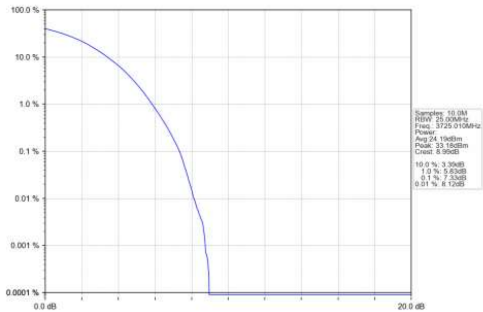
n77a_15kHz_SISO_NTNV_50MHz_DFT-s-OFDM_16_QAM_3725.01MHz_Outer_Full_Ant1
