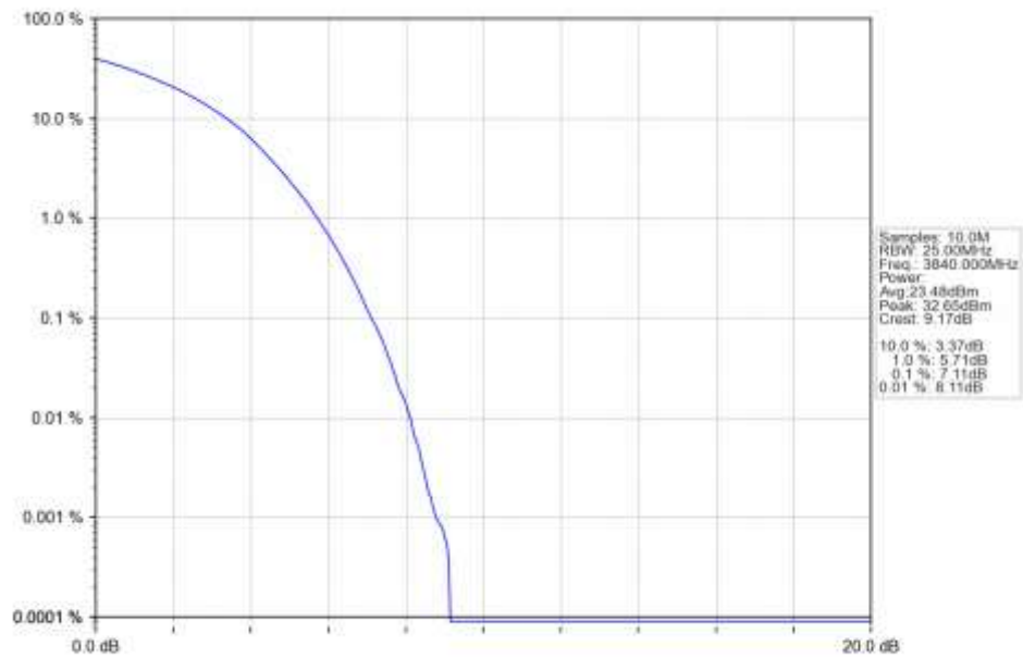
n77a_15kHz_SISO_NTNV_40MHz_DFT-s-OFDM_256_QAM_3840MHz_Outer_Full_Ant1
