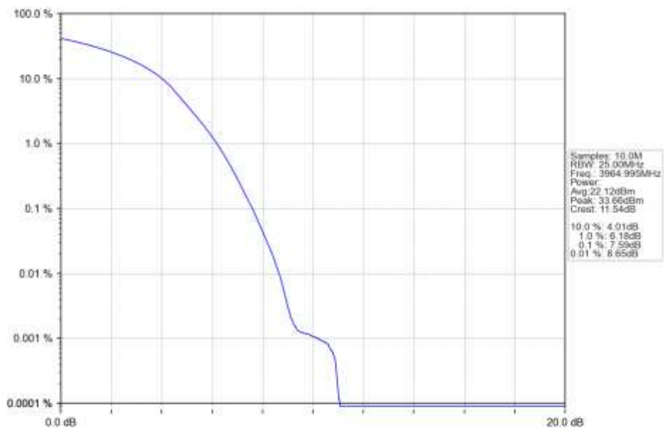
n77a_15kHz_SISO_NTNV_30MHz_DFT-s-OFDM_256_QAM_3964.995MHz_Outer_Full_Ant1
