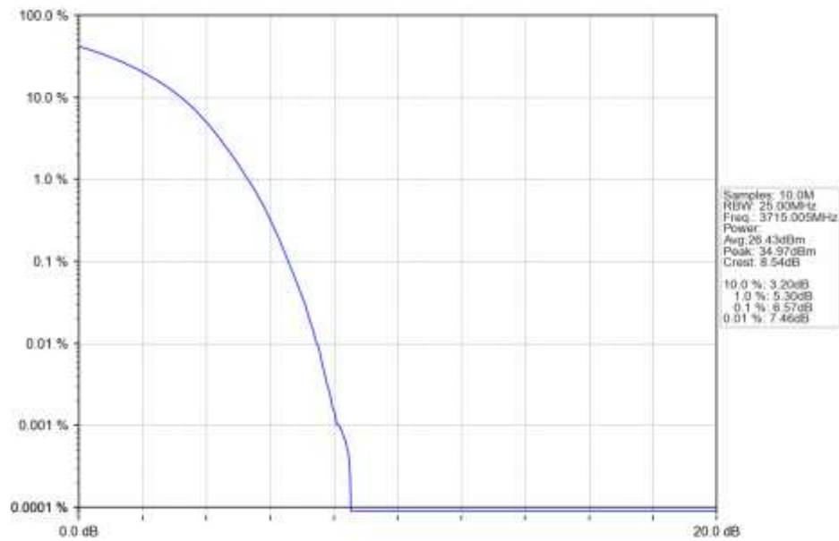
n77a_15kHz_SISO_NTNV_30MHz_DFT-s-OFDM_64_QAM_3715.005MHz_Outer_Full_Ant1
