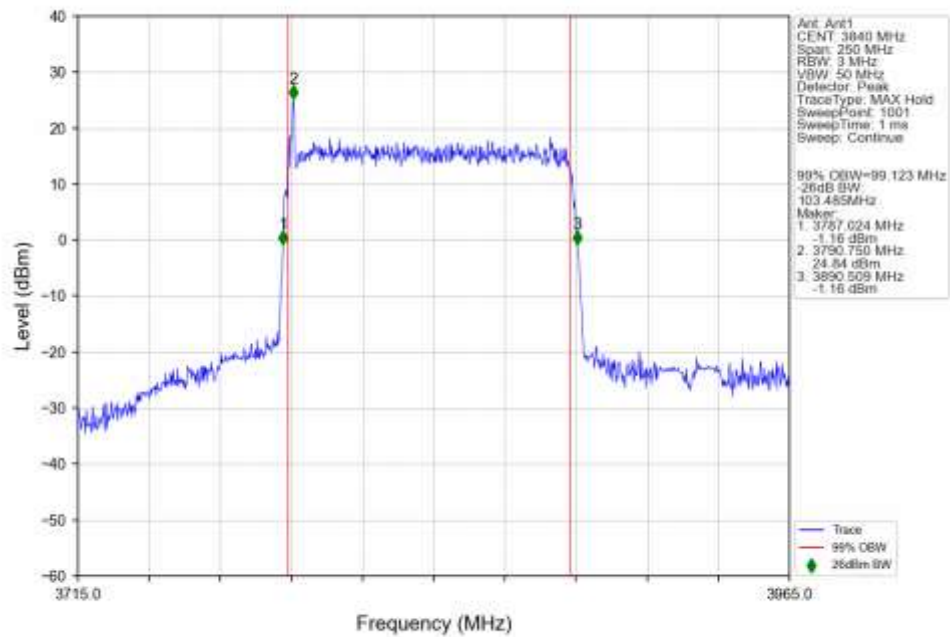
n77a_30kHz_SISO_NTNV_100MHz_DFT-s-OFDM QPSK_3840MHz_Outer_Full_Ant1
