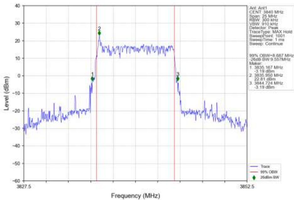
n77a_30kHz_SISO_NTNV_10MHz_DFT-s-OFDM QPSK_3840MHz_Outer_Full_Ant1
