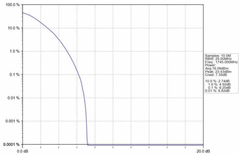
n66_15kHz_SISO_NTNV_15MHz_DFT-s-OFDM 64 QAM_1745MHz_Outer_Full_Ant1
