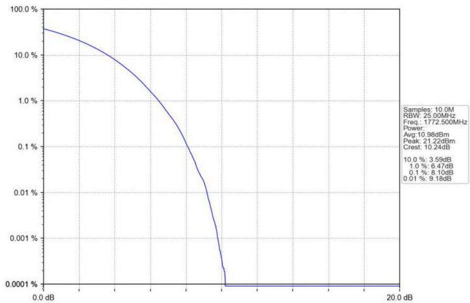
n66_15kHz_SISO_NTNV_15MHz_CP-OFDM 256 QAM_1772.5MHz_Outer_Full_Ant1
