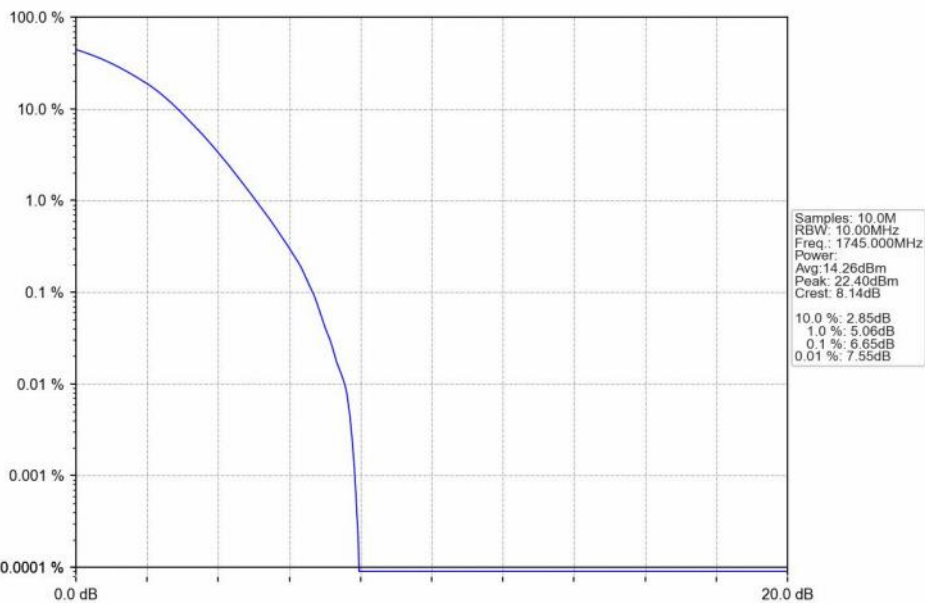
n66_30kHz_SISO_NTNV_10MHz_DFT-s-OFDM_256_QAM_1745MHz_Outer_Full_Ant1
