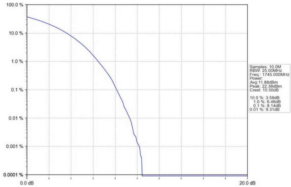
n66_15kHz_SISO_NTNV_15MHz_CP-OFDM 256 QAM_1745MHz_Outer_Full_Ant1
