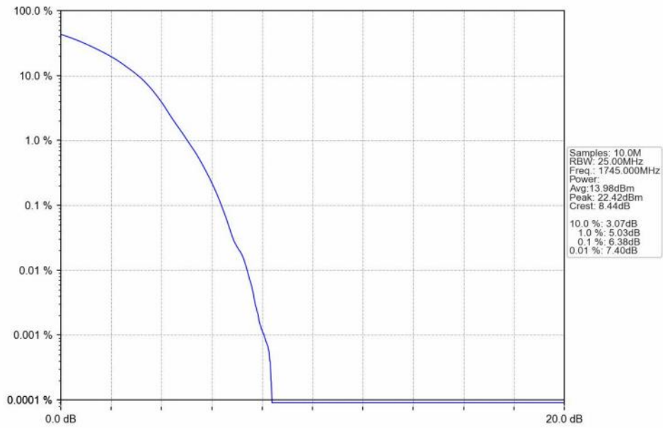
n66_15kHz_SISO_NTNV_25MHz_DFT-s-OFDM_256_QAM_1745MHz_Outer_Full_Ant1
