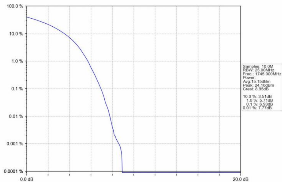
n66_15kHz_SISO_NTNV_45MHz_DFT-s-OFDM 64 QAM_1745MHz_Outer_Full_Ant1
