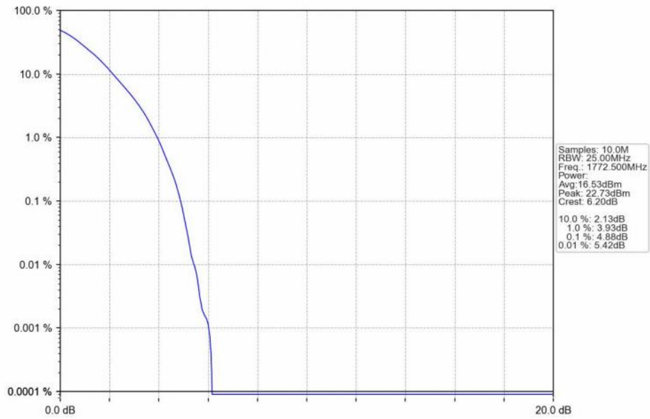
n66_15kHz_SISO_NTNV_15MHz_DFT-s-OFDM QPSK_1772.5MHz_Outer_Full_Ant1
