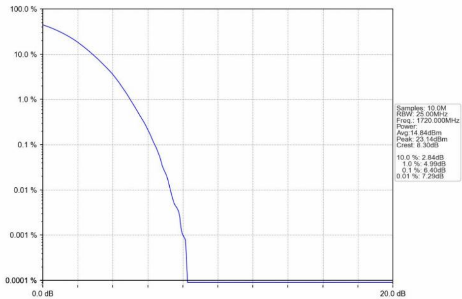
n66_30kHz_SISO_NTNV_20MHz_DFT-s-OFDM 256 QAM_1720MHz_Outer_Full_Ant1
