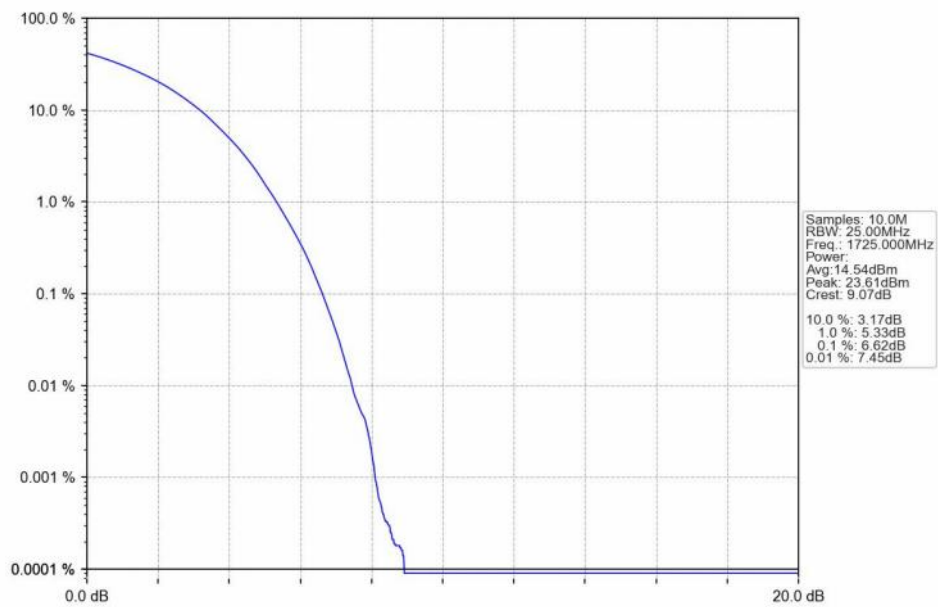
n66_15kHz_SISO_NTNV_30MHz_DFT-s-OFDM 256 QAM_1725MHz_Outer_Full_Ant1
