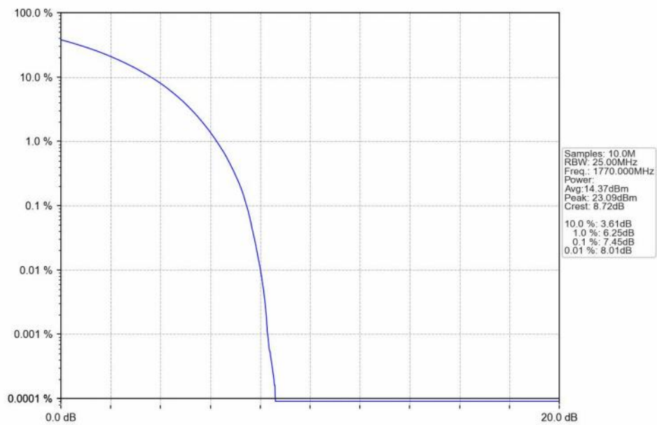
n66_15kHz_SISO_NTNV_20MHz_CP-OFDM_16_QAM_1770MHz_Outer_Full_Ant1
