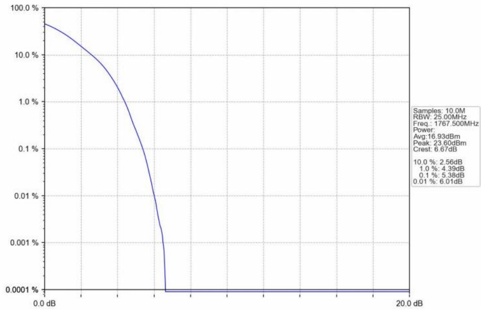
n66_15kHz_SISO_NTNV_25MHz_DFT-s-OFDM QPSK_1767.5MHz_Outer_Full_Ant1
