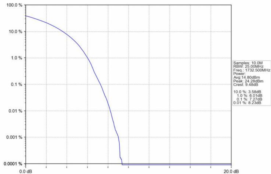
n66_15kHz_SISO_NTNV_45MHz_DFT-s-OFDM 64 QAM_1732.5MHz_Outer_Full_Ant1
