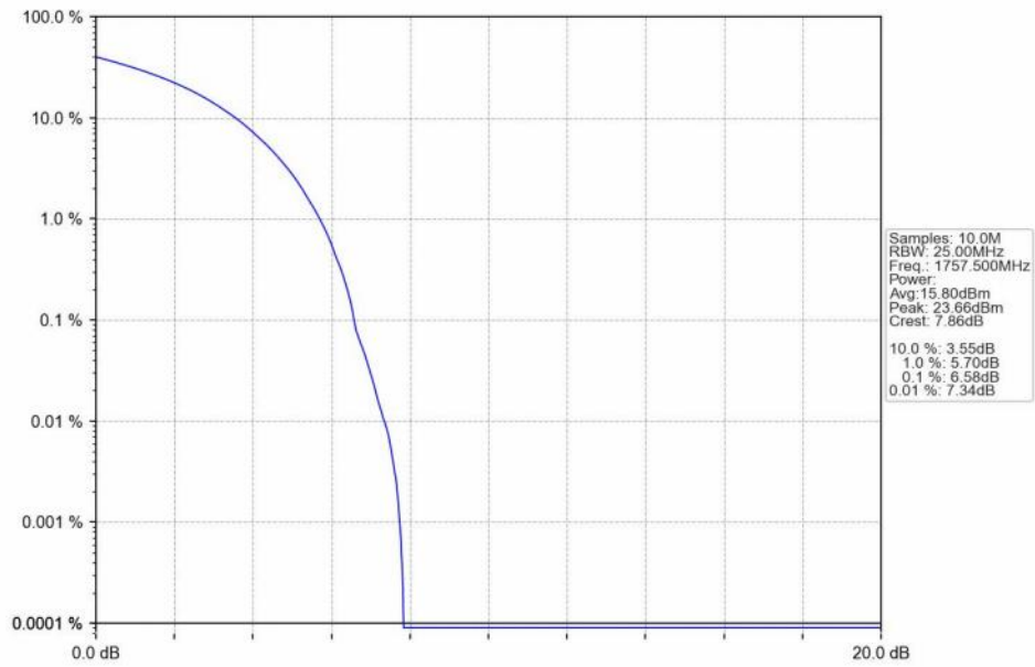
n66_15kHz_SISO_NTNV_45MHz_DFT-s-OFDM QPSK_1757.5MHz_Outer_Full_Ant1
