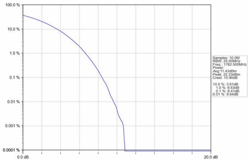
n66_15kHz_SISO_NTNV_35MHz_CP-OFDM 256 QAM_1762.5MHz_Outer_Full_Ant1
