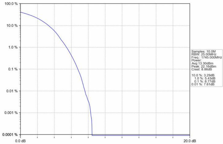
n66_15kHz_SISO_NTNV_35MHz_DFT-s-OFDM_256_QAM_1745MHz_Outer_Full_Ant1
