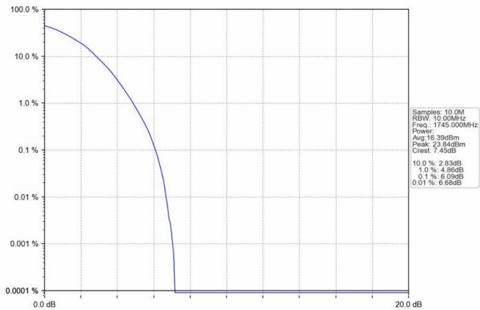
n66_30kHz_SISO_NTNV_10MHz_DFT-s-OFDM 64 QAM_1745MHz_Outer_Full_Ant1
