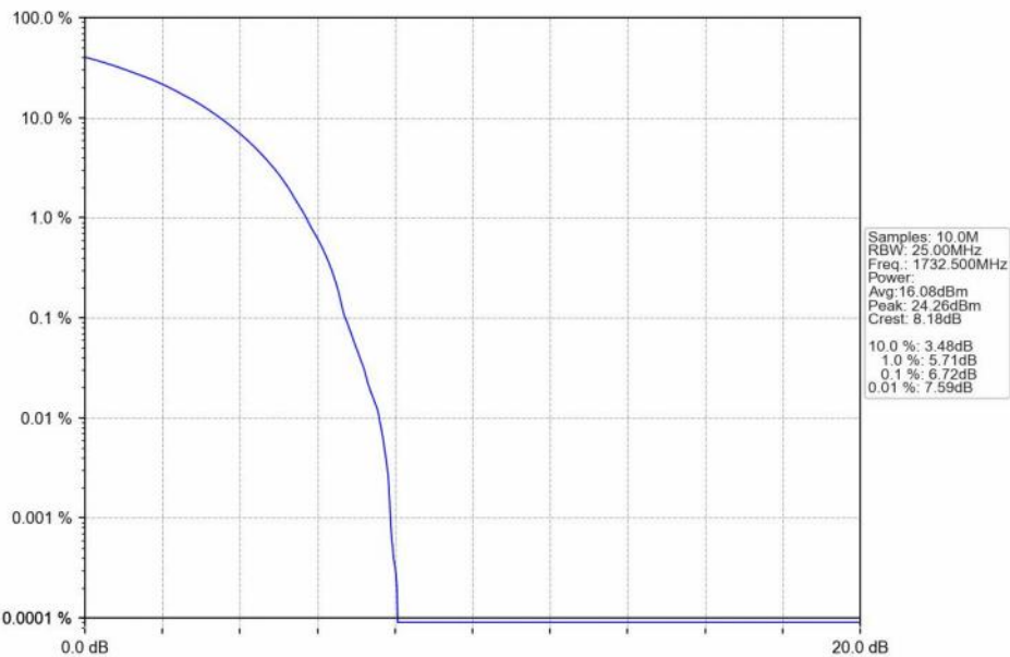
n66_15kHz_SISO_NTNV_45MHz_DFT-s-OFDM QPSK_1732.5MHz_Outer_Full_Ant1
