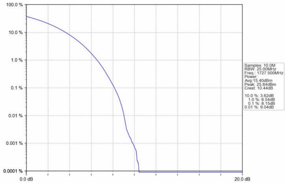
n66_15kHz_SISO_NTNV_35MHz_CP-OFDM QPSK_1727.5MHz_Outer_Full_Ant1
