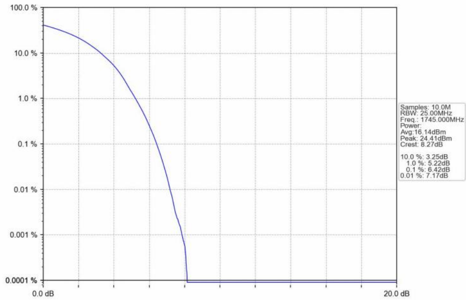
n66_15kHz_SISO_NTNV_35MHz_DFT-s-OFDM_16_QAM_1745MHz_Outer_Full_Ant1
