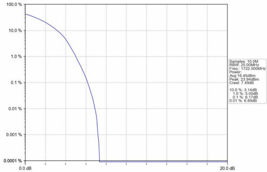
n66_15kHz_SISO_NTNV_25MHz_DFT-s-OFDM 64 QAM_1722.5MHz_Outer_Full_Ant1
