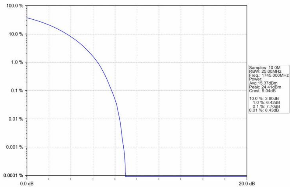
n66_30kHz_SISO_NTNV_15MHz_CP-OFDM 64 QAM_1745MHz_Outer_Full_Ant1
