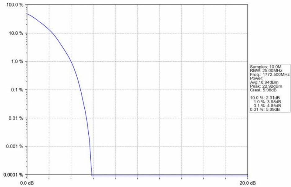
n66_30kHz_SISO_NTNV_15MHz_DFT-s-OFDM QPSK_1772.5MHz_Outer_Full_Ant1
