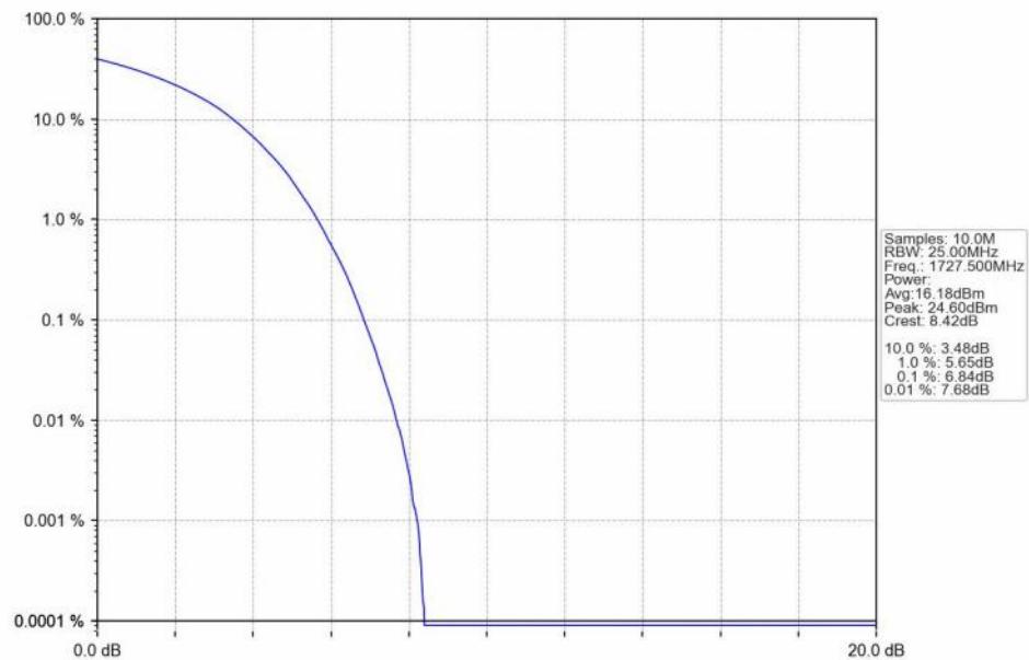
n66_15kHz_SISO_NTNV_35MHz_DFT-s-OFDM 64 QAM_1727.5MHz_Outer_Full_Ant1
