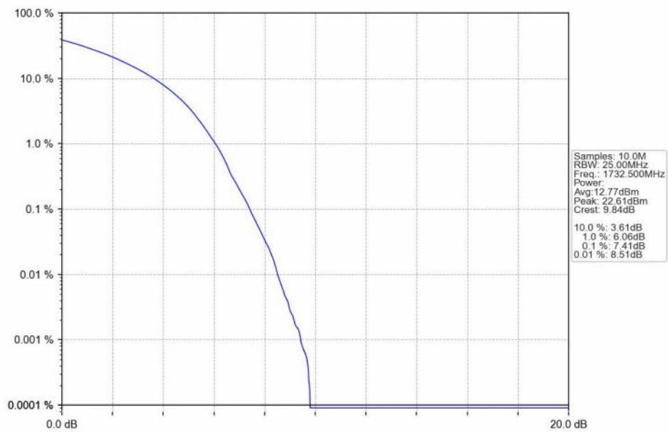
n66_15kHz_SISO_NTNV_45MHz_DFT-s-OFDM 256 QAM_1732.5MHz_Outer_Full_Ant1
