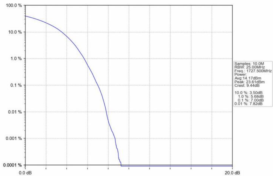
n66_15kHz_SISO_NTNV_35MHz_DFT-s-OFDM 256 QAM_1727.5MHz_Outer_Full_Ant1
