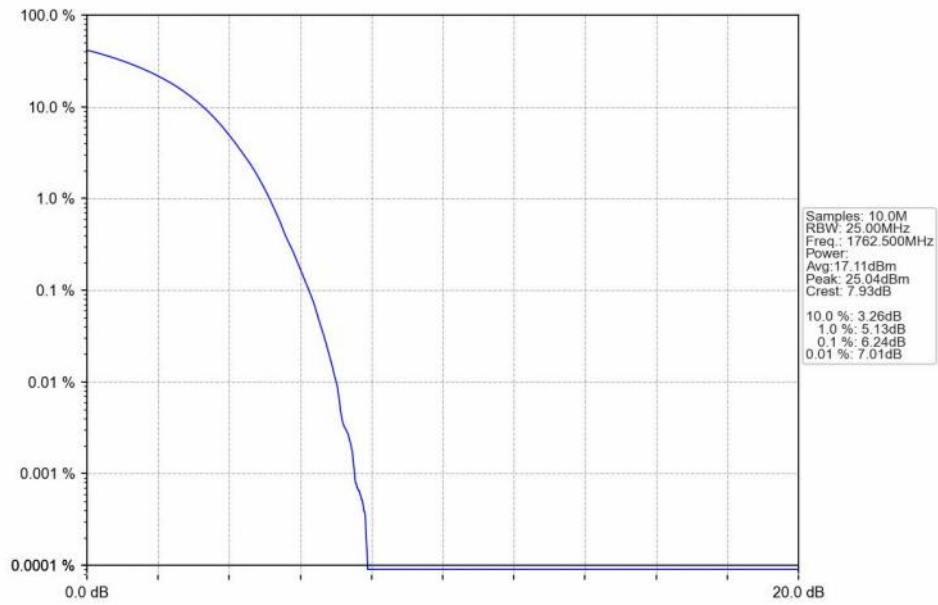
n66_15kHz_SISO_NTNV_35MHz_DFT-s-OFDM QPSK_1762.5MHz_Outer_Full_Ant1
