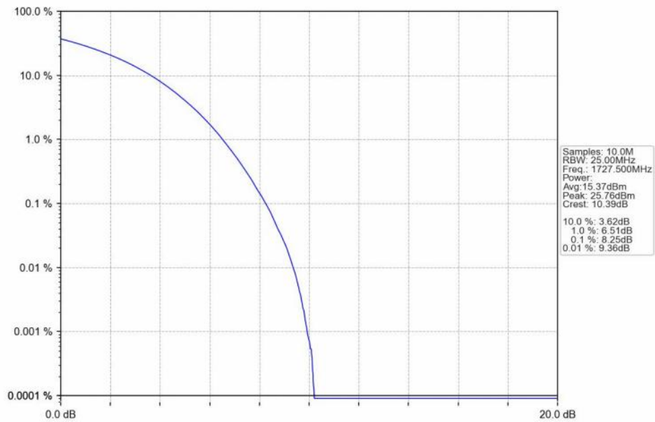
n66_15kHz_SISO_NTNV_35MHz_CP-OFDM 16 QAM_1727.5MHz_Outer_Full_Ant1
