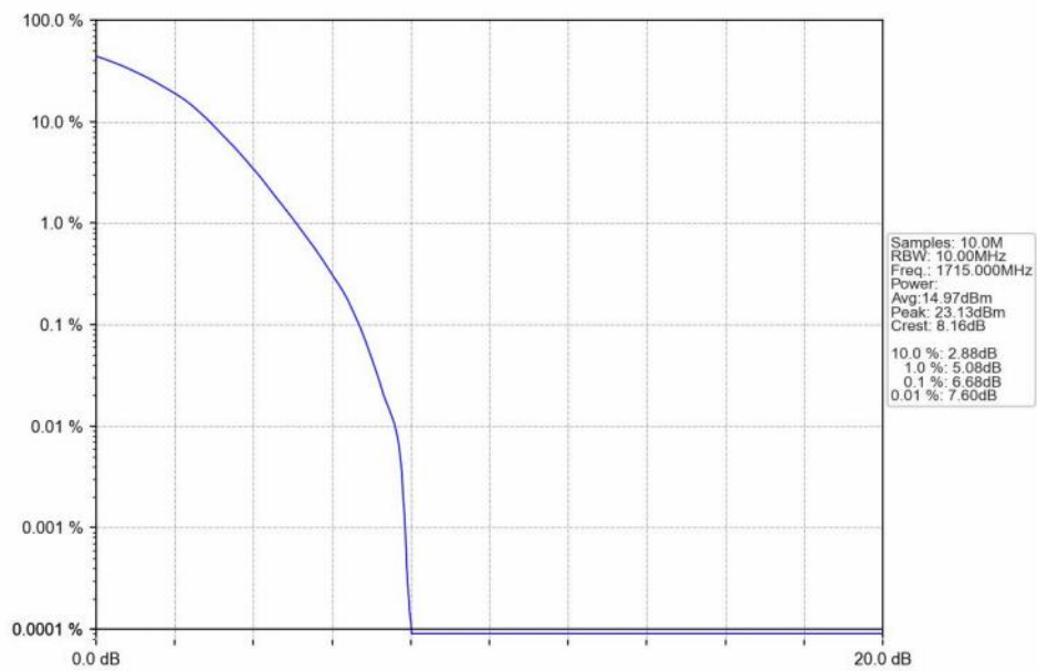
n66_30kHz_SISO_NTNV_10MHz_DFT-s-OFDM 256 QAM_1715MHz_Outer_Full_Ant1
