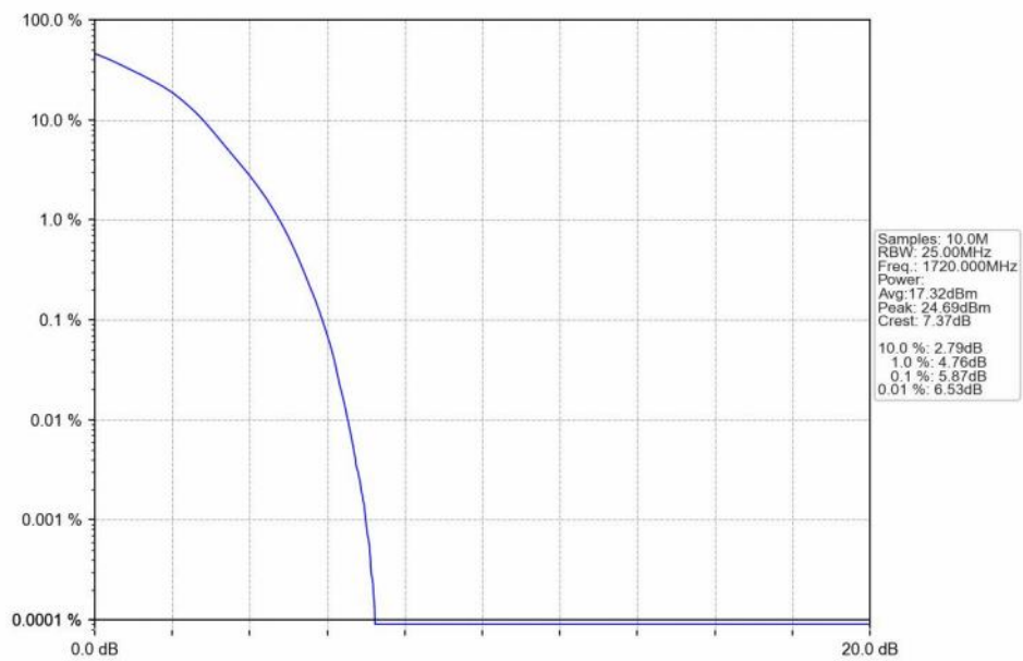
n66_30kHz_SISO_NTNV_20MHz_DFT-s-OFDM 16 QAM_1720MHz_Outer_Full_Ant1
