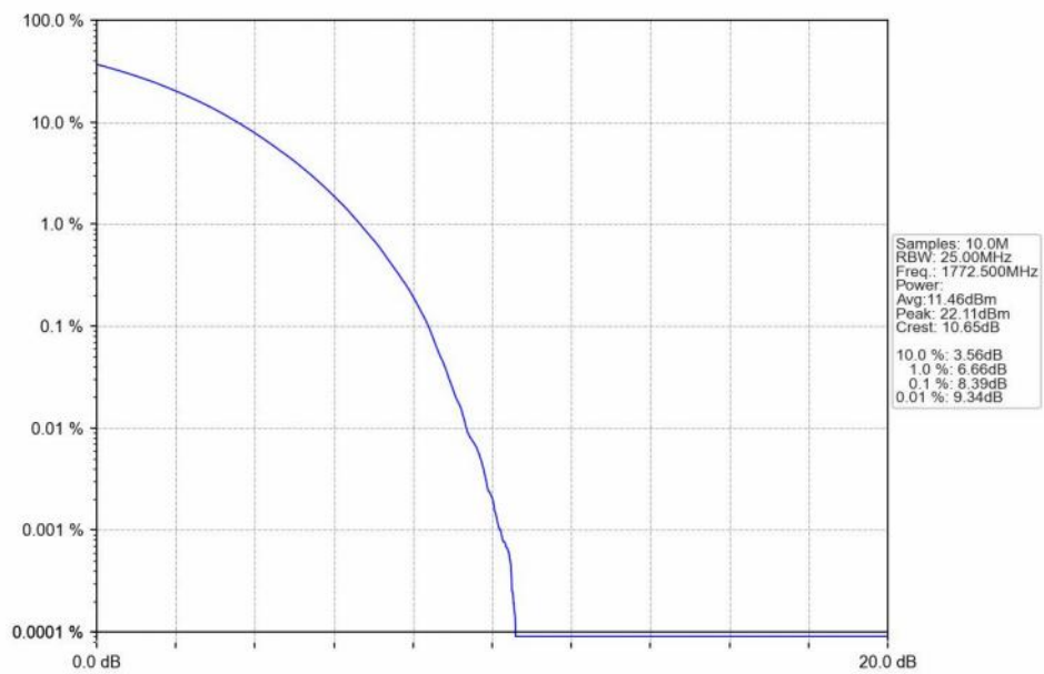
n66_30kHz_SISO_NTNV_15MHz_CP-OFDM 256 QAM_1772.5MHz_Outer_Full_Ant1
