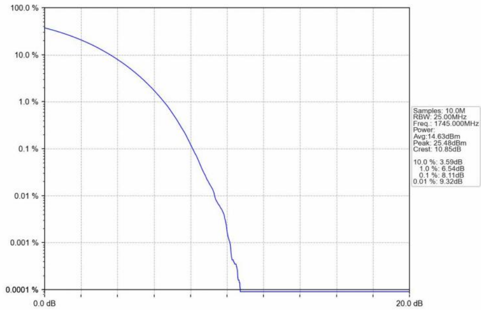
n66_15kHz_SISO_NTNV_40MHz_CP-OFDM_16 QAM_1745MHz_Outer_Full_Ant1
