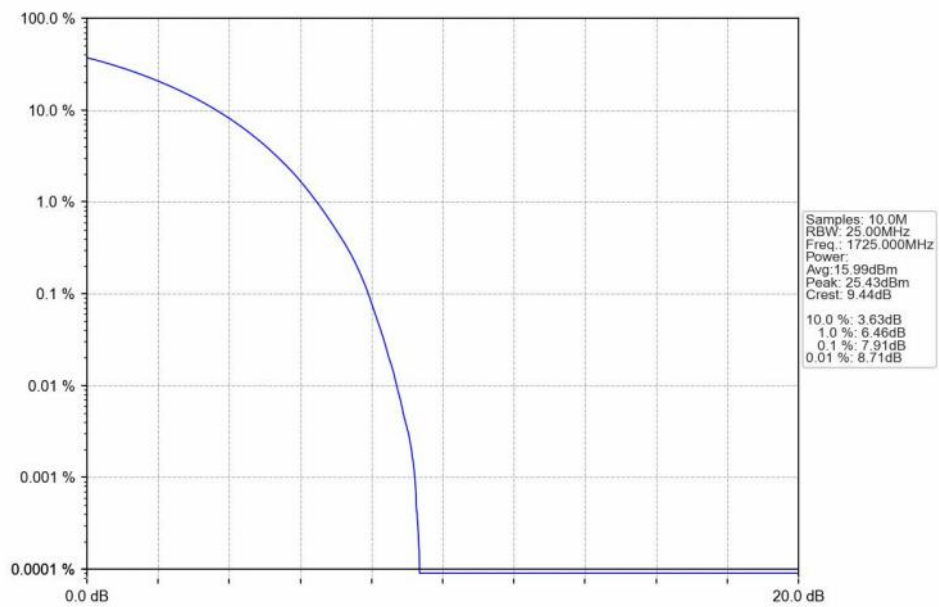
n66_15kHz_SISO_NTNV_30MHz_CP-OFDM 16 QAM_1725MHz_Outer_Full_Ant1
