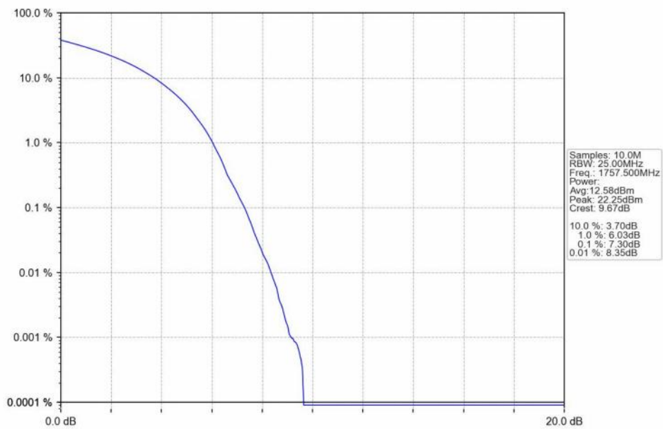
n66_15kHz_SISO_NTNV_45MHz_DFT-s-OFDM_256_QAM_1757.5MHz_Outer_Full_Ant1
