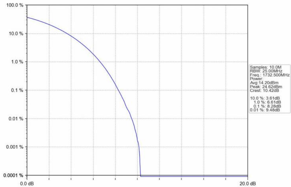
n66_15kHz_SISO_NTNV_45MHz_CP-OFDM 16 QAM_1732.5MHz_Outer_Full_Ant1
