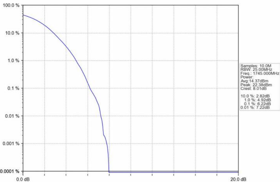
n66_30kHz_SISO_NTNV_15MHz_DFT-s-OFDM_256_QAM_1745MHz_Outer_Full_Ant1
