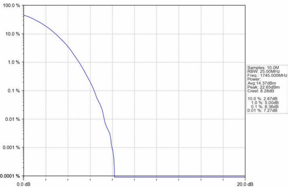
n66_30kHz_SISO_NTNV_20MHz_DFT-s-OFDM_256_QAM_1745MHz_Outer_Full_Ant1
