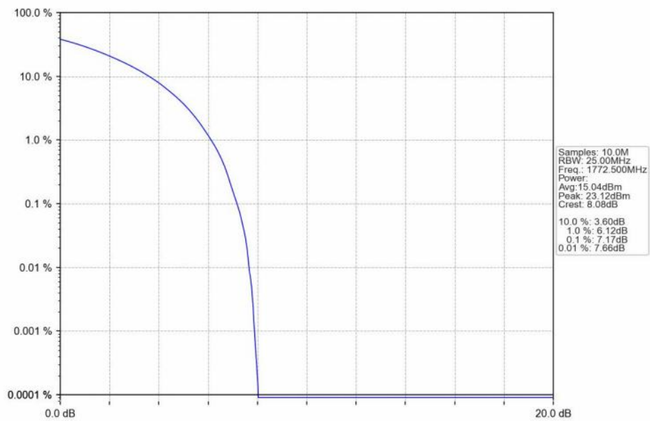
n66_30kHz_SISO_NTNV_15MHz_CP-OFDM_16_QAM_1772.5MHz_Outer_Full_Ant1
