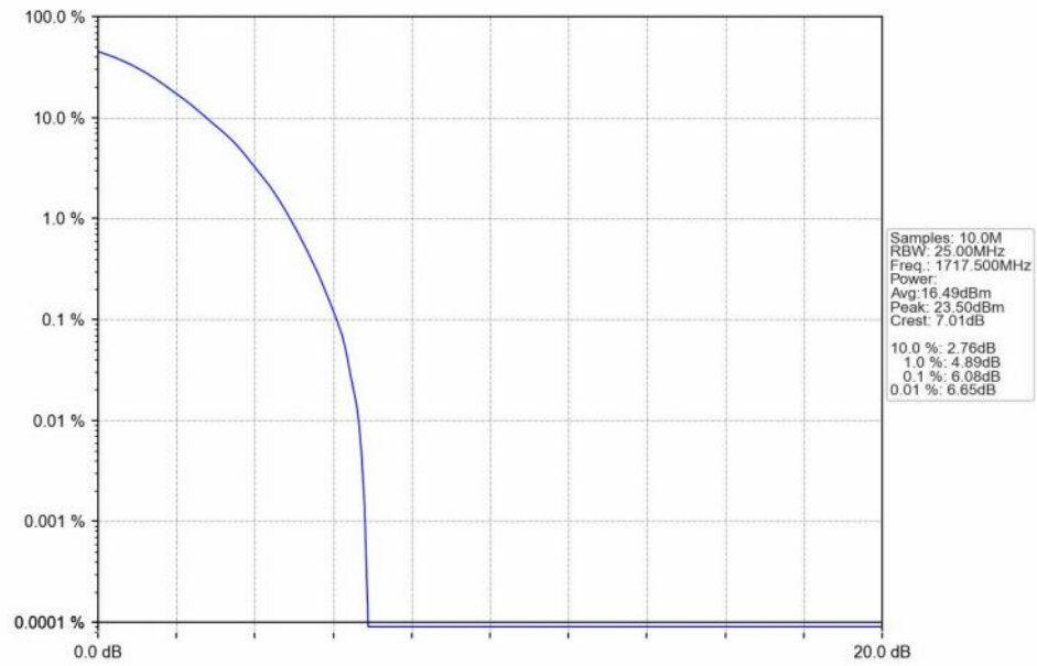
n66_15kHz_SISO_NTNV_15MHz_DFT-s-OFDM 64 QAM_1717.5MHz_Outer_Full_Ant1
