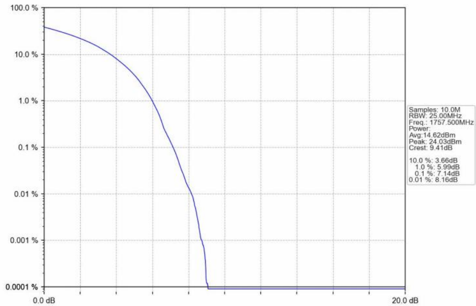
n66_15kHz_SISO_NTNV_45MHz_DFT-s-OFDM 64 QAM_1757.5MHz_Outer_Full_Ant1
