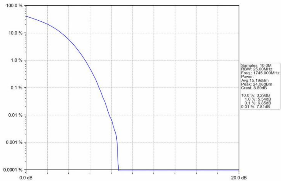
n66_15kHz_SISO_NTNV_40MHz_DFT-s-OFDM_64_QAM_1745MHz_Outer_Full_Ant1
