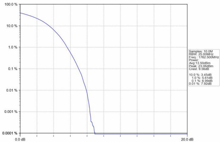
n66_15kHz_SISO_NTNV_35MHz_DFT-s-OFDM_256_QAM_1762.5MHz_Outer_Full_Ant1
