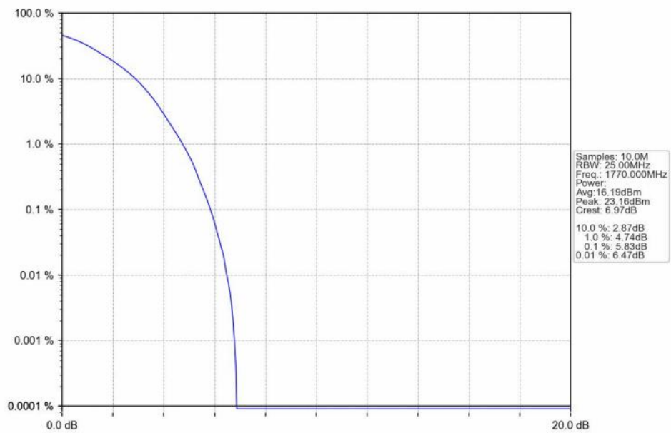
n66_30kHz_SISO_NTNV_20MHz_DFT-s-OFDM_16_QAM_1770MHz_Outer_Full_Ant1
