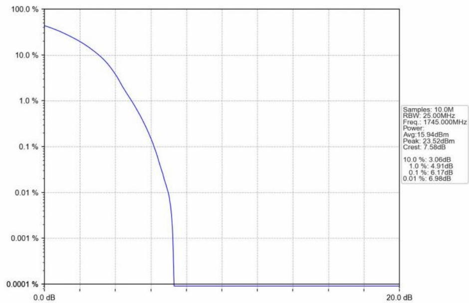
n66_15kHz_SISO_NTNV_25MHz_DFT-s-OFDM 64 QAM_1745MHz_Outer_Full_Ant1
