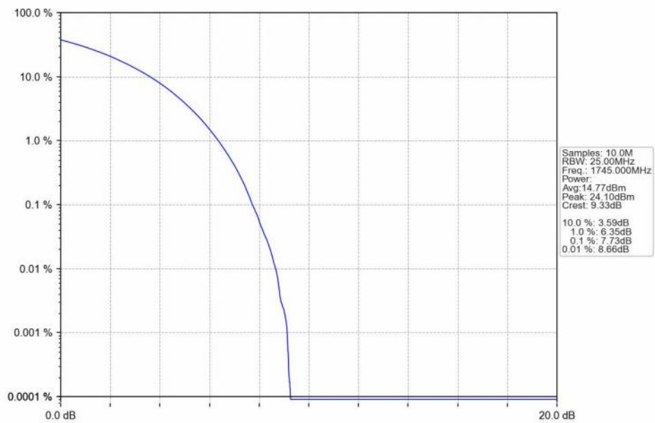
n66_15kHz_SISO_NTNV_20MHz_CP-OFDM 64 QAM_1745MHz_Outer_Full_Ant1
