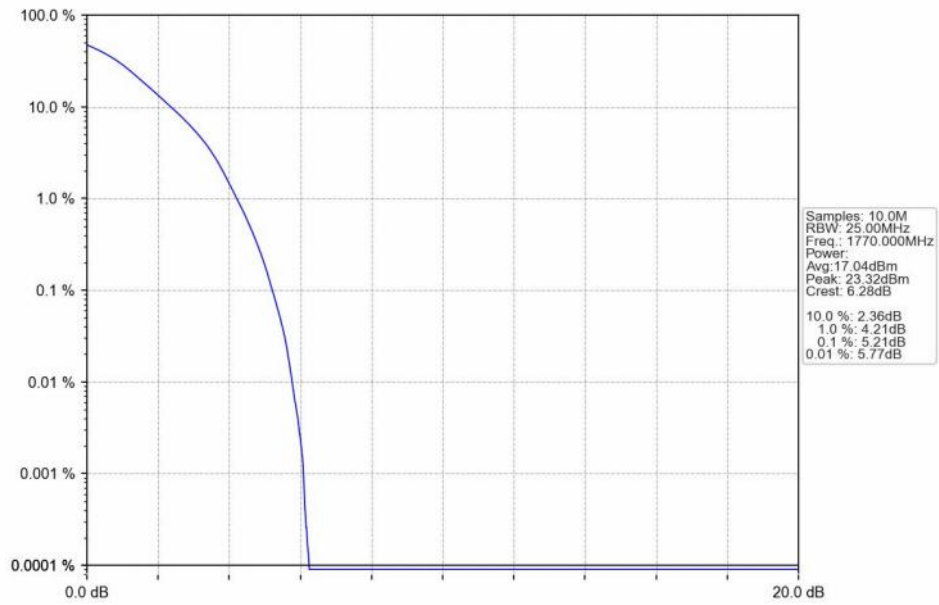
n66_30kHz_SISO_NTNV_20MHz_DFT-s-OFDM QPSK_1770MHz_Outer_Full_Ant1
