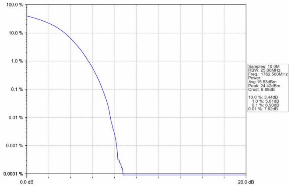
n66_15kHz_SISO_NTNV_35MHz_DFT-s-OFDM 64 QAM_1762.5MHz_Outer_Full_Ant1
