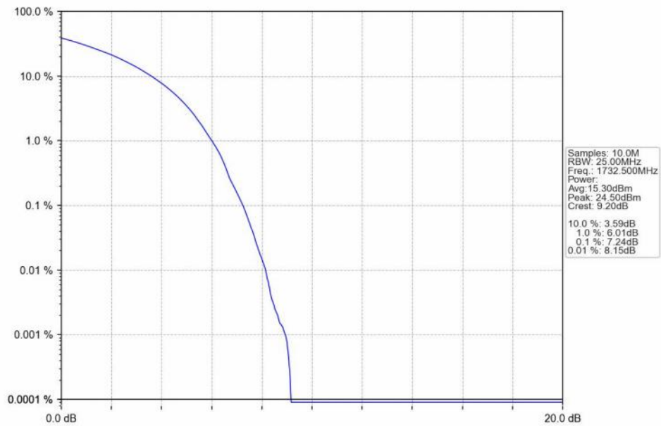
n66_15kHz_SISO_NTNV_45MHz_DFT-s-OFDM 16 QAM_1732.5MHz_Outer_Full_Ant1
