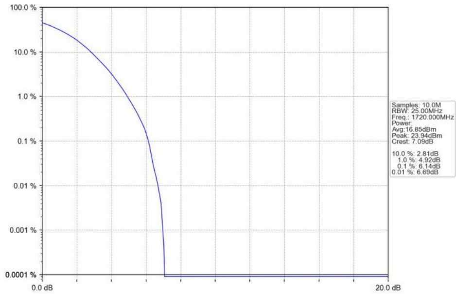
n66_30kHz_SISO_NTNV_20MHz_DFT-s-OFDM_64_QAM_1720MHz_Outer_Full_Ant1
