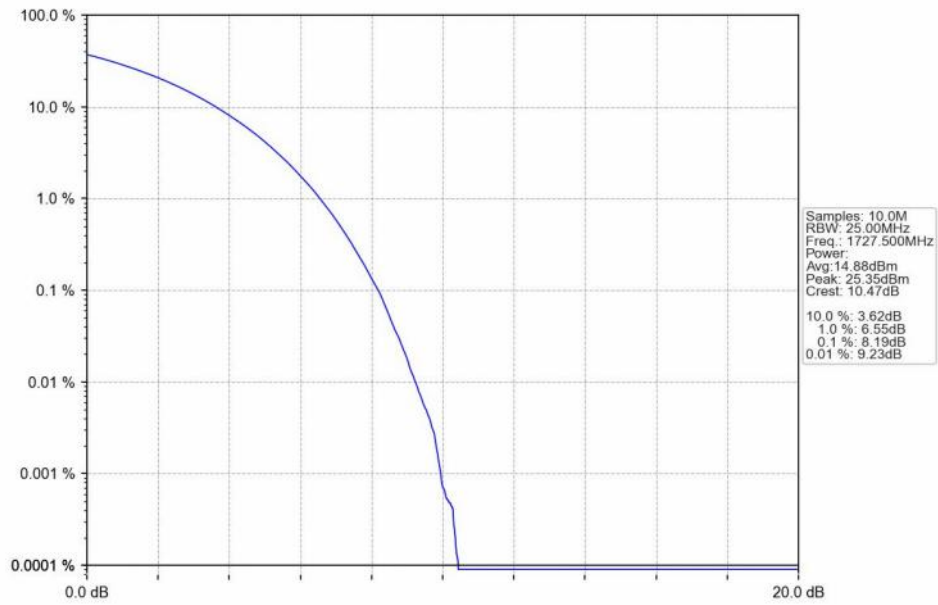
n66_15kHz_SISO_NTNV_35MHz_CP-OFDM 64 QAM_1727.5MHz_Outer_Full_Ant1
