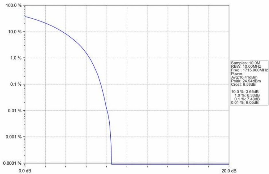
n66_30kHz_SISO_NTNV_10MHz_CP-OFDM 16 QAM_1715MHz_Outer_Full_Ant1
