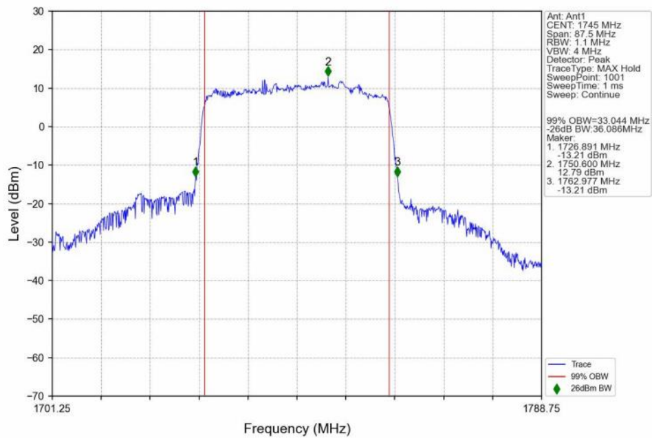
n66_30kHz_SISO_NTNV_35MHz_CP-OFDM 64 QAM_1745MHz_Outer_Full_Ant1
