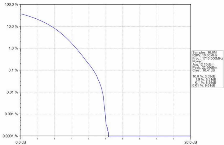
n66_15kHz_SISO_NTNV_10MHz_CP-OFDM 256 QAM_1715MHz_Outer_Full_Ant1
