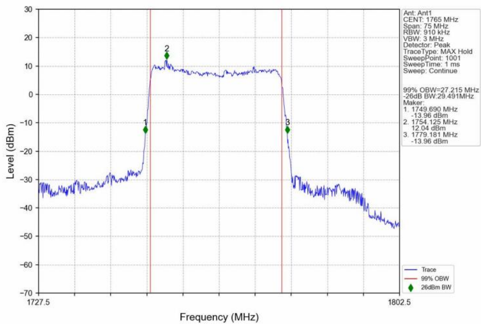
n66_30kHz_SISO_NTNV_30MHz_DFT-s-OFDM_256_QAM_1765MHz_Outer_Full_Ant1
