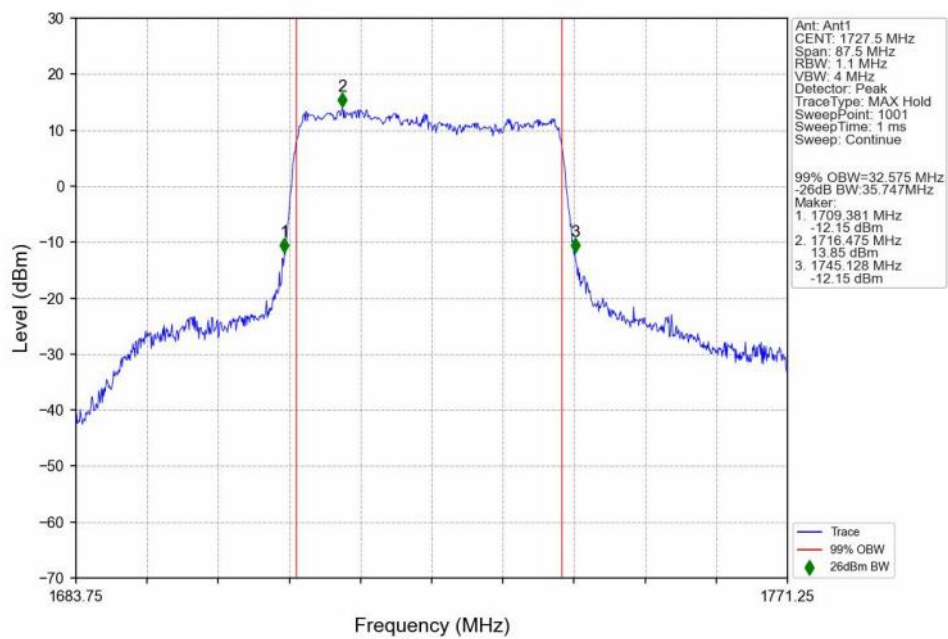
n66_30kHz_SISO_NTNV_35MHz_DFT-s-OFDM 16 QAM_1727.5MHz_Outer_Full_Ant1
