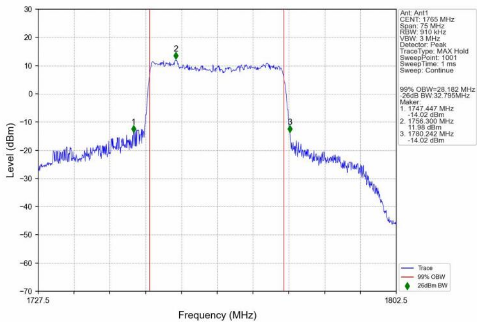
n66_30kHz_SISO_NTNV_30MHz_CP-OFDM_16 QAM_1765MHz_Outer_Full_Ant1
