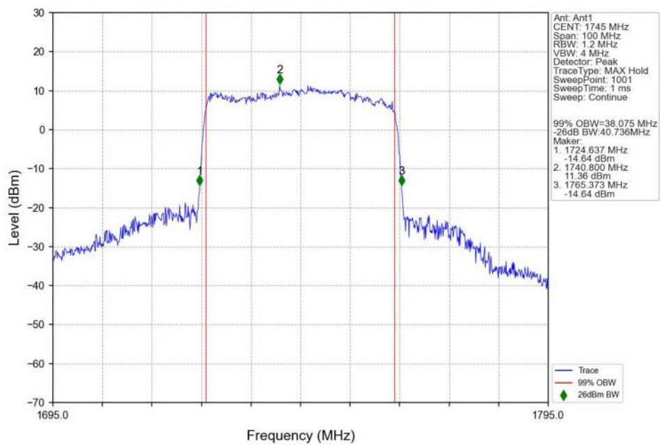
n66_30kHz_SISO_NTNV_40MHz_CP-OFDM 64 QAM_1745MHz_Outer_Full_Ant1
