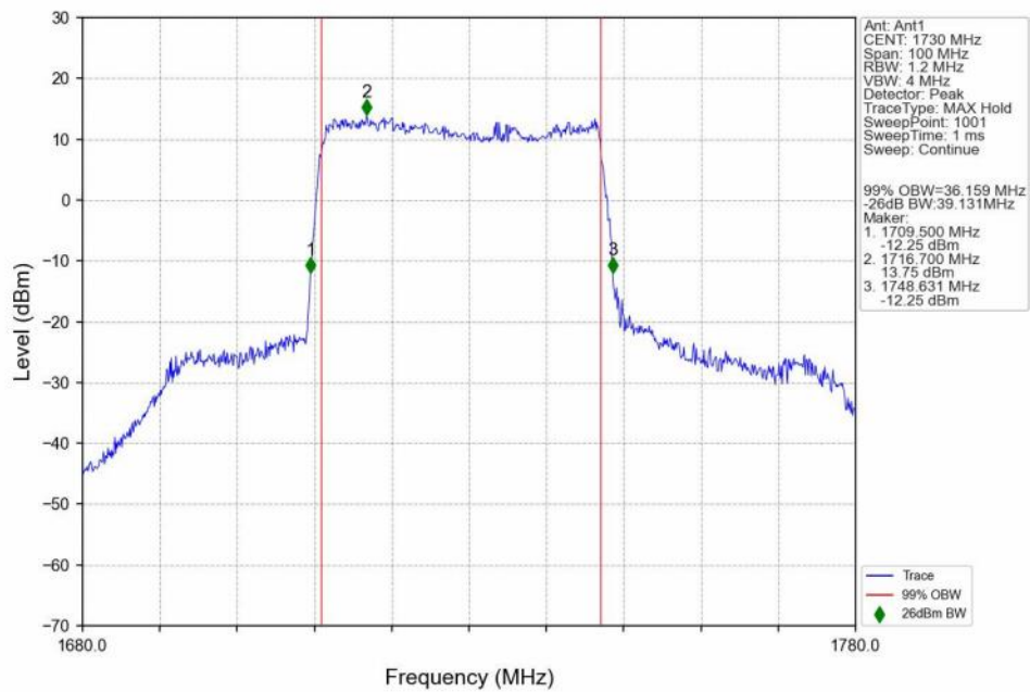
n66_30kHz_SISO_NTNV_40MHz_DFT-s-OFDM 16 QAM 1730MHz_Outer_Full_Ant1
