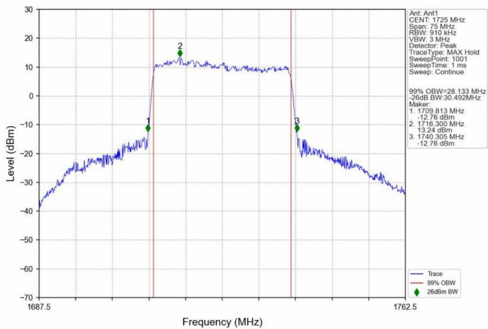
n66_30kHz_SISO_NTNV_30MHz_CP-OFDM 16 QAM_1725MHz_Outer_Full_Ant1
