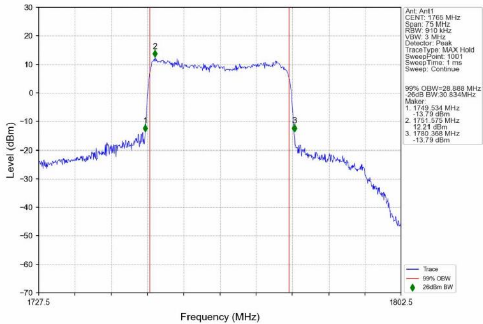
n66_15kHz_SISO_NTNV_30MHz_CP-OFDM_16 QAM_1765MHz_Outer_Full_Ant1
