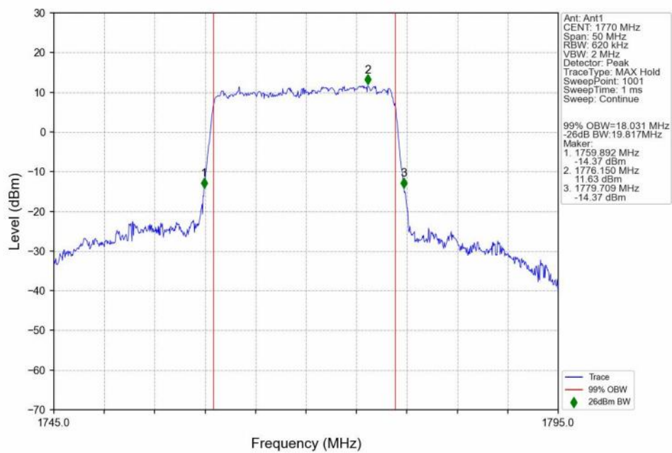
n66_30kHz_SISO_NTNV_20MHz_DFT-s-OFDM_16_QAM_1770MHz_Outer_Full_Ant1
