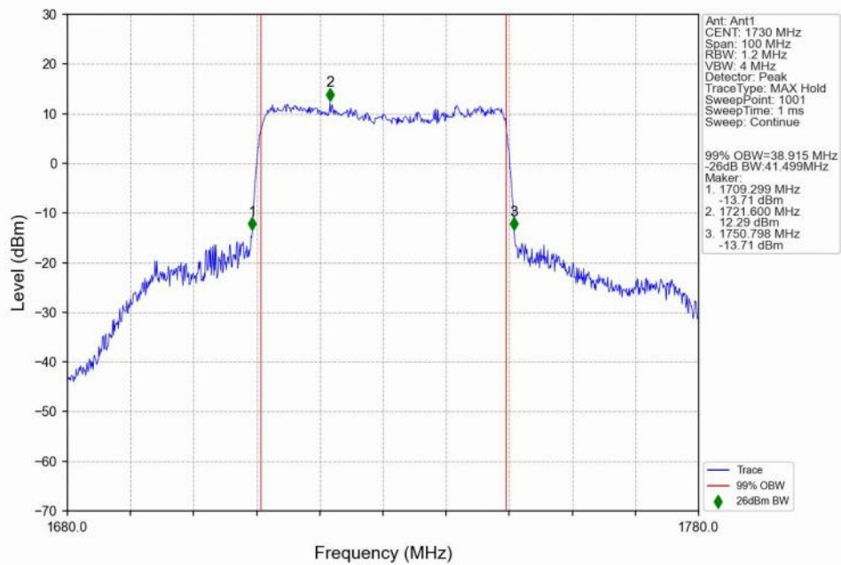
n66_15kHz_SISO_NTNV_40MHz_CP-OFDM 16 QAM_1730MHz_Outer_Full_Ant1
