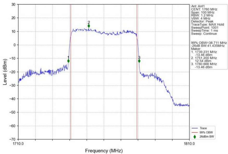
n66_15kHz_SISO_NTNV_40MHz_CP-OFDM_16 QAM_1760MHz_Outer_Full_Ant1
