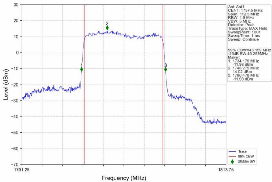
n66_15kHz_SISO_NTNV_45MHz_DFT-s-OFDM_16_QAM_1757.5MHz_Outer_Full_Ant1
