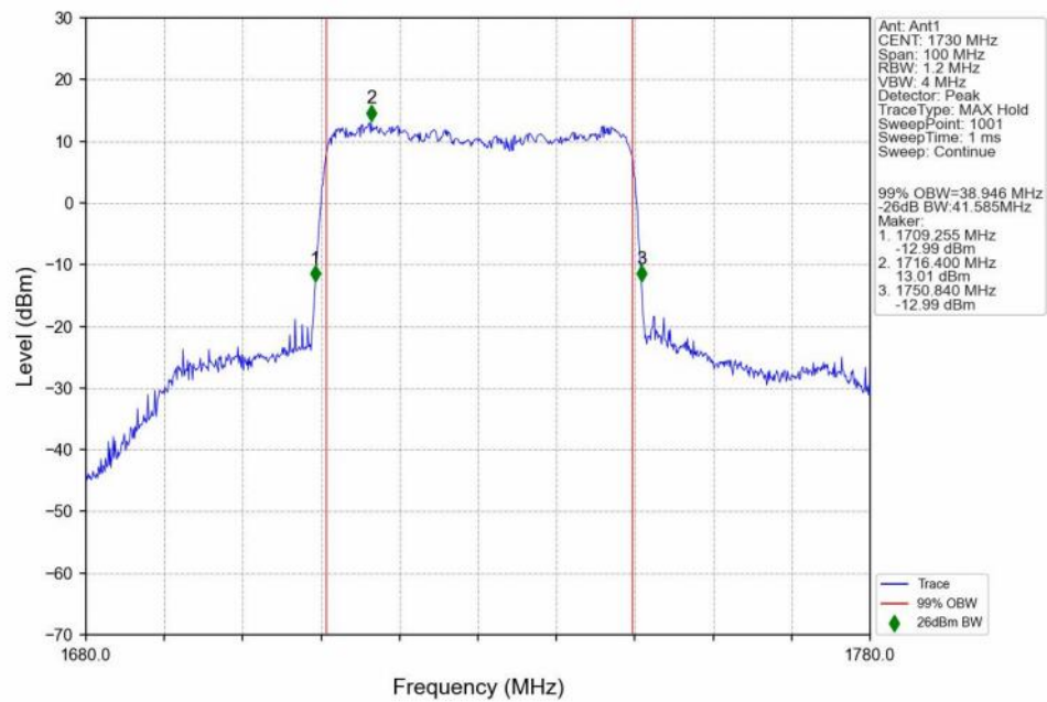
n66_15kHz_SISO_NTNV_40MHz_DFT-s-OFDM 16 QAM 1730MHz_Outer_Full_Ant1
