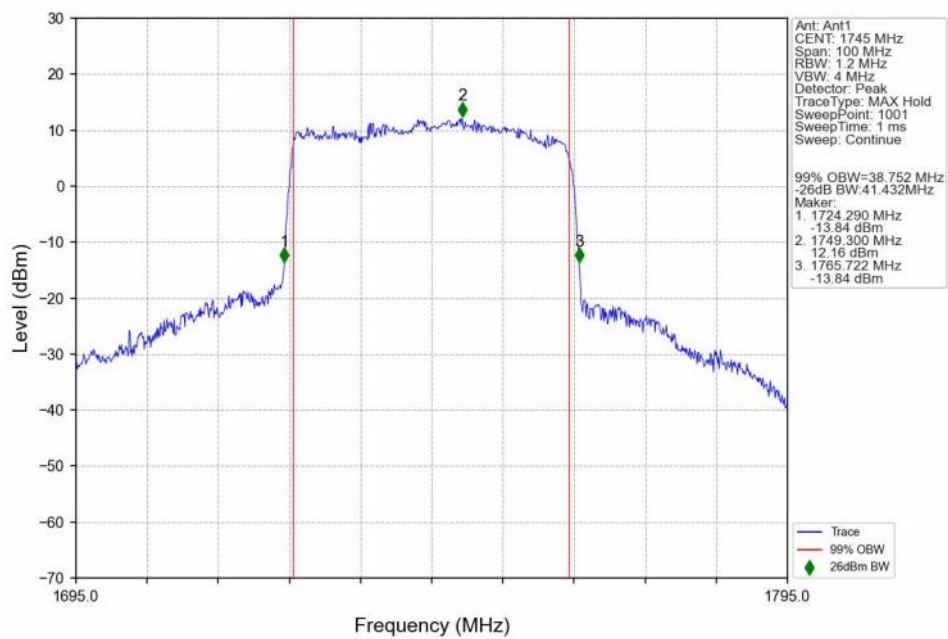
n66_15kHz_SISO_NTNV_40MHz_CP-OFDM QPSK_1745MHz_Outer_Full_Ant1
