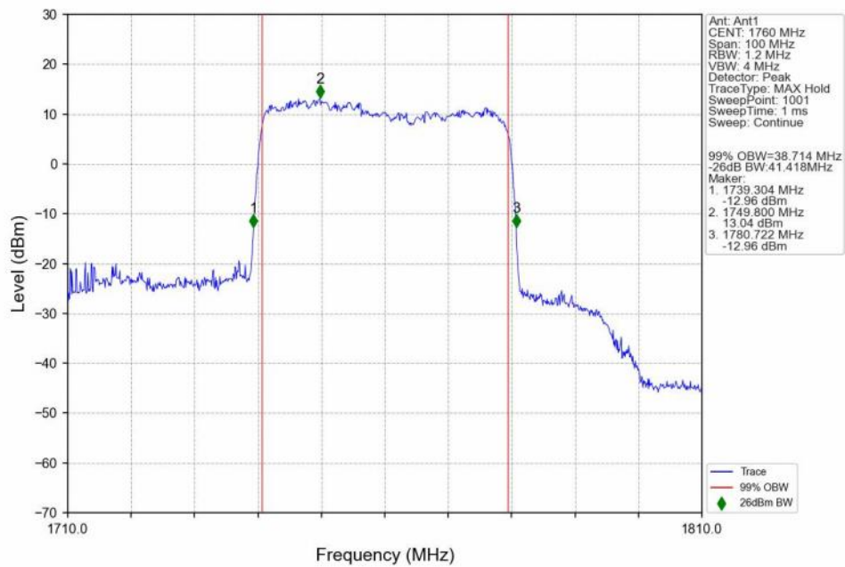
n66_15kHz_SISO_NTNV_40MHz_DFT-s-OFDM_16_QAM_1760MHz_Outer_Full_Ant1
