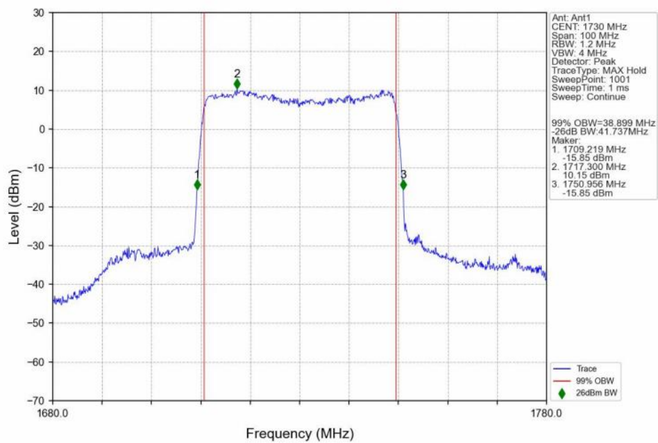
n66_15kHz_SISO_NTNV_40MHz_DFT-s-OFDM 256 QAM_1730MHz_Outer_Full_Ant1
