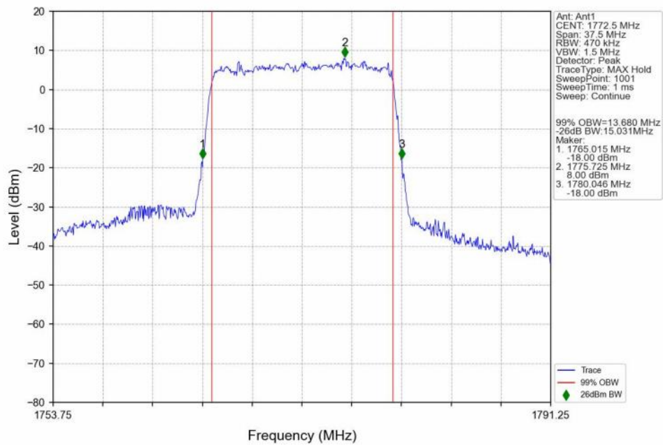
n66_30kHz_SISO_NTNV_15MHz_CP-OFDM 256 QAM 1772.5MHz_Outer_Full_Ant1
