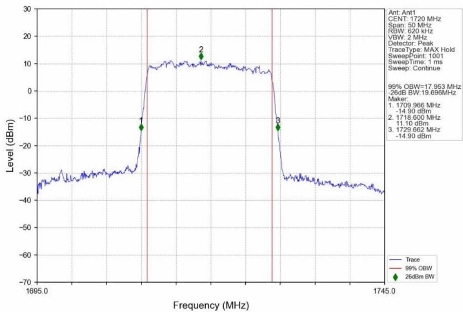
n66_30kHz_SISO_NTNV_20MHz_DFT-s-OFDM 256 QAM_1720MHz_Outer_Full_Ant1
