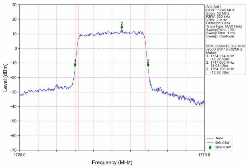
n66_30kHz_SISO_NTNV_20MHz_DFT-s-OFDM_64_QAM_1745MHz_Outer_Full_Ant1
