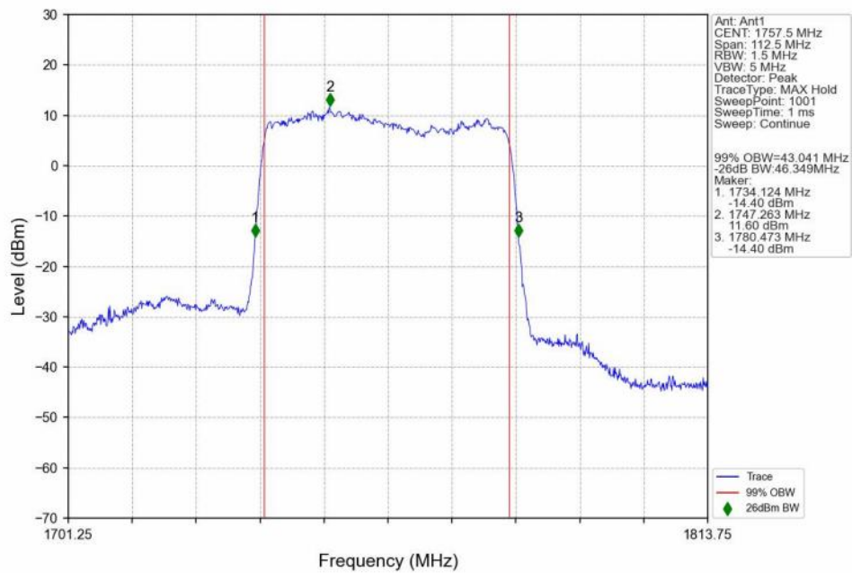
n66_15kHz_SISO_NTNV_45MHz_DFT-s-OFDM_256_QAM_1757.5MHz_Outer_Full_Ant1
