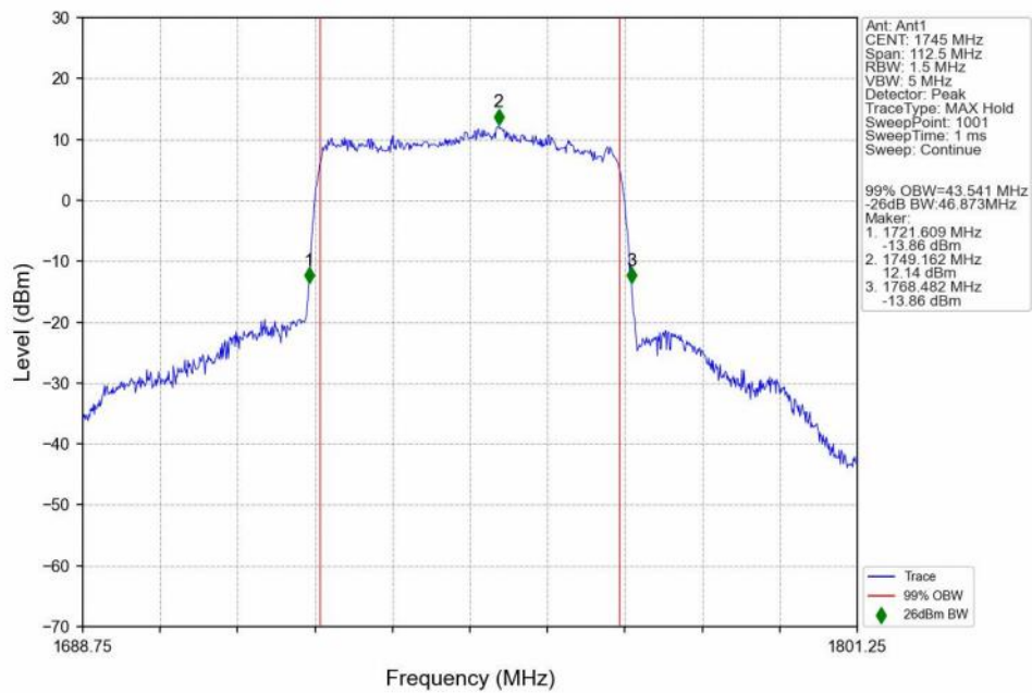
n66_15kHz_SISO_NTNV_45MHz_CP-OFDM 64 QAM 1745MHz_Outer_Full_Ant1
