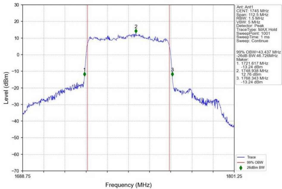
n66_15kHz_SISO_NTNV_45MHz_CP-OFDM_QPSK_1745MHz_Outer_Full_Ant1
