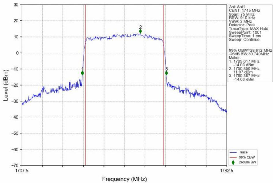
n66_15kHz_SISO_NTNV_30MHz_CP-OFDM QPSK_1745MHz_Outer_Full_Ant1
