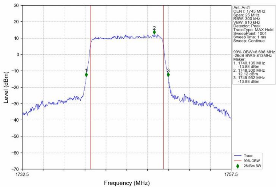
n66_30kHz_SISO_NTNV_10MHz_DFT-s-OFDM_64_QAM_1745MHz_Outer_Full_Ant1
