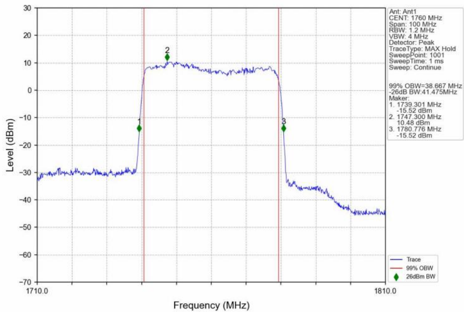
n66_15kHz_SISO_NTNV_40MHz_DFT-s-OFDM_256_QAM_1760MHz_Outer_Full_Ant1
