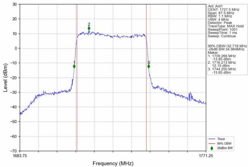
n66_15kHz_SISO_NTNV_35MHz_DFT-s-OFDM 256 QAM_1727.5MHz_Outer_Full_Ant1
