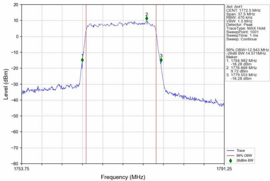
n66_30kHz_SISO_NTNV_15MHz_DFT-s-OFDM_256_QAM_1772.5MHz_Outer_Full_Ant1
