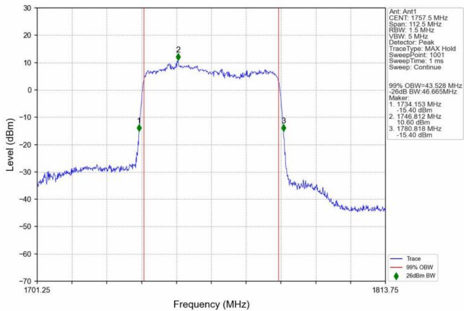
n66_15kHz_SISO_NTNV_45MHz_CP-OFDM_256_QAM_1757.5MHz_Outer_Full_Ant1
