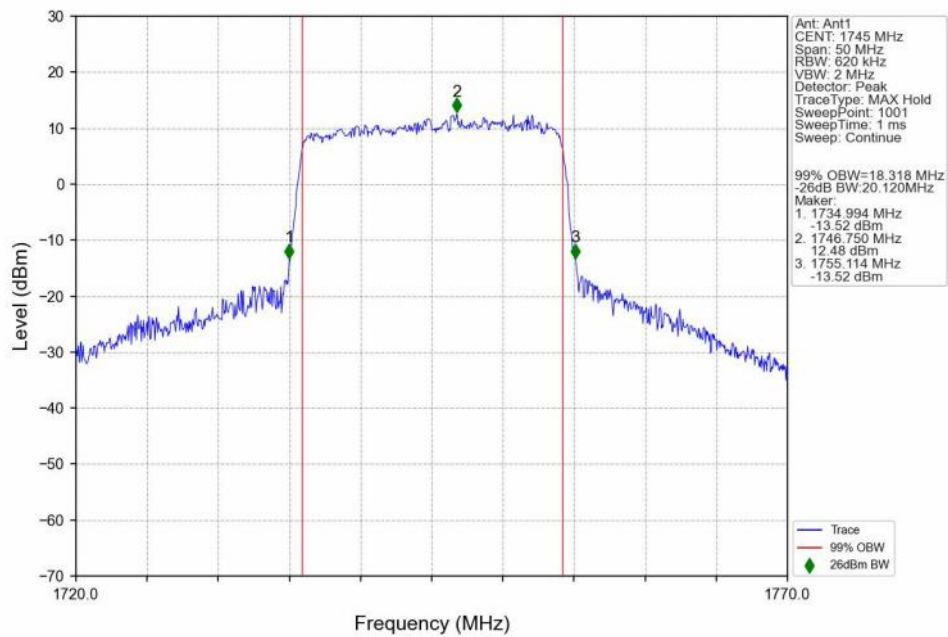
n66_30kHz_SISO_NTNV_20MHz_CP-OFDM QPSK_1745MHz_Outer_Full_Ant1
