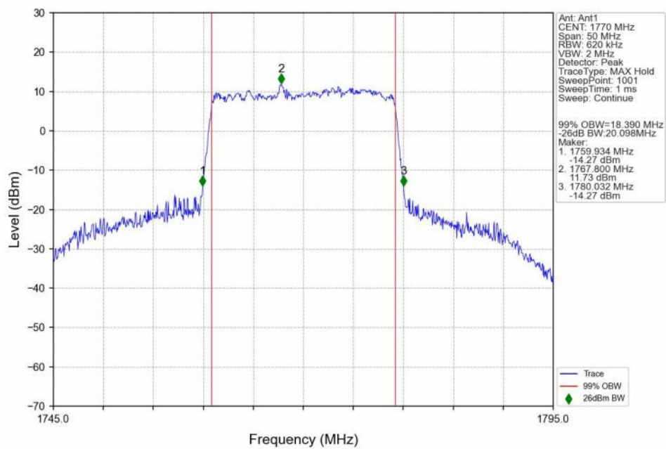
n66_30kHz_SISO_NTNV_20MHz_CP-OFDM_16 QAM_1770MHz_Outer_Full_Ant1
