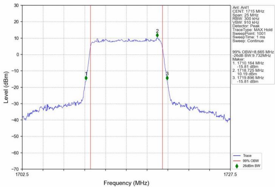
n66_30kHz_SISO_NTNV_10MHz_DFT-s-OFDM 256 QAM_1715MHz_Outer_Full_Ant1
