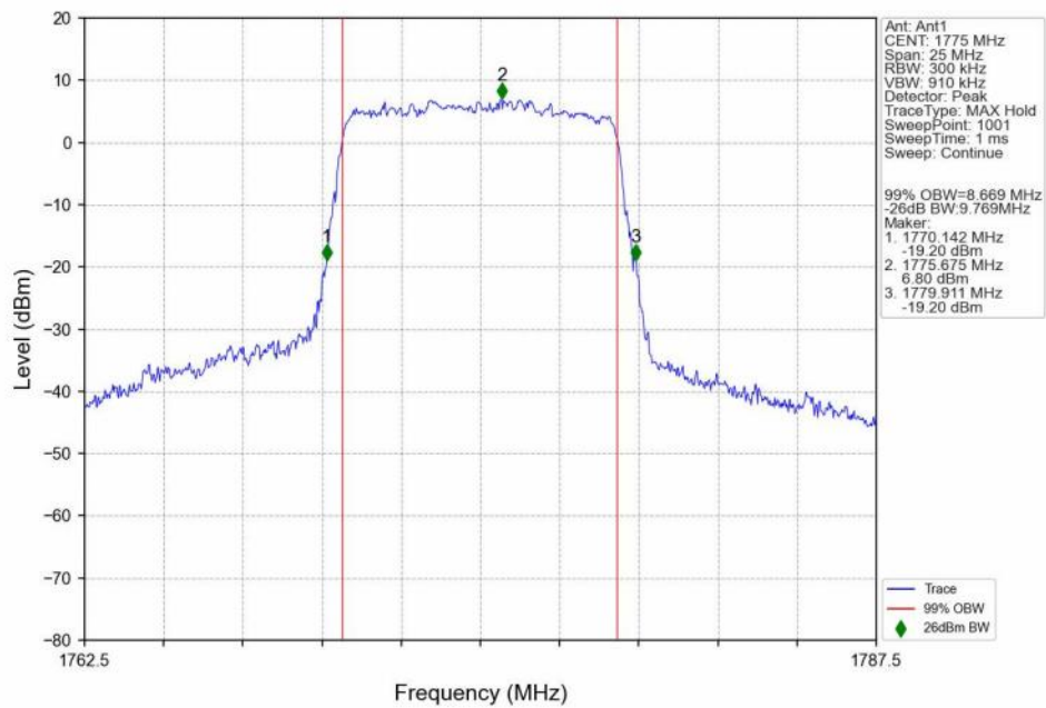
n66_30kHz_SISO_NTNV_10MHz_CP-OFDM_256_QAM_1775MHz_Outer_Full_Ant1
