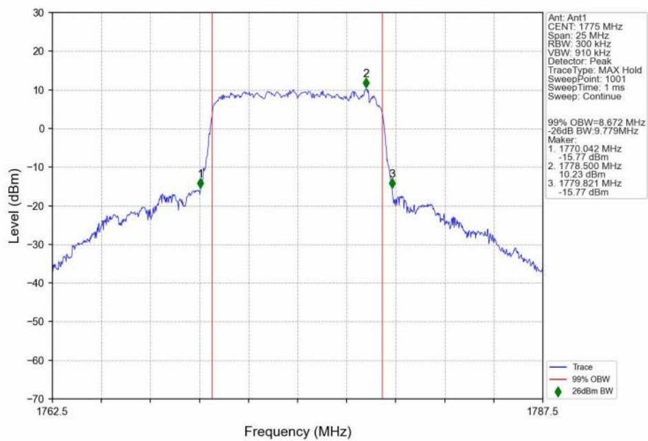
n66_30kHz_SISO_NTNV_10MHz_CP-OFDM_16 QAM_1775MHz_Outer_Full_Ant1
