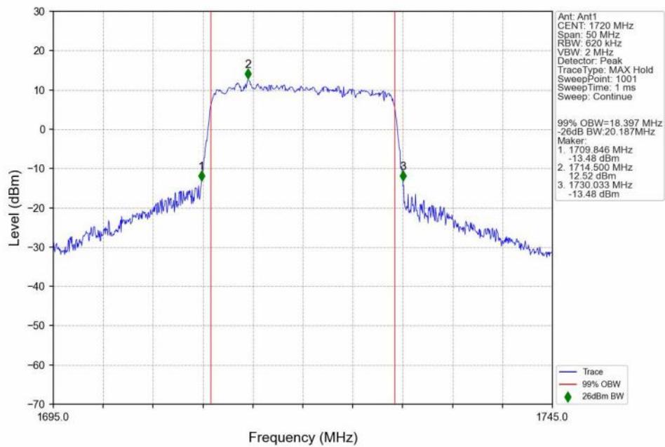
n66_30kHz_SISO_NTNV_20MHz_CP-OFDM 16 QAM 1720MHz_Outer_Full_Ant1
