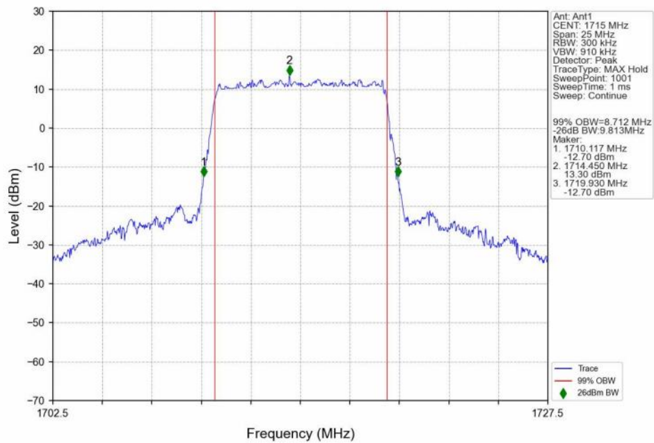
n66_30kHz_SISO_NTNV_10MHz_DFT-s-OFDM 16 QAM 1715MHz_Outer_Full_Ant1
