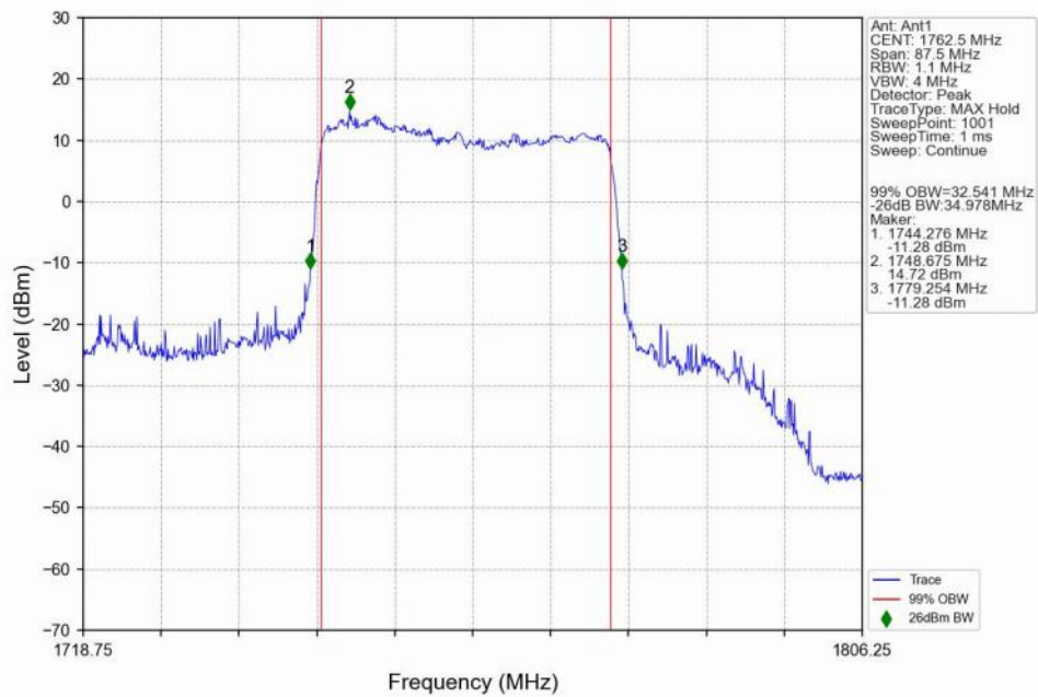
n66_15kHz_SISO_NTNV_35MHz_DFT-s-OFDM_16_QAM_1762.5MHz_Outer_Full_Ant1
