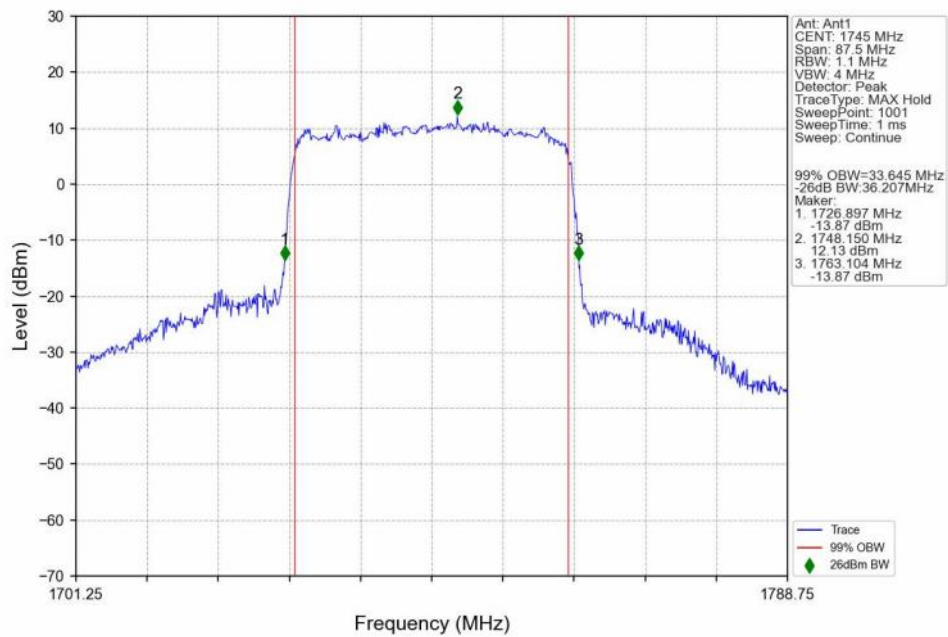
n66_15kHz_SISO_NTNV_35MHz_CP-OFDM 64 QAM 1745MHz_Outer_Full_Ant1
