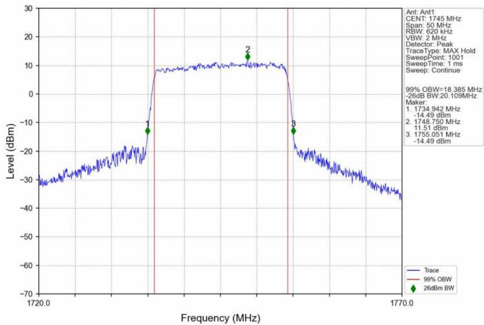
n66_30kHz_SISO_NTNV_20MHz_CP-OFDM 64 QAM_1745MHz_Outer_Full_Ant1
