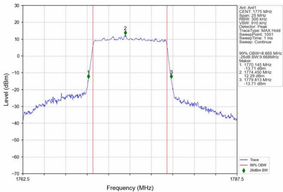
n66_30kHz_SISO_NTNV_10MHz_DFT-s-OFDM_16_QAM_1775MHz_Outer_Full_Ant1
