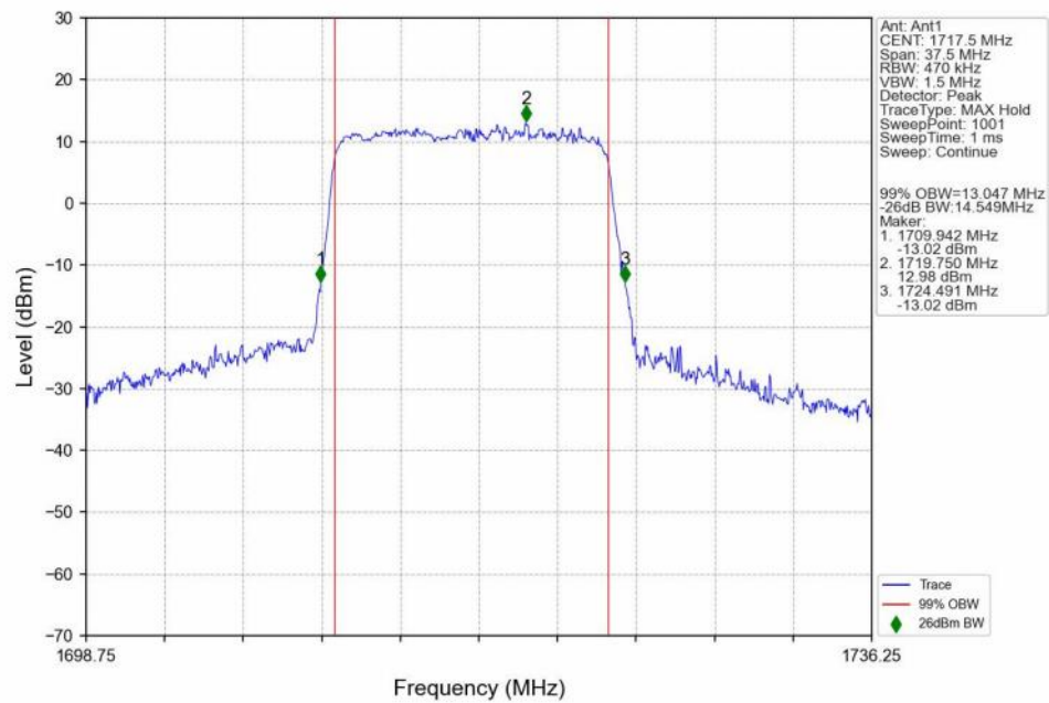
n66_30kHz_SISO_NTNV_15MHz_DFT-s-OFDM 16 QAM_1717.5MHz_Outer_Full_Ant1
