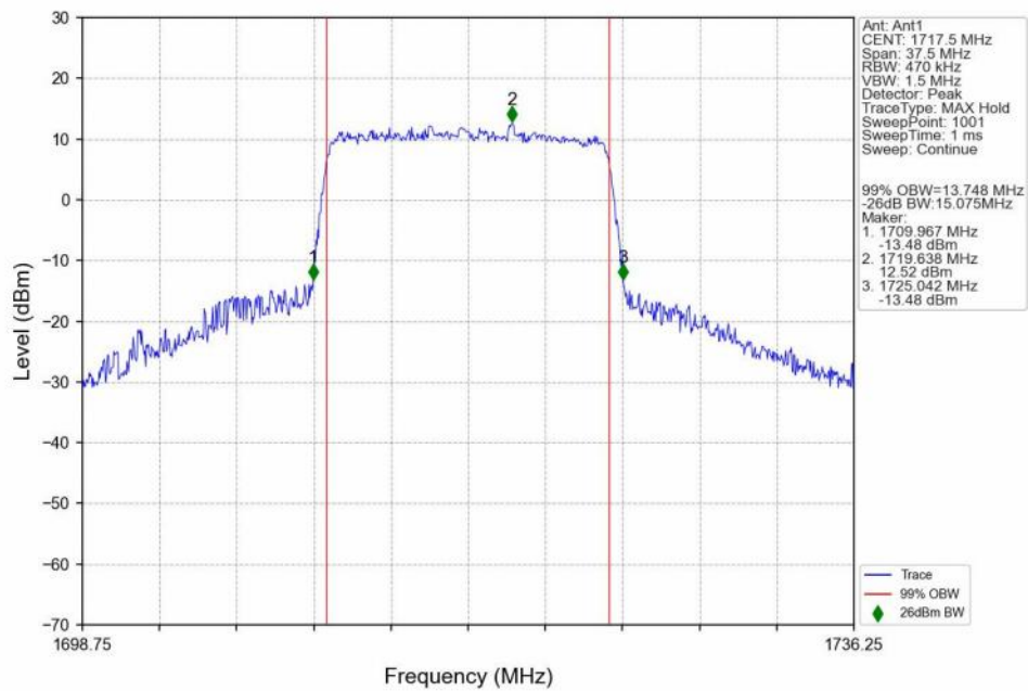
n66_30kHz_SISO_NTNV_15MHz_CP-OFDM 16 QAM_1717.5MHz_Outer_Full_Ant1
