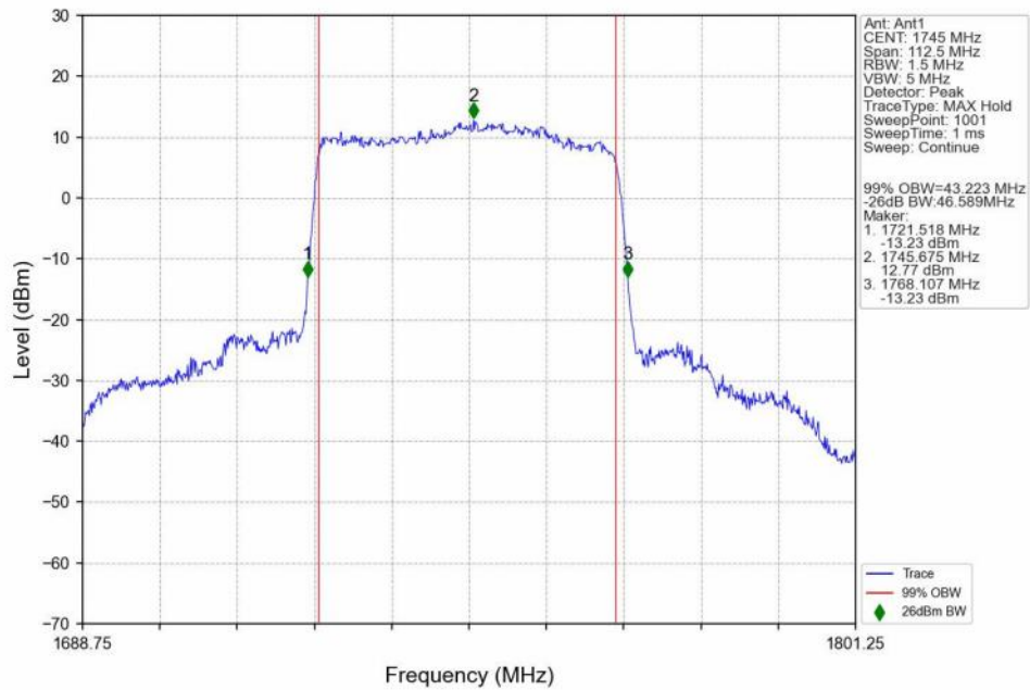
n66_15kHz_SISO_NTNV_45MHz_DFT-s-OFDM_64_QAM_1745MHz_Outer_Full_Ant1
