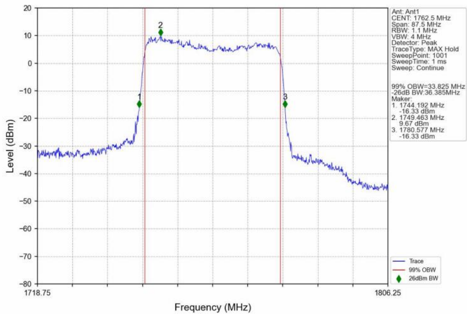
n66_15kHz_SISO_NTNV_35MHz_CP-OFDM 256 QAM 1762.5MHz_Outer_Full_Ant1
