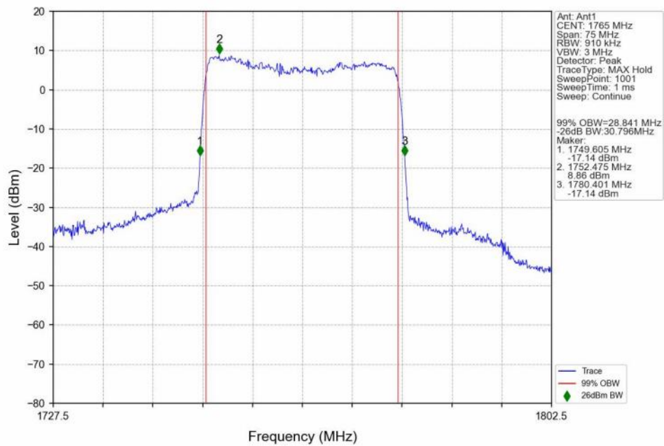
n66_15kHz_SISO_NTNV_30MHz_CP-OFDM_256_QAM_1765MHz_Outer_Full_Ant1
