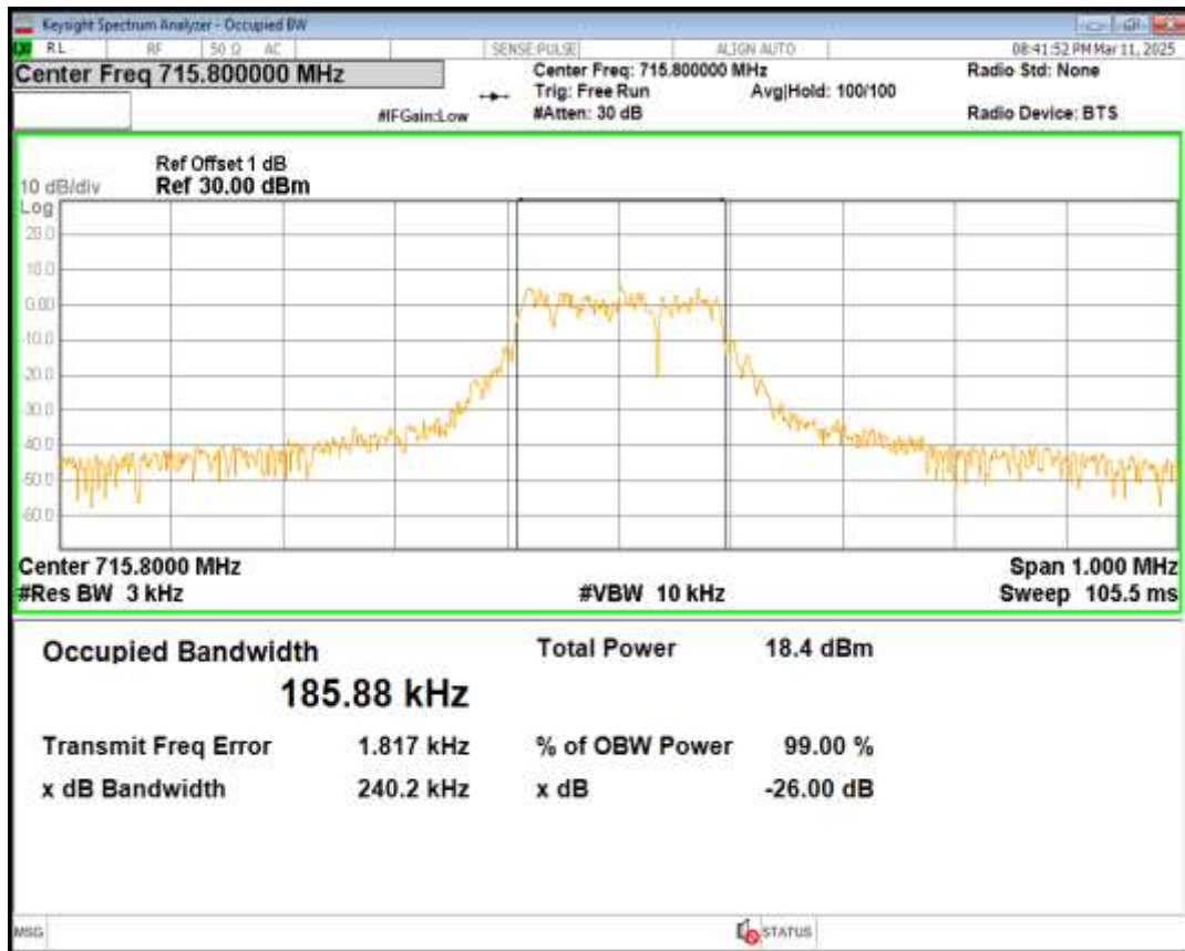
Band12 QPSK Channel=23178 nTones=1@0 Spacing=15kHz
