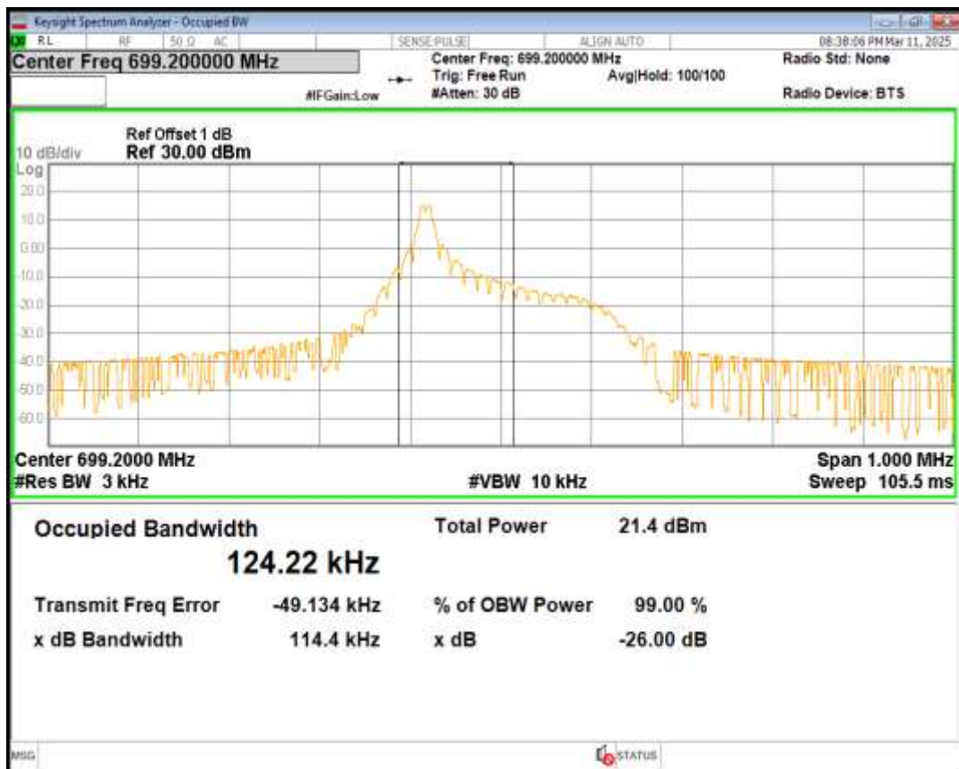
Band12 QPSK Channel=23095 nTones=12@0 Spacing=15kHz
