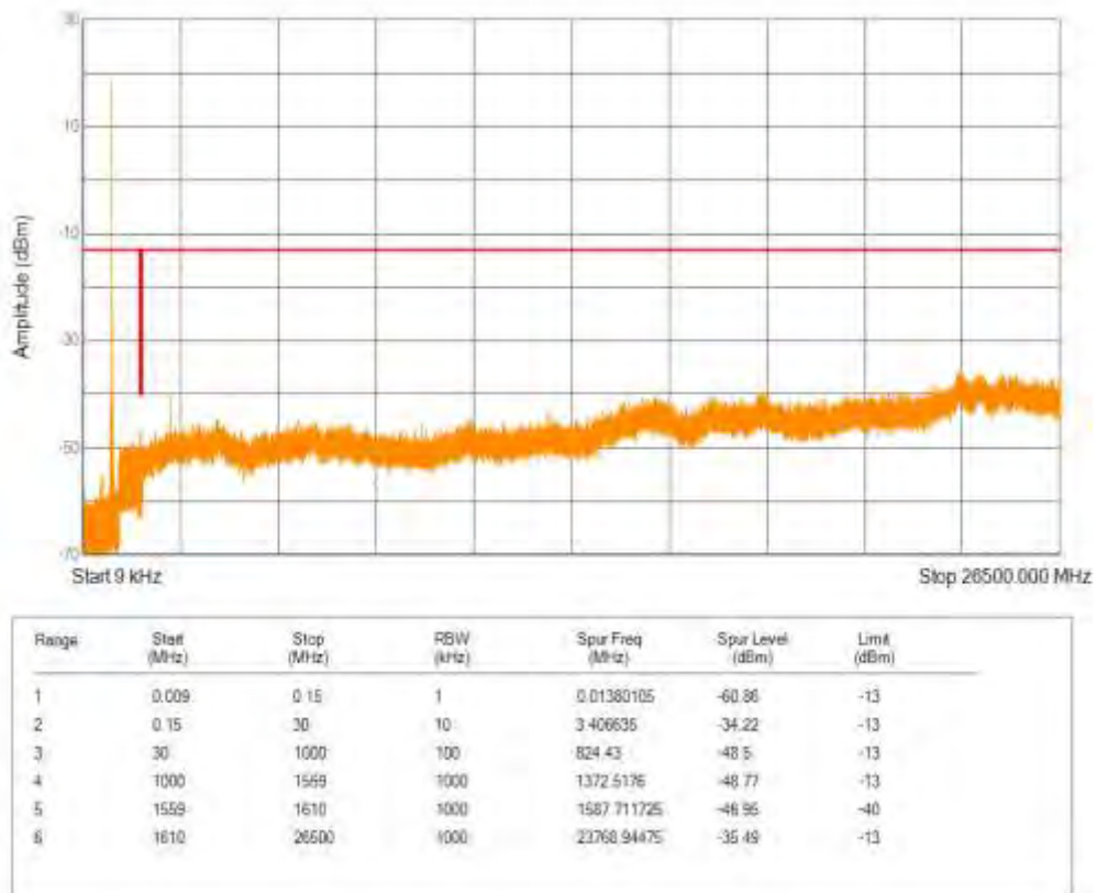
Band14 16QAM BW=5MHz Channel=23355 RB Size=1 Position=#0 NB Index=0
