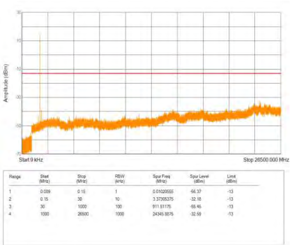
Band2 16QAM BW=1.4MHz Channel=18607 RB Size=5 Position=#0 NB Index=0
