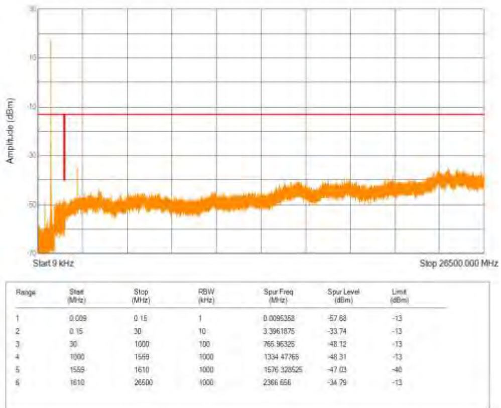
Band14 16QAM BW=5MHz Channel=23305 RB Size=1 Position=#0 NB Index=0
