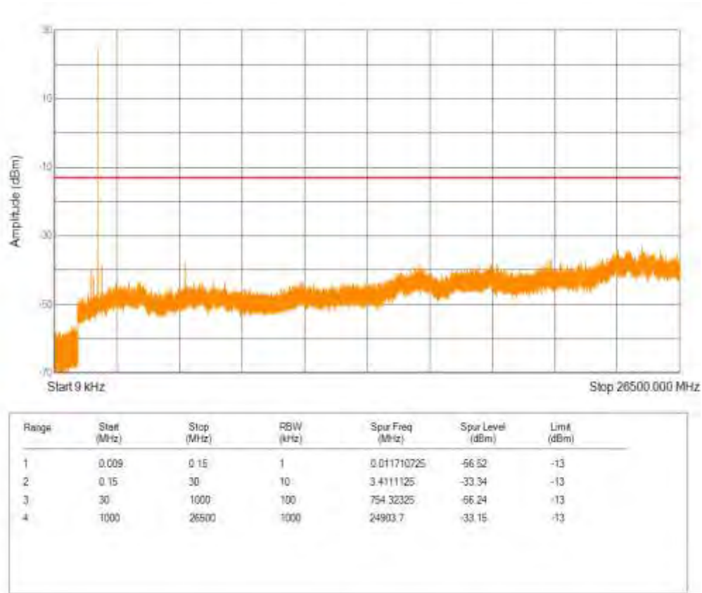
Band2 QPSK BW=1.4MHz Channel=18607 RB Size=6 Position=#0 NB Index=0
