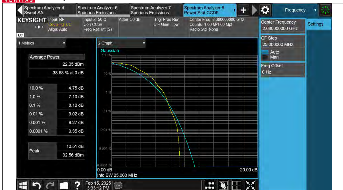
Band41-20MHz-QPSK-41490-100RB#0
