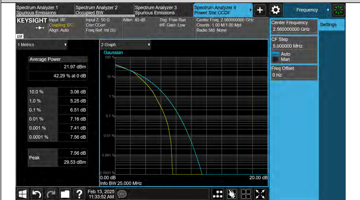
Band7-20MHz-16QAM-21350-27RB#0
