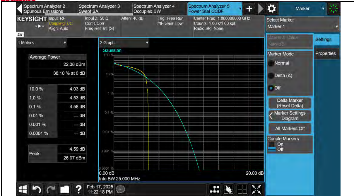
Band25-20MHz-16QAM-26140-1RB#0
