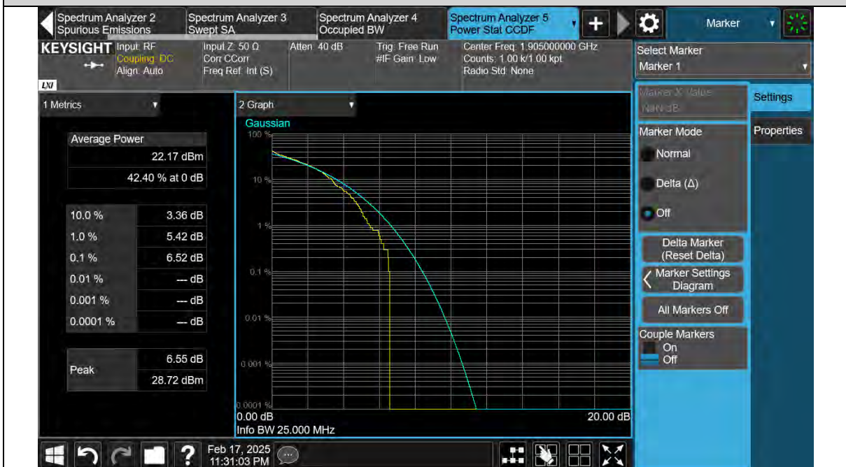
Band25-20MHz-16QAM-26590-27RB#0
