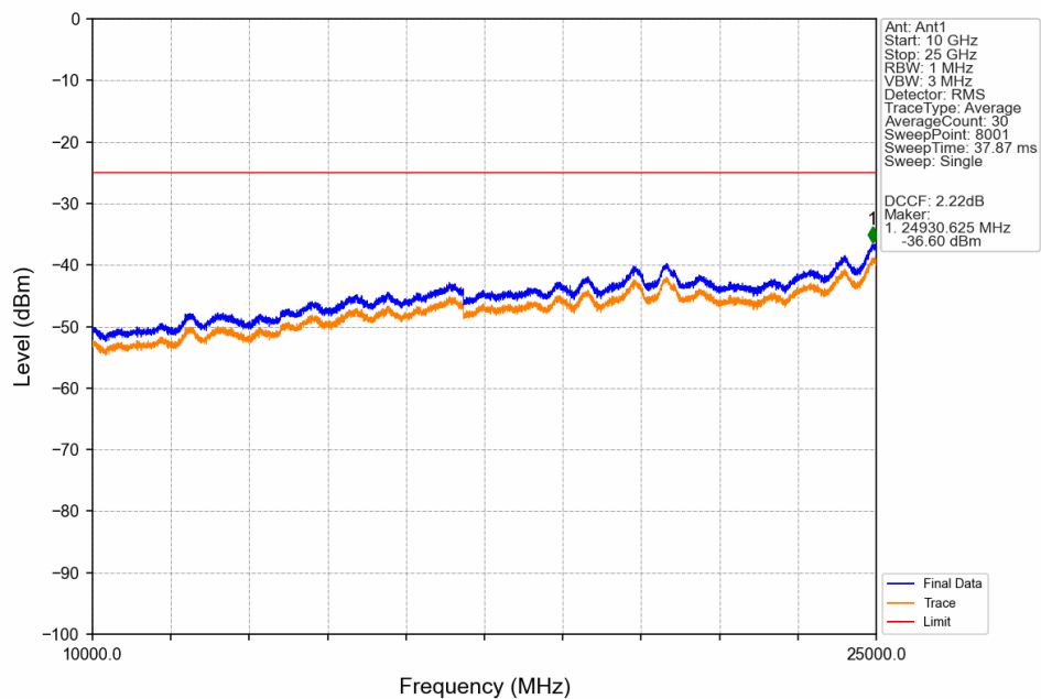
Band41 15MHz QPSK MCH 2593MHz RB 1 0 NTN
