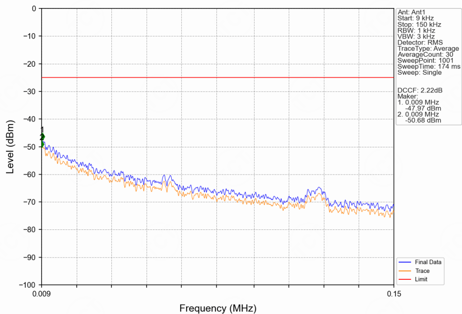
Band41 15MHz 16QAM HCH 2682.5MHz RB 1 0 NTV
