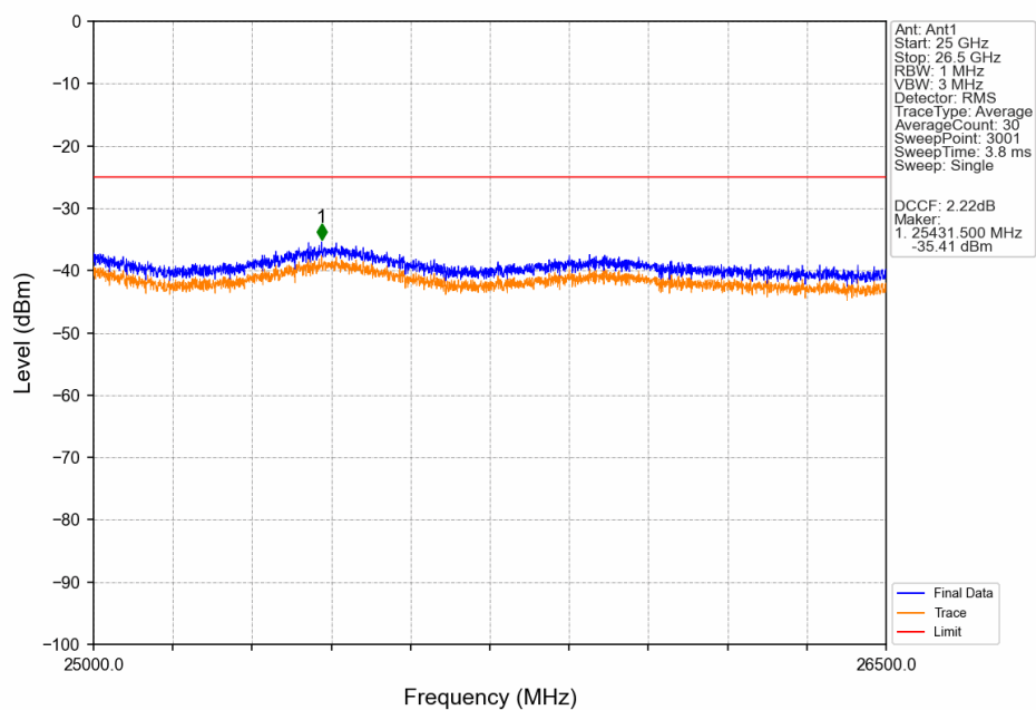
Band41 15MHz QPSK MCH 2593MHz RB 1 0 NTN
