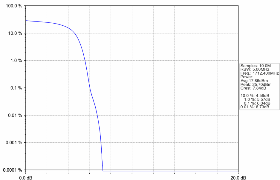
Band4 HSDPA LCH 1712.4MHz Subtest 1 NTN
