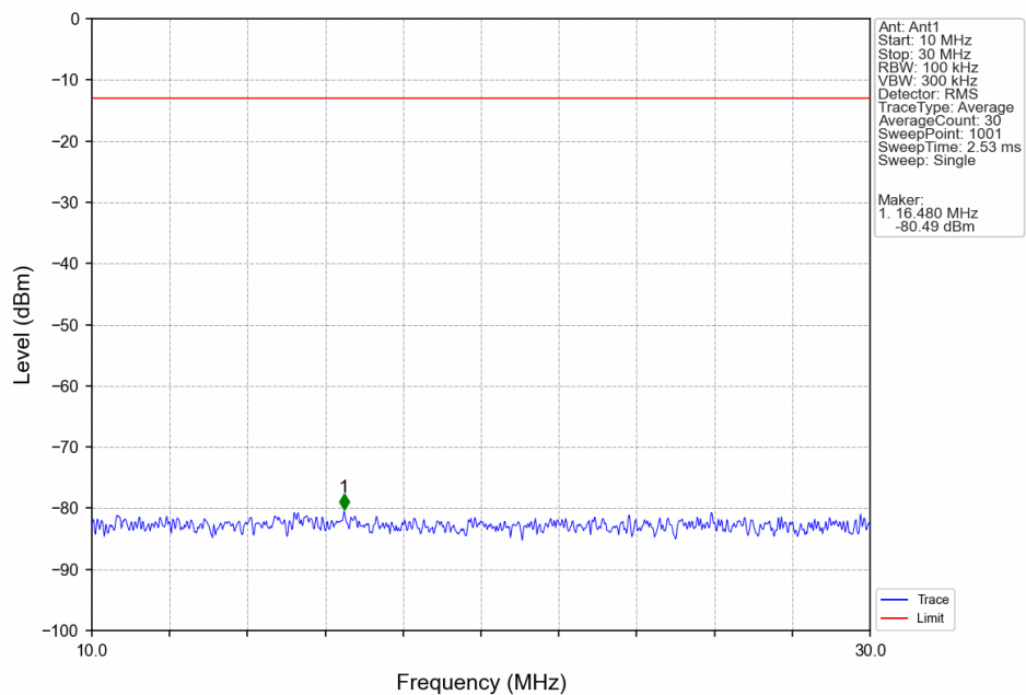
Band4 RMC MCH 1732.6MHz 12.2kbps RMC NTN
