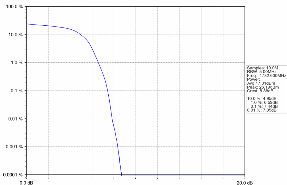
Band4 HSUPA MCH 1732.6MHz Subtest 1 NTV
