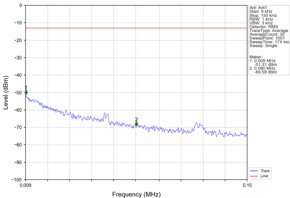
Band4 RMC HCH 1752.6MHz 12.2kbps RMC NTN
