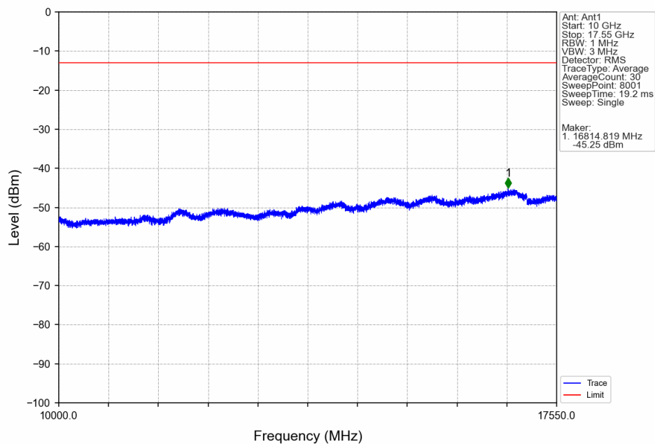
Band4 HSDPA LCH 1712.4MHz Subtest 1 NTN
