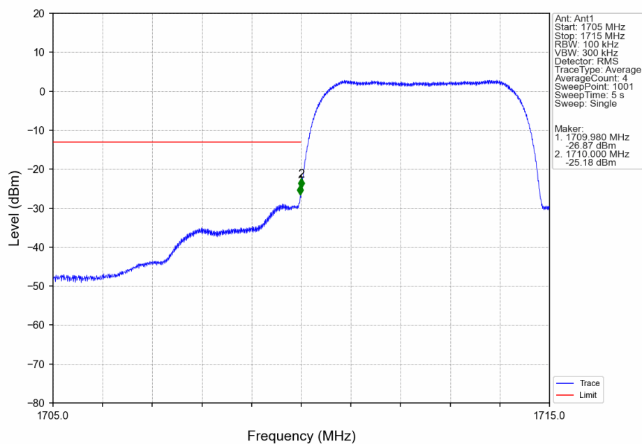
Band4 HSDPA LCH 1712.4MHz Subtest 1 NTN
