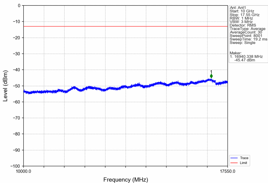
Band4 RMC LCH 1712.4MHz 12.2kbps RMC NTN
