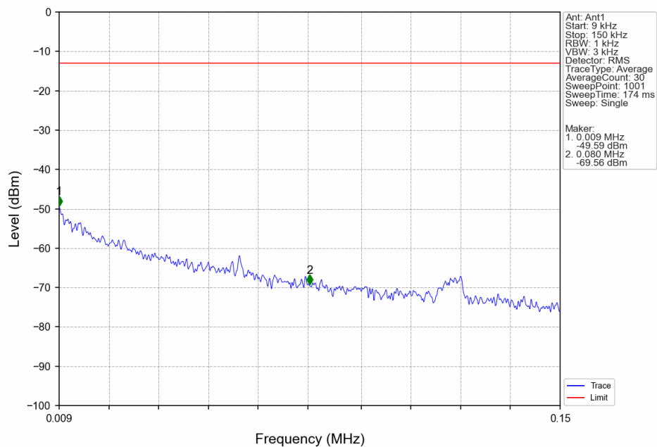
Band2 HSDPA LCH 1852.4MHz Subtest 1 NTNV
