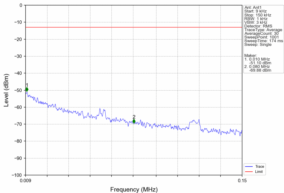
Band2 RMC MCH 1880MHz 12.2kbps RMC NTNV
