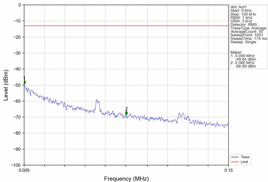
Band2 RMC HCH 1907.6MHz 12.2kbps RMC NTN
