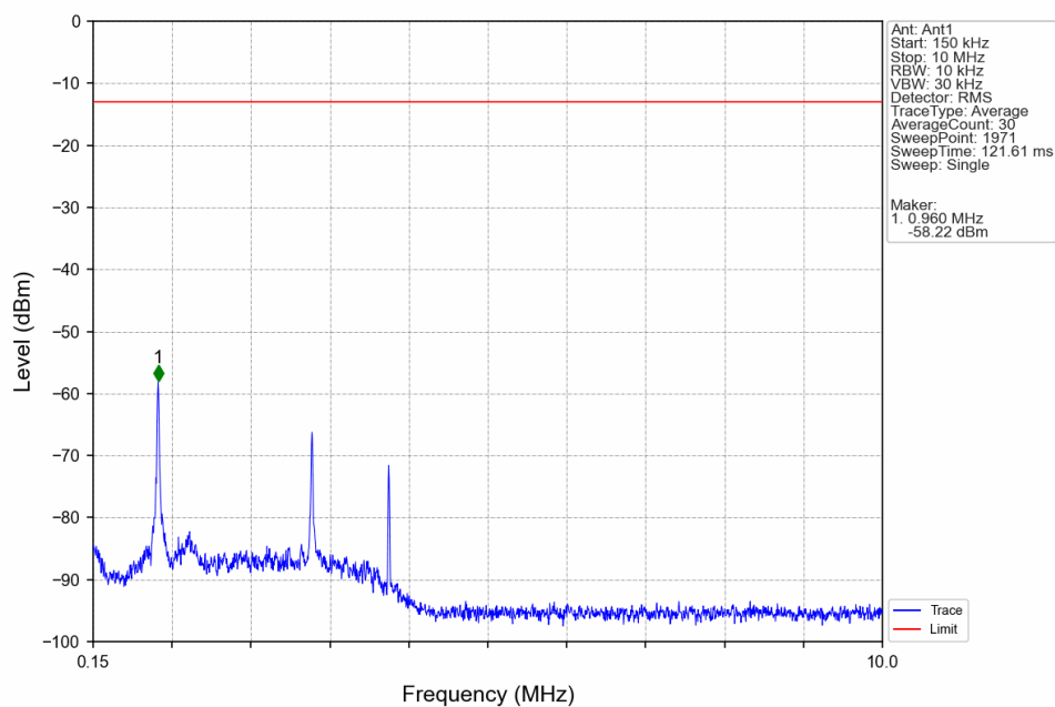
Band2 HSDPA LCH 1852.4MHz Subtest 1 NTNV
