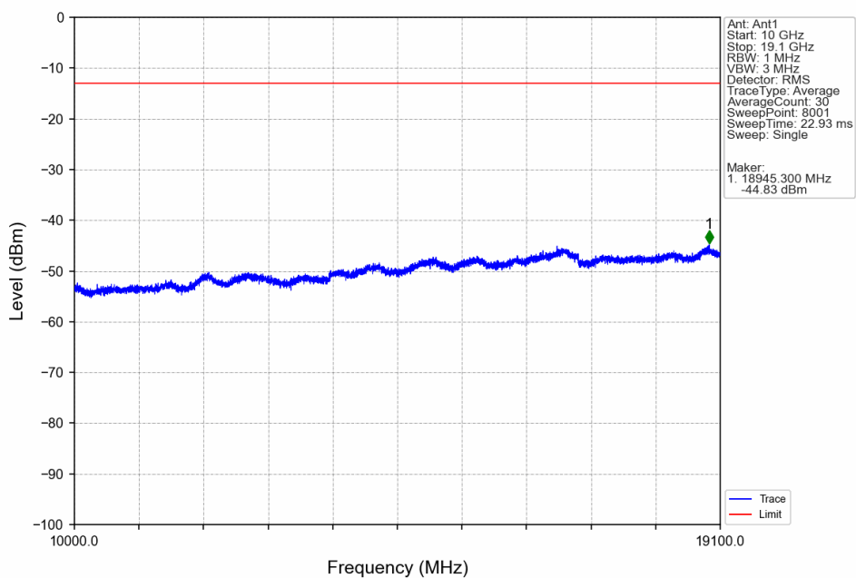
Band2 RMC LCH 1852.4MHz 12.2kbps RMC NTN
