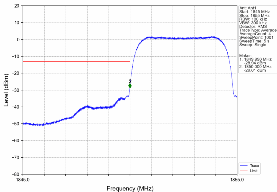
Band2 HSDPA LCH 1852.4MHz Subtest 1 NTN
