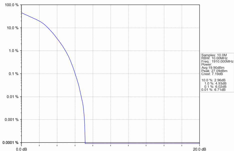
Band25 10MHz 16QAM HCH 1910MHz RB 50 0 NTN
