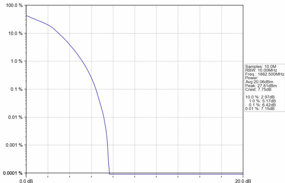
Band25 10MHz 16QAM MCH 1882.5MHz RB 50 0 NTN
