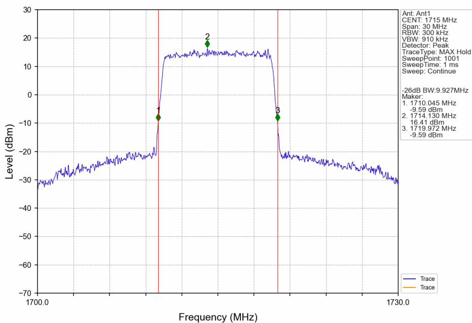
Band4 10MHz 16QAM LCH 1715MHz RB 50 0 NTNV
