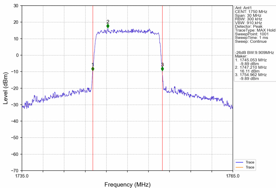
Band4 10MHz 16QAM HCH 1750MHz RB 50 0 NTN
