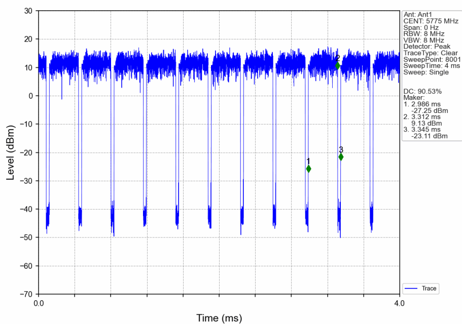
802.11ac(VHT80)_MCH_5775MHz_Ant1_NTNV
