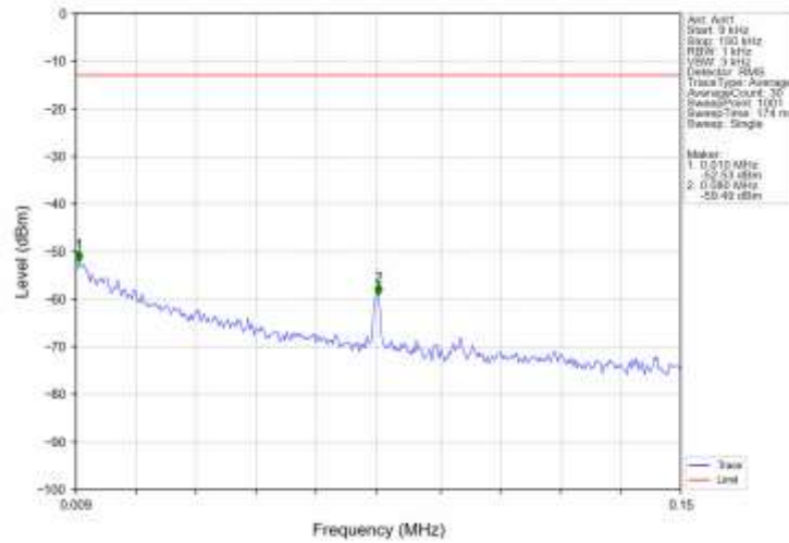
Band66_3MHz_QPSK_HCH_1778.5MHz_RB_1_0_NTV
