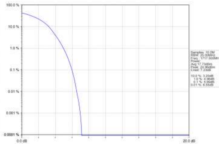
Band66_15MHz_16QAM_LCH_1717.5MHz_RB_75_0_NTNV
