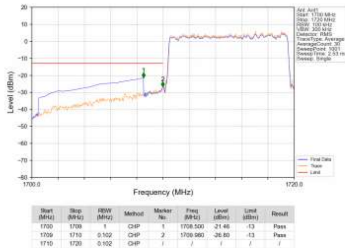
Band66_10MHz_16QAM_LCH_1715MHz_RB_50_0_NTNV
