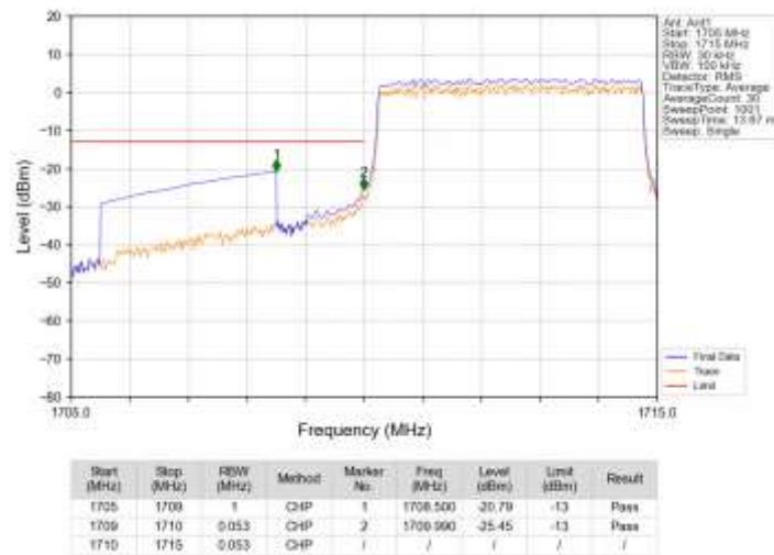
Band66_5MHz_16QAM_LCH_1712.5MHz_RB_25_0_NTNV
