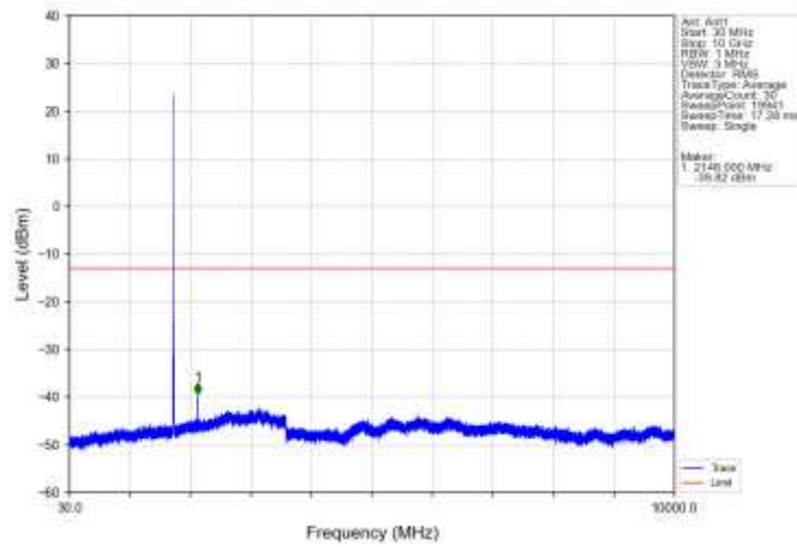
Band66_5MHz_16QAM_MCH_1745MHz_RB_1_0_NTNV
