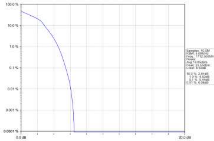
Band66 5MHz 16QAM LCH 1712.5MHz RB 25 0 NTN
