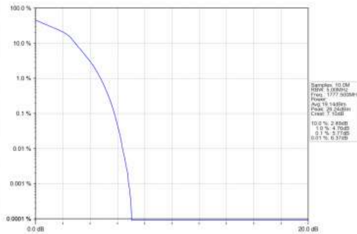
Band66_5MHz_16QAM_HCH_1777.5MHz_RB_25_0_NTNV
