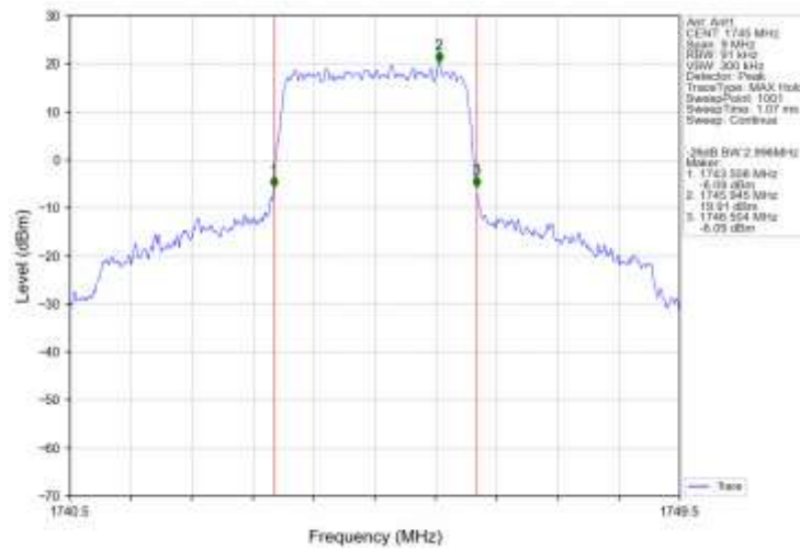
Band66_3MHz_QPSK_MCH_1745MHz_RB_15_0_NTNV
