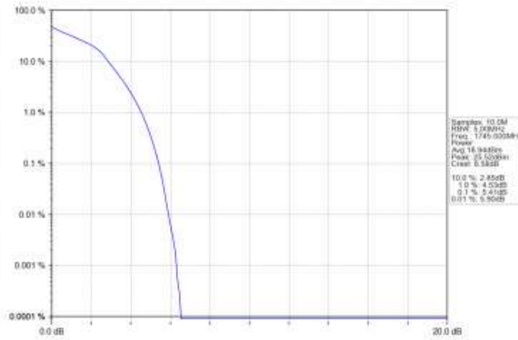
Band66_5MHz_16QAM_MCH_1745MHz_RB_25_0_NTNV
