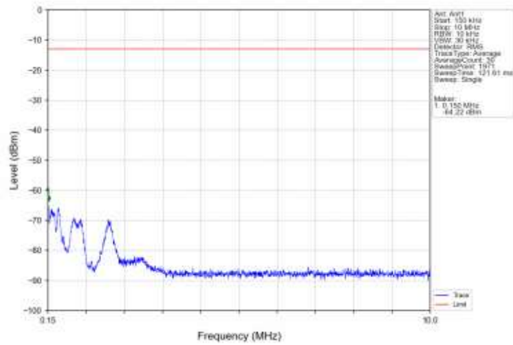
Band66_3MHz_QPSK_HCH_1778.5MHz_RB_1_0_NTV
