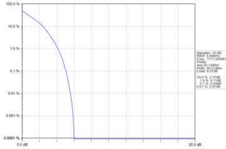
Band66 5MHz QPSK HCH 1777.5MHz RB 25 0 NTN
