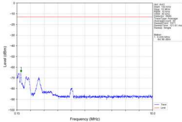
Band66_3MHz_QPSK_LCH_1711.5MHz_RB_1_0_NTV
