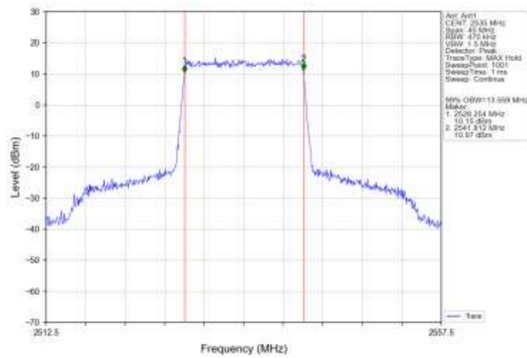
Band7_15MHz_QPSK_MCH_2535MHz_RB_75_0_NTNV
