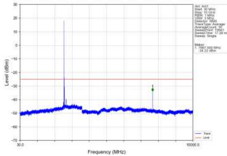
Band7_15MHz_QPSK_HCH_2562.5MHz_RB_1_0_NTNV
