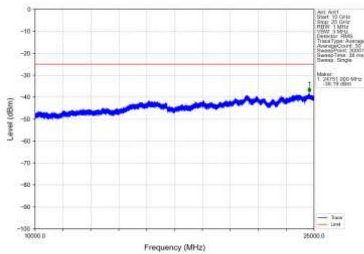
Band7_15MHz_QPSK_LCH_2507.5MHz_RB_1_0_NTNV
