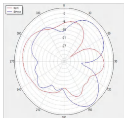
V Phi=90 freq=2020MHz
