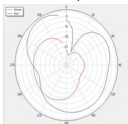
H Theta=90 freq=711MHz
