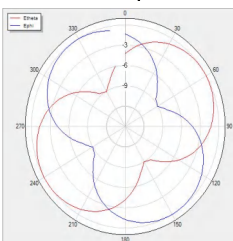
H Theta=0 freq=5800MHz
