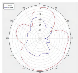
H Theta=90 freq=900MHz
