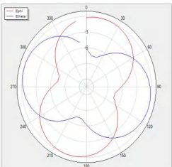
H Theta=0 freq=900MHz
