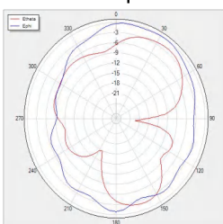
V Phi=90 freq=711MHz
