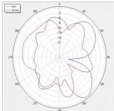
V Phi=90 freq=2520MHz
