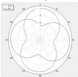
H Theta=0 freq=693MHz
