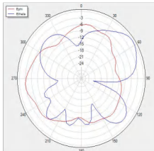
V Phi=0 freq=2600MHz
