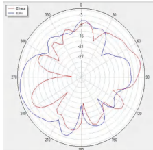
V Phi=90 freq=5200MHz
