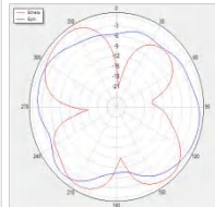
V Phi=0 freq=1575MHz
