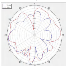
V Phi=90 freq=5800MHz
