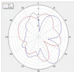
V Phi=90 freq=2360MHz
