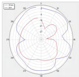
H Theta=90 freq=1575MHz
