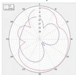
H Theta=90 freq=820MHz
