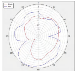
H Theta=90 freq=2450MHz
