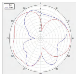
V Phi=0 freq=2020MHz
