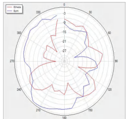
H Theta=90 freq=5200MHz
