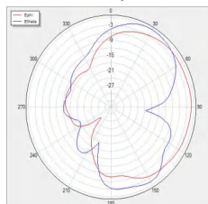
V Phi=90 freq=820MHz
