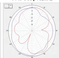
V Phi=0 freq=782MHz
