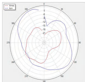
H Theta=90 freq=782MHz
