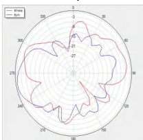
V Phi=90 freq=5400MHz
