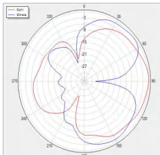
V Phi=90 freq=900MHz
