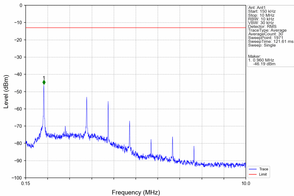
Band5_HSDPA_LCH_826.4MHz_Subtest 1_NTNV
