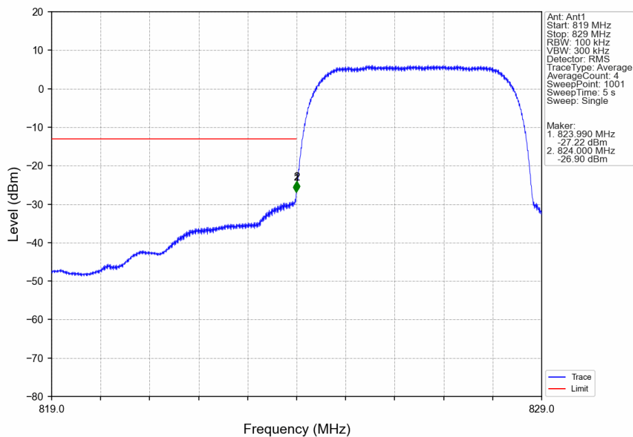
Band5_HSDPA_LCH_826.4MHz_Subtest 1_NTNV
