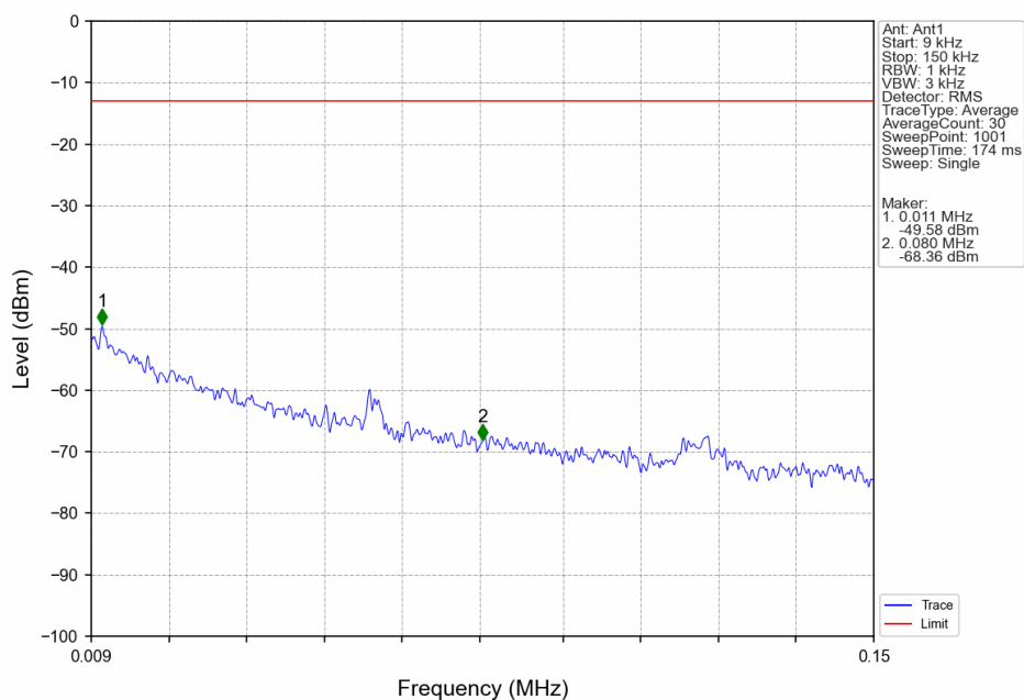
Band2 HSUPA LCH 1852.4MHz Subtest 1 NTV
