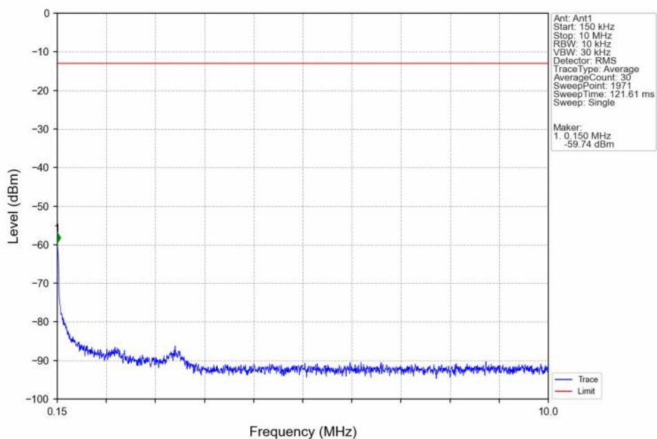
Band66_3MHz_QPSK_HCH_1778.5MHz_RB_1_0_NTV
