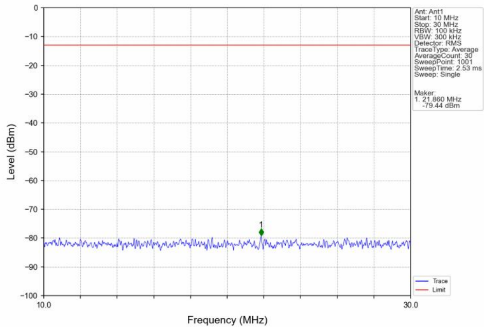
Band66_3MHz_QPSK_HCH_1778.5MHz_RB_1_0_NTV
