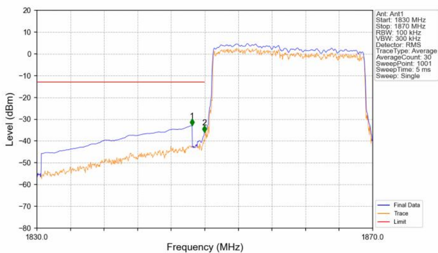
Band25_20MHz_16QAM_LCH_1860MHz_RB_100_0 NTN
