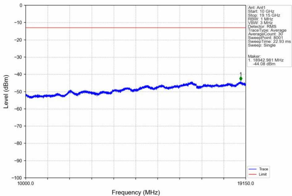
Band25_20MHz_16QAM_LCH_1860MHz_RB_100_0 NTN
