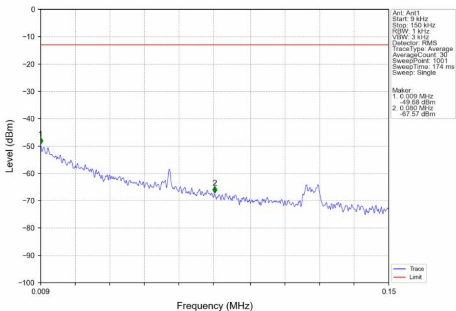
Band25_20MHz_16QAM_HCH_1905MHz_RB_1_0 NTN
