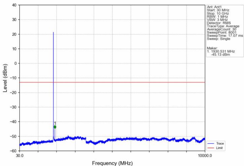
Band25 3MHz 16QAM LCH 1851.5MHz RB 1 0 NTV
