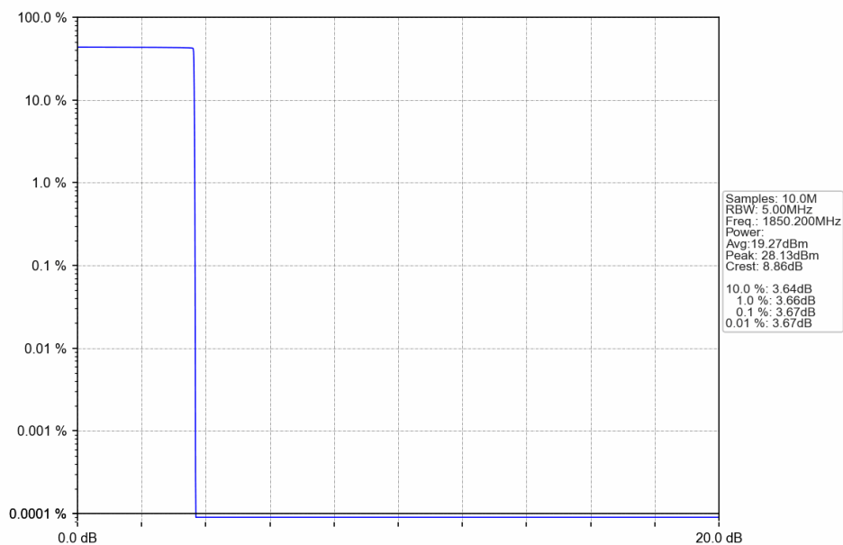
PCS1900 GPRS LCH 1850.2MHz 4 TX Slots NTN
