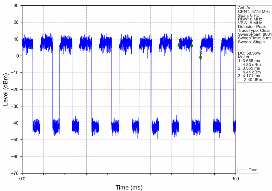
802.11ac(VHT80)_MCH_5775MHz_Ant1_NTNV
