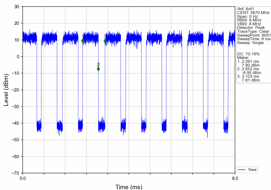
802.11ac(VHT40)_HCH_5670MHz_Ant1_NTNV
