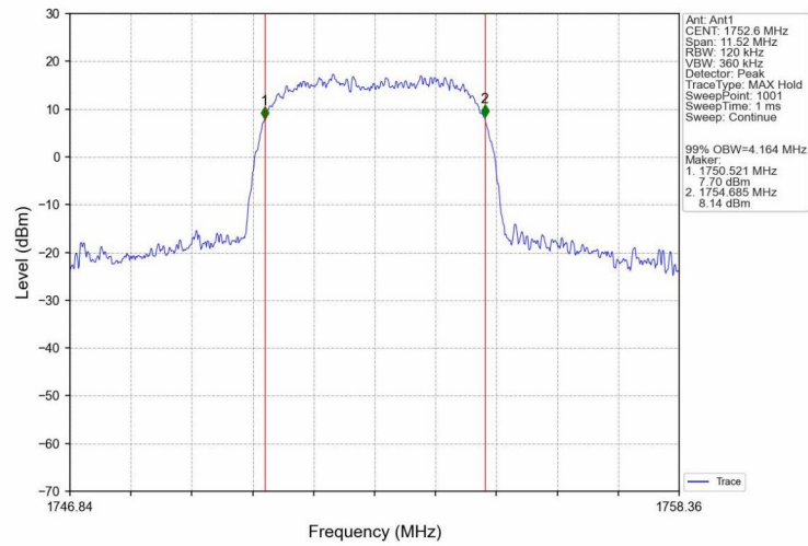
Band4 HSUPA HCH 1752.6MHz_Subtest 1_NTNV
