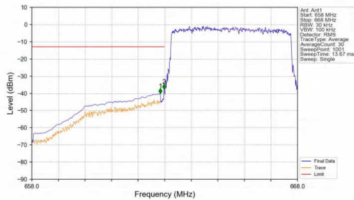
Band71_5MHz_16QAM_LCH_665.5MHz_RB_25_0_NTNV
