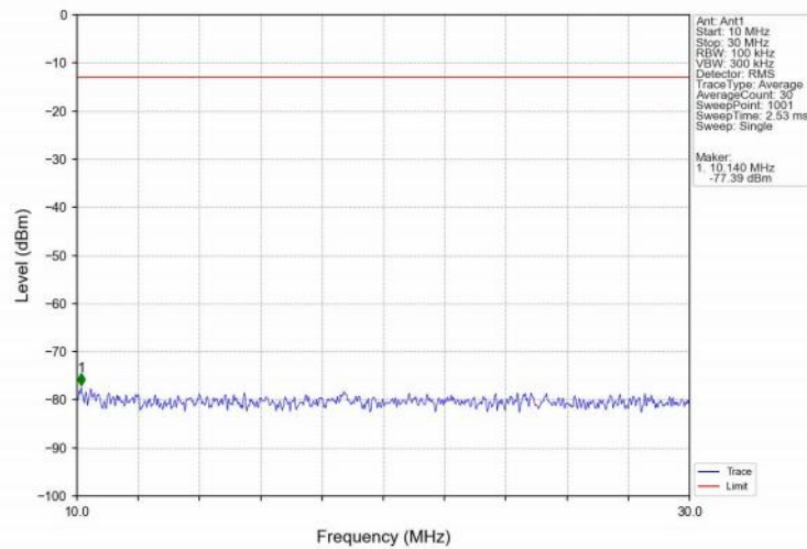
Band71_15MHz_16QAM_LCH_670.5MHz_RB_1_0_NTNV
