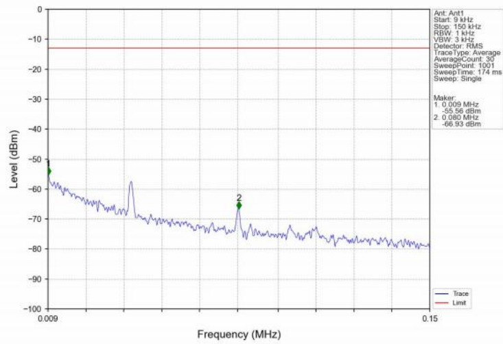
Band71_10MHz_16QAM_HCH_693MHz_RB_1_0_NTNV
