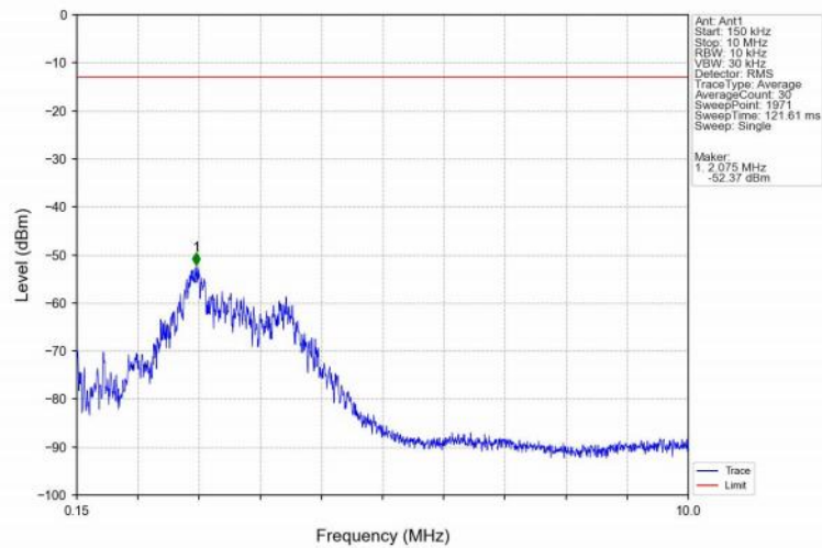
Band71_10MHz_16QAM_MCH_680.5MHz_RB_1_0_NTNV
