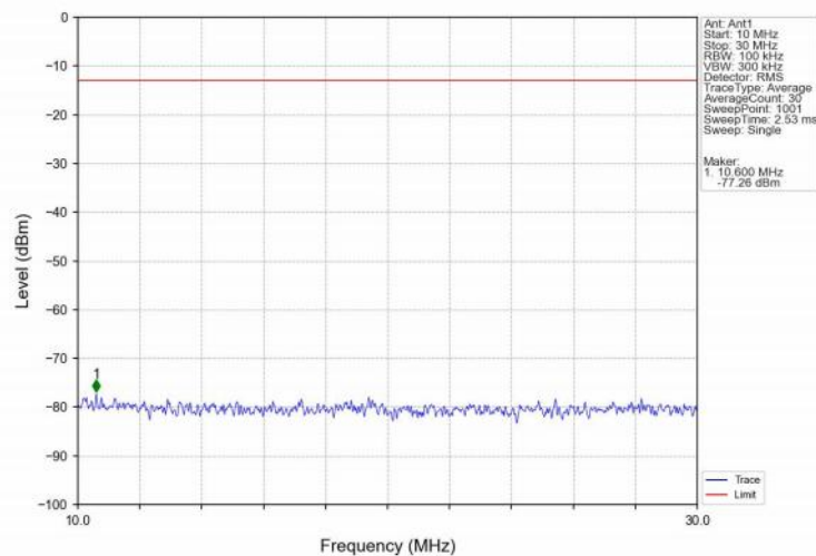
Band71_10MHz_16QAM_LCH_668MHz_RB_1_0_NTNV
