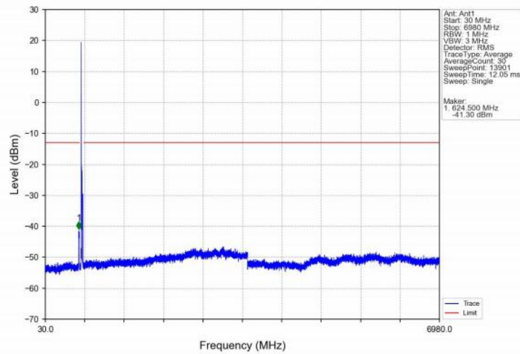
Band71_15MHz_QPSK_LCH_670.5MHz_RB_75_0_NTNV
