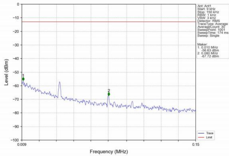
Band71_15MHz_16QAM_HCH_690.5MHz_RB_1_0_NTNV
