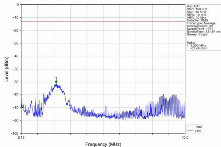
Band66_10MHz_16QAM_MCH_1745MHz_RB_1_0_NTNV
