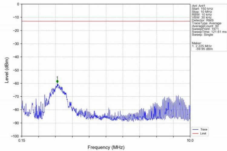
Band66_15MHz_QPSK_LCH_1717.5MHz_RB_1_0_NTNV
