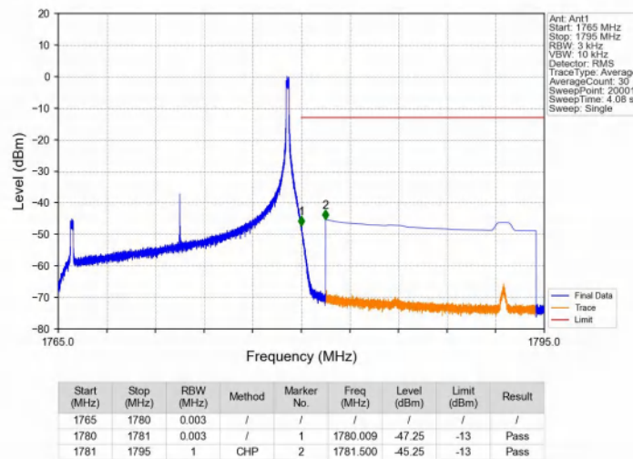
Band66_15MHz_QPSK_HCH_1772.5MHz_RB_1_74_NTNV
