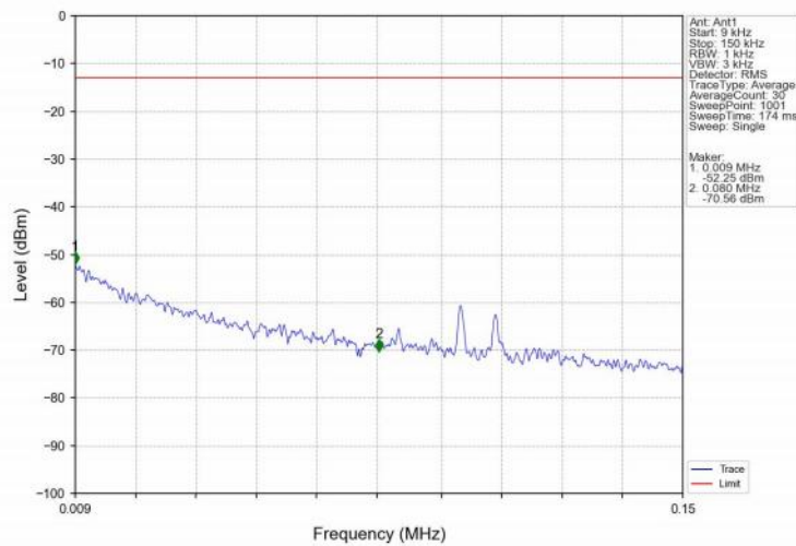
Band66_5MHz_QPSK_LCH_1712.5MHz_RB_1_0_NTNV
