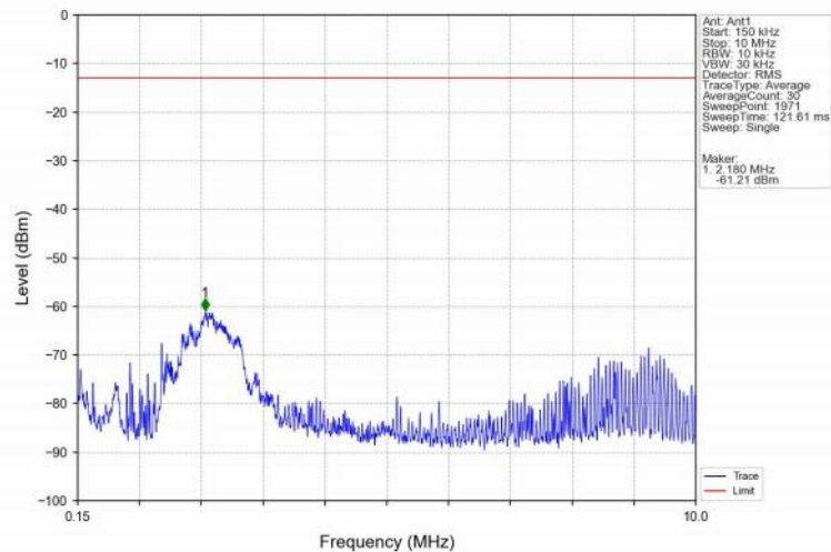
Band66_15MHz_16QAM_LCH_1717.5MHz_RB_1_0_NTNV
