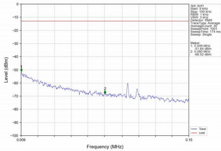
Band66_3MHz_16QAM_LCH_1711.5MHz_RB_1_0_NTNV
