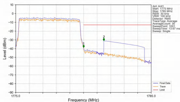
Band66_5MHz_16QAM_HCH_1777.5MHz_RB_25_0_NTNV
