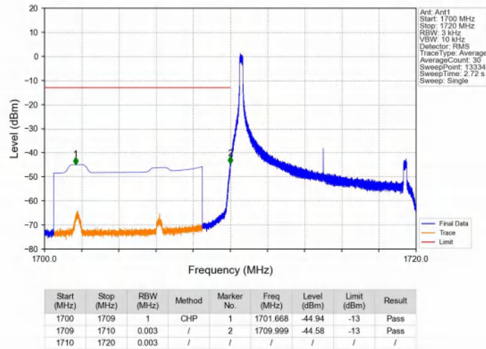
Band66_10MHz_QPSK_LCH_1715MHz_RB_1_0_NTNV
