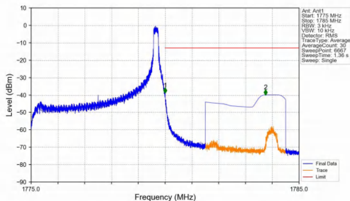
Band66_5MHz_16QAM_HCH_1777.5MHz_RB_1_24_NTNV
