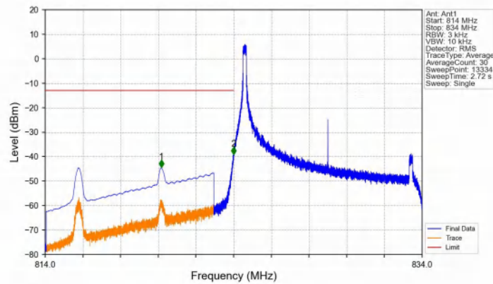
Band26b_10MHz_16QAM_LCH_829MHz_RB_1_0_NTNV
