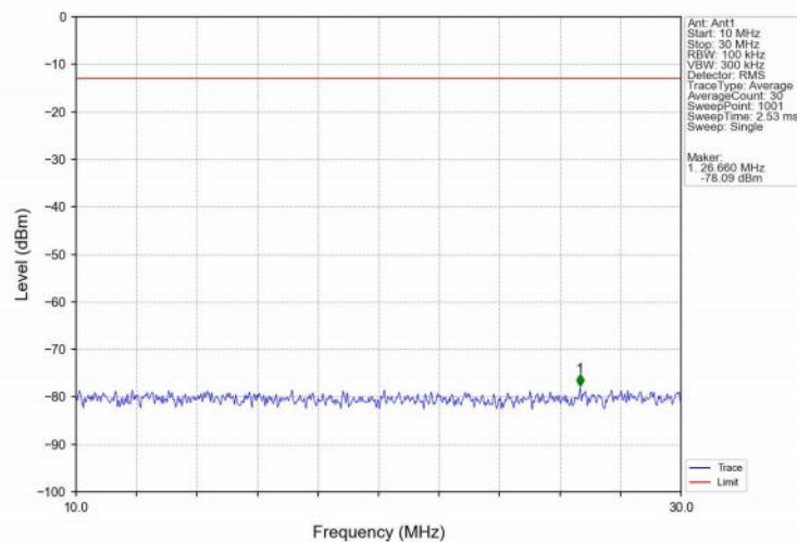
Band26b_3MHz_16QAM_LCH_825.5MHz_RB_1_0_NTNV
