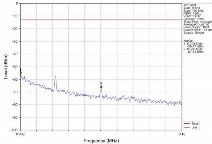
Band26b_15MHz_QPSK_LCH_831.5MHz_RB_1_0_NTNV
