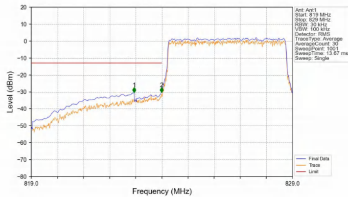
Band26b_5MHz_QPSK_LCH_826.5MHz_RB_25_0_NTNV
