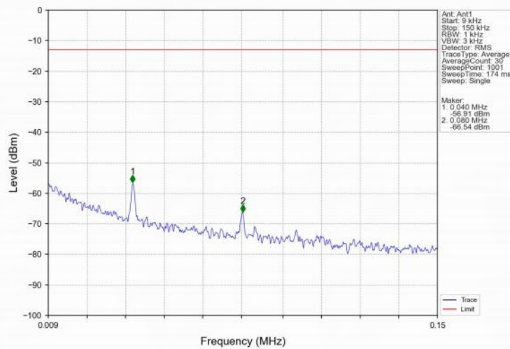
Band26b_5MHz_QPSK_LCH_826.5MHz_RB_1_0_NTNV
