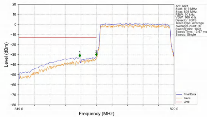
Band26b_5MHz_16QAM_LCH_826.5MHz_RB_25_0_NTNV
