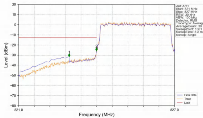
Band26b_3MHz_16QAM_LCH_825.5MHz_RB_15_0_NTNV
