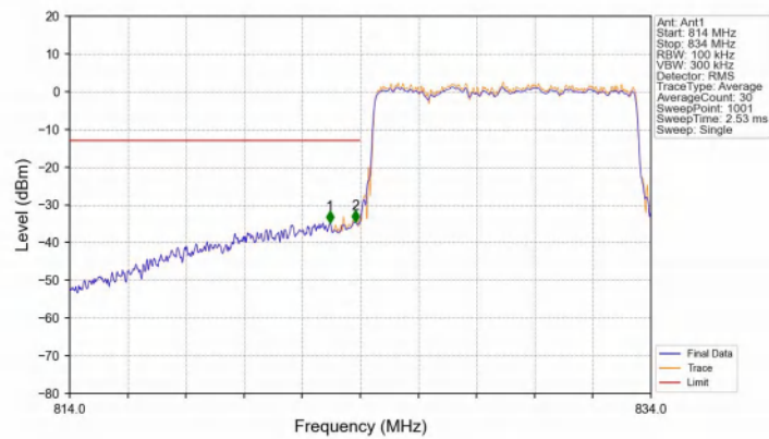
Band26b_10MHz_16QAM_LCH_829MHz_RB_50_0_NTNV
