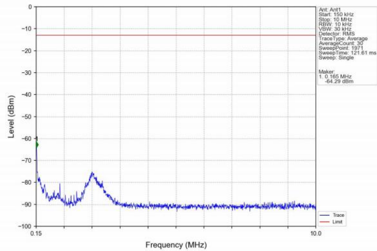
Band26b_5MHz_16QAM_LCH_826.5MHz_RB_1_0_NTNV
