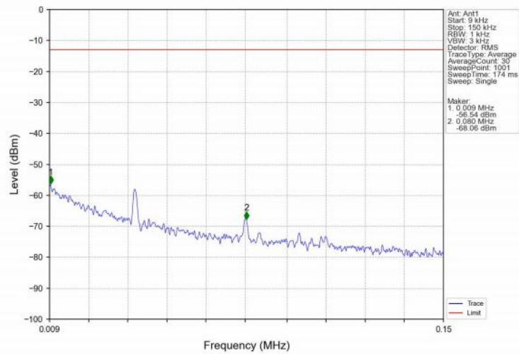
Band26b_15MHz_QPSK_MCH_836.5MHz_RB_1_0_NTNV
