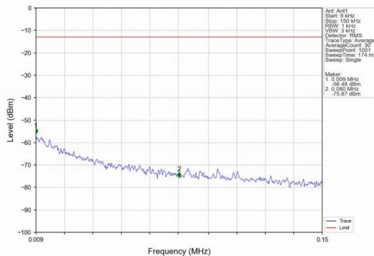
Band26b_3MHz_16QAM_LCH_825.5MHz_RB_1_0_NTNV
