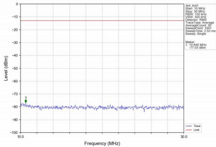
Band26b_15MHz_QPSK_HCH_841.5MHz_RB_1_0_NTNV
