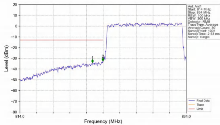
Band26b_10MHz_QPSK_LCH_829MHz_RB_50_0_NTNV
