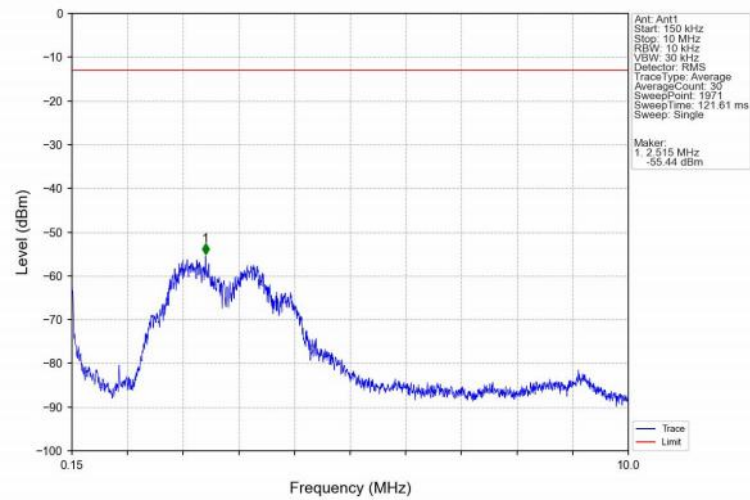
Band26b_10MHz_QPSK_LCH_829MHz_RB_1_0_NTNV
