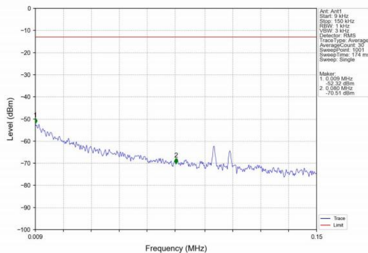
Band25_15MHz_QPSK_LCH_1857.5MHz_RB_1_0_NTNV
