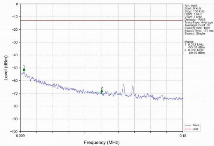
Band25_3MHz_QPSK_HCH_1913.5MHz_RB_1_0_NTNV
