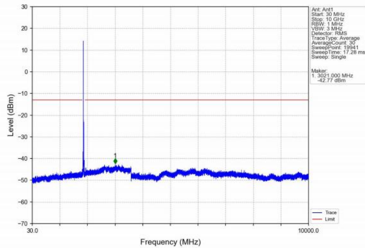
Band25_20MHz_QPSK_MCH_1882.5MHz_RB_1_0_NTNV
