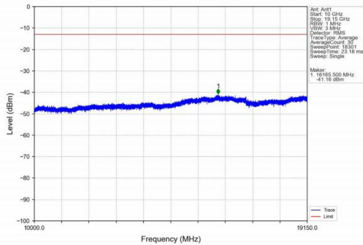
Band25_10MHz_16QAM_HCH_1910MHz_RB_1_0_NTNV
