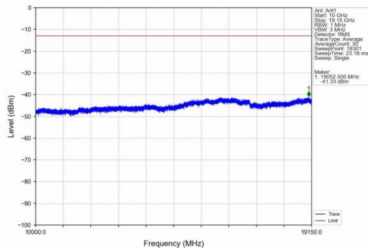
Band25_15MHz_QPSK_LCH_1857.5MHz_RB_1_0_NTNV
