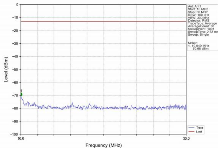
Band25_3MHz_16QAM_HCH_1913.5MHz_RB_1_0_NTNV
