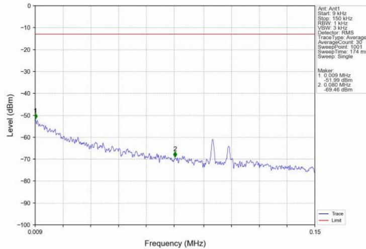
Band25_5MHz_QPSK_LCH_1852.5MHz_RB_1_0_NTNV
