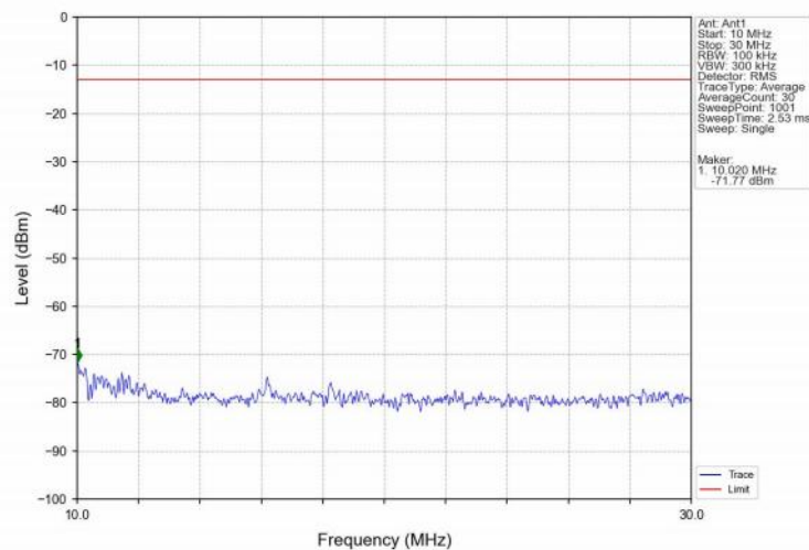
Band25_15MHz_QPSK_MCH_1882.5MHz_RB_1_0_NTNV
