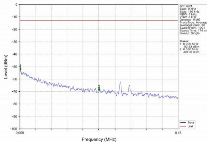
Band25_3MHz_16QAM_HCH_1913.5MHz_RB_1_0_NTNV
