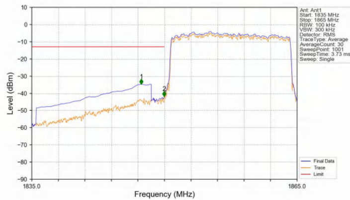
Band25_15MHz_16QAM_LCH_1857.5MHz_RB_75_0_NTNV
