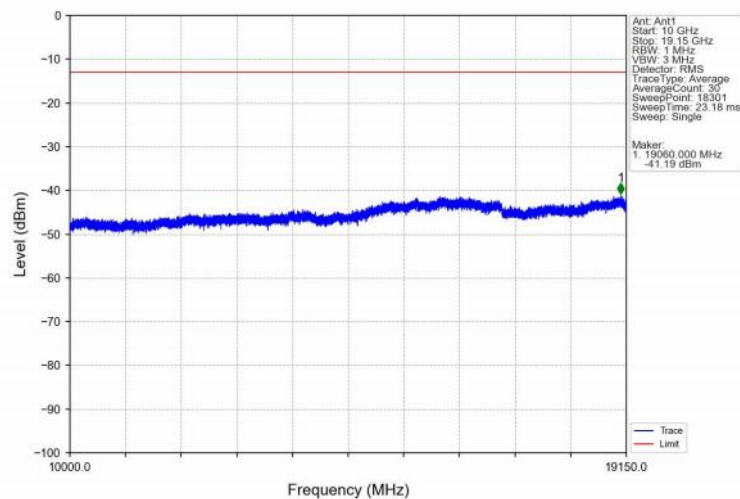
Band25_20MHz_16QAM_HCH_1905MHz_RB_1_0_NTNV
