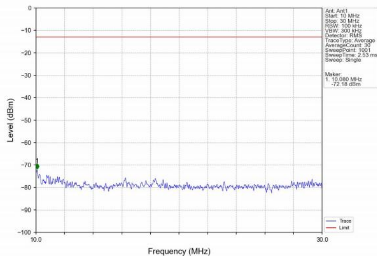
Band25_5MHz_16QAM_HCH_1912.5MHz_RB_1_0_NTNV
