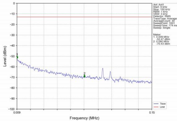
Band25_5MHz_QPSK_HCH_1912.5MHz_RB_1_0_NTNV
