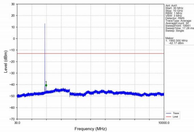
Band25_5MHz_16QAM_HCH_1912.5MHz_RB_1_0_NTNV
