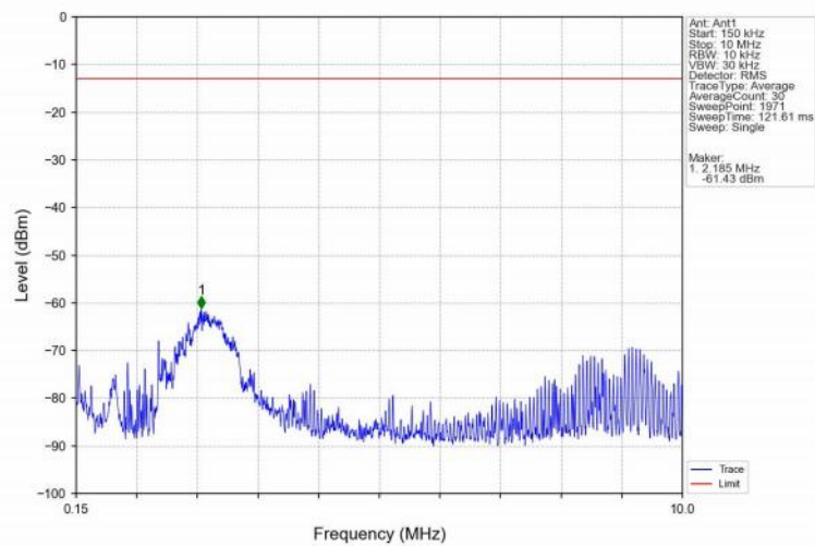
Band25_5MHz_16QAM_LCH_1852.5MHz_RB_1_0_NTNV
