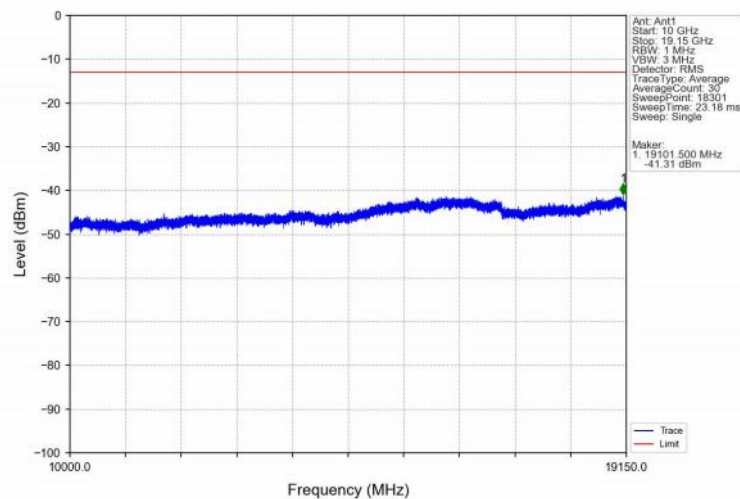
Band25_5MHz_QPSK_MCH_1882.5MHz_RB_1_0_NTNV
