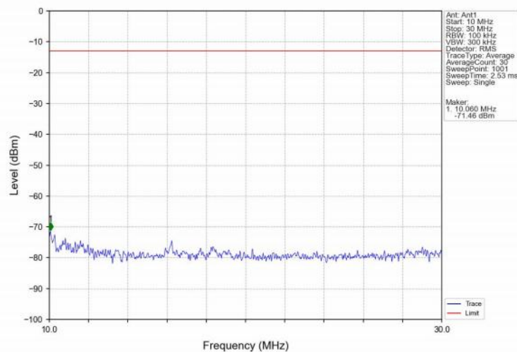
Band25_20MHz_QPSK_MCH_1882.5MHz_RB_1_0_NTNV
