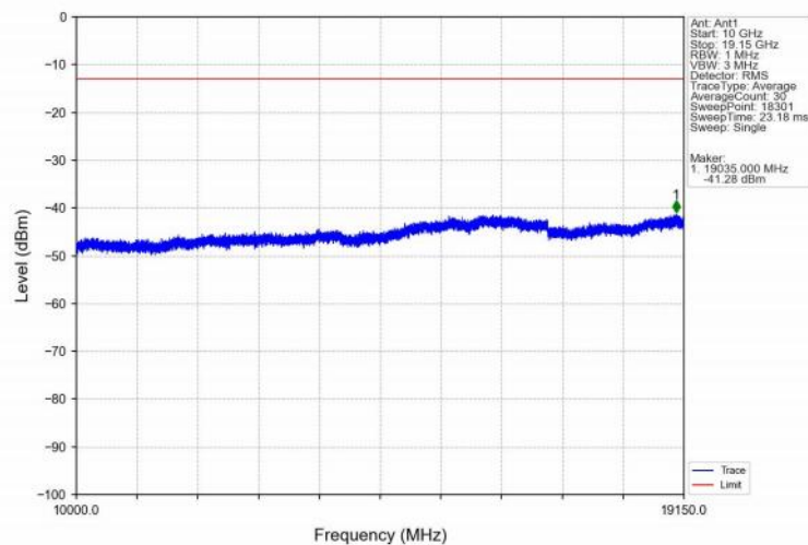
Band25_3MHz_16QAM_HCH_1913.5MHz_RB_1_0_NTNV
