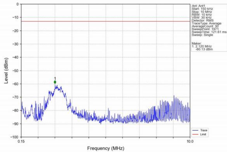
Band25_15MHz_QPSK_MCH_1882.5MHz_RB_1_0_NTNV
