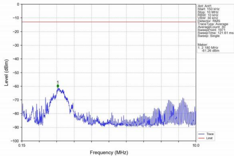
Band25_3MHz_16QAM_MCH_1882.5MHz_RB_1_0_NTNV
