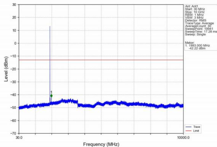
Band25_5MHz_QPSK_HCH_1912.5MHz_RB_1_0_NTNV
