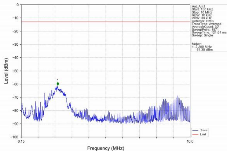
Band25_5MHz_16QAM_MCH_1882.5MHz_RB_1_0_NTNV
