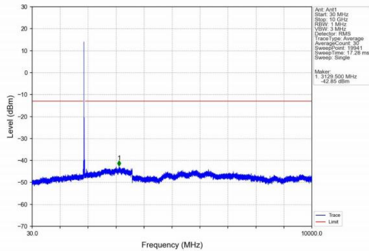
Band25_15MHz_QPSK_MCH_1882.5MHz_RB_1_0_NTNV
