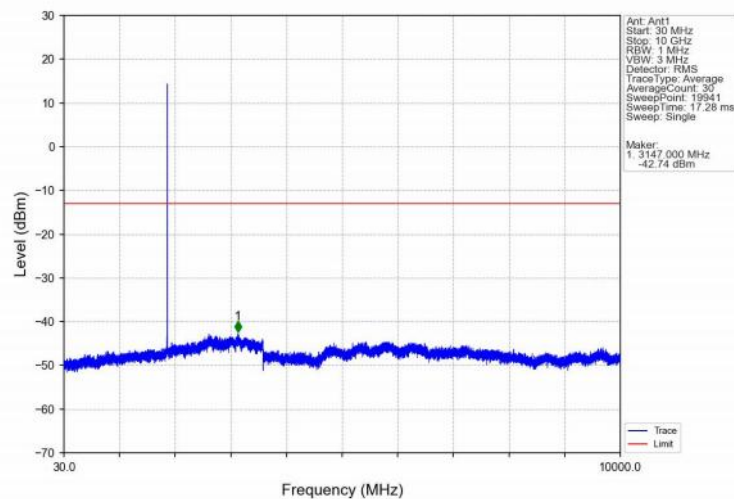
Band25_3MHz_16QAM_MCH_1882.5MHz_RB_1_0_NTNV
