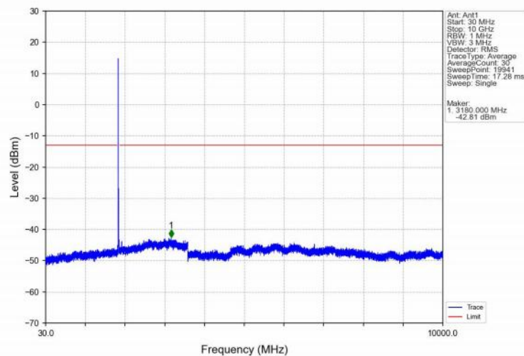
Band25_15MHz_16QAM_LCH_1857.5MHz_RB_1_0_NTNV
