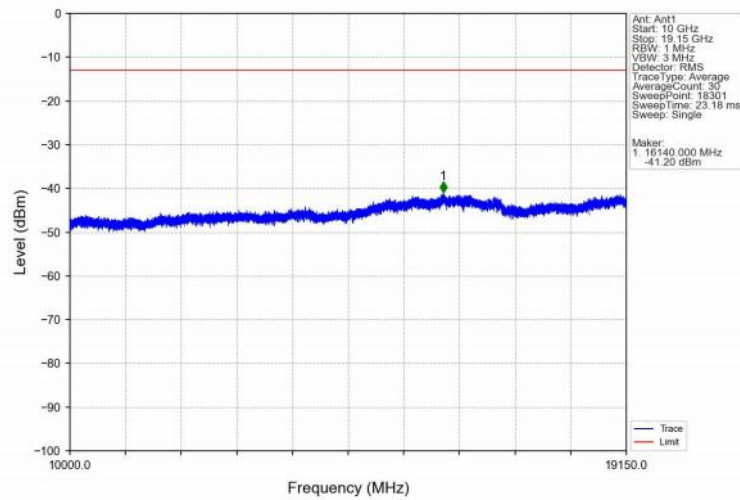
Band25_5MHz_QPSK_HCH_1912.5MHz_RB_1_24_NTNV
