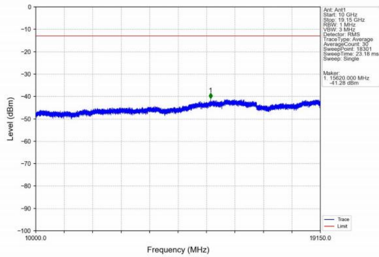
Band25_20MHz_16QAM_LCH_1860MHz_RB_100_0_NTNV
