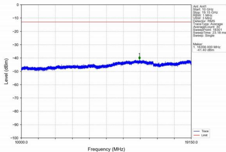
Band25_3MHz_QPSK_MCH_1882.5MHz_RB_1_0_NTNV
