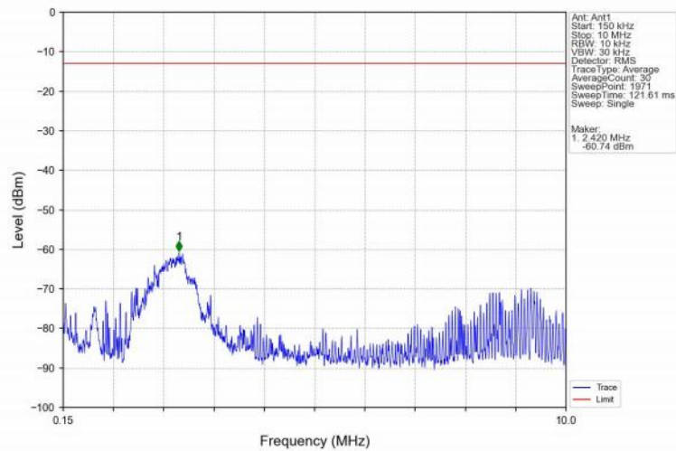
Band25_15MHz_16QAM_LCH_1857.5MHz_RB_1_0_NTNV
