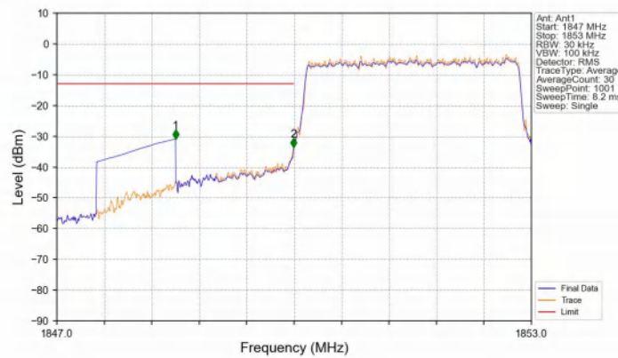
Band25_3MHz_16QAM_LCH_1851.5MHz_RB_15_0_NTNV
