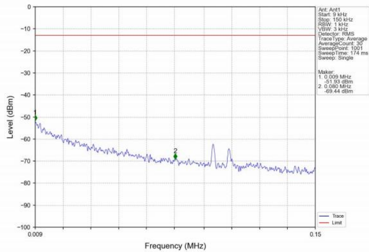
Band25_5MHz_16QAM_MCH_1882.5MHz_RB_1_0_NTNV
