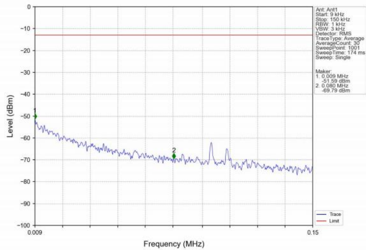
Band25_15MHz_QPSK_HCH_1907.5MHz_RB_1_0_NTNV
