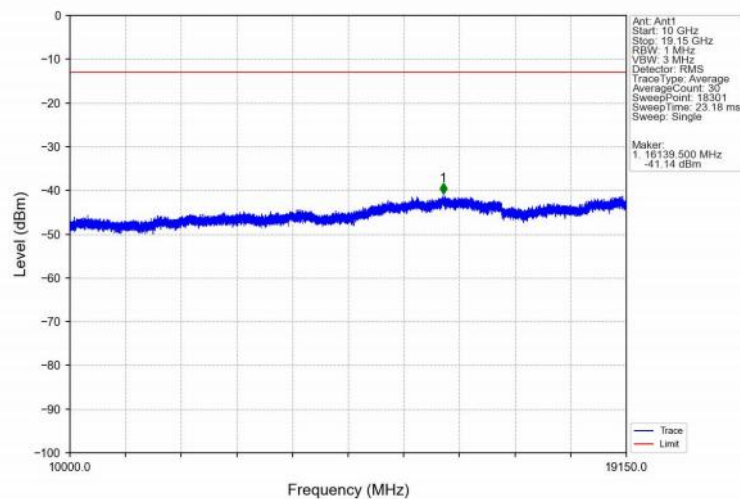
Band25_20MHz_QPSK_MCH_1882.5MHz_RB_1_0_NTNV
