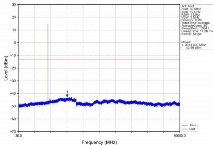
Band25_3MHz_16QAM_LCH_1851.5MHz_RB_1_0_NTNV
