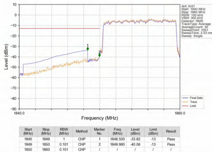
Band25_10MHz_16QAM_LCH_1855MHz_RB_50_0_NTNV
