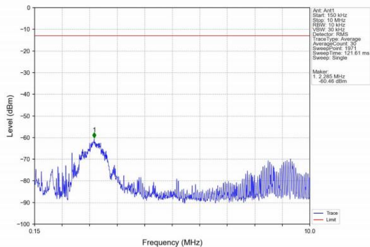
Band25_15MHz_QPSK_HCH_1907.5MHz_RB_1_0_NTNV
