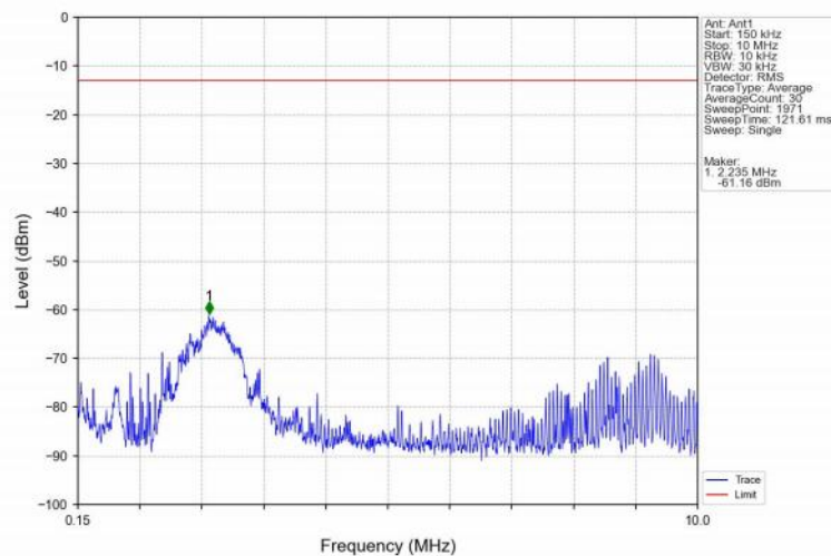
Band25_3MHz_QPSK_HCH_1913.5MHz_RB_1_0_NTNV
