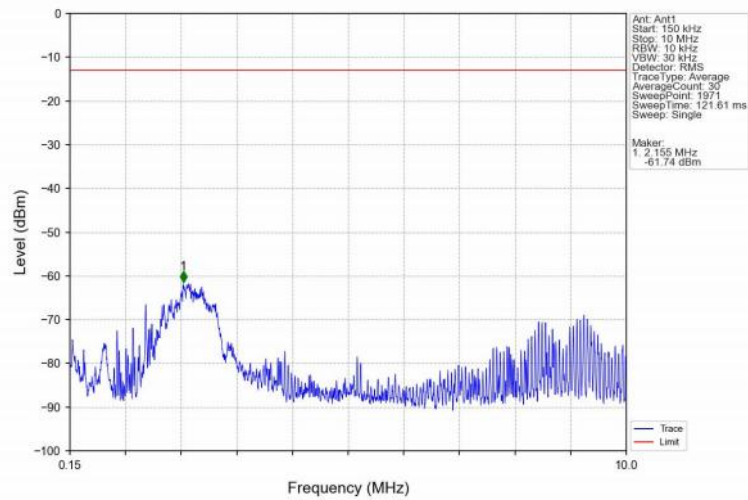
Band25_5MHz_QPSK_MCH_1882.5MHz_RB_1_0_NTNV
