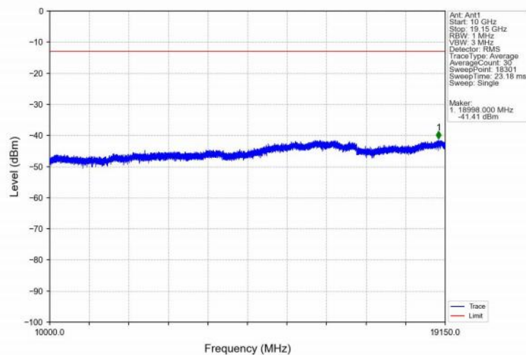
Band25_5MHz_16QAM_HCH_1912.5MHz_RB_1_0_NTNV
