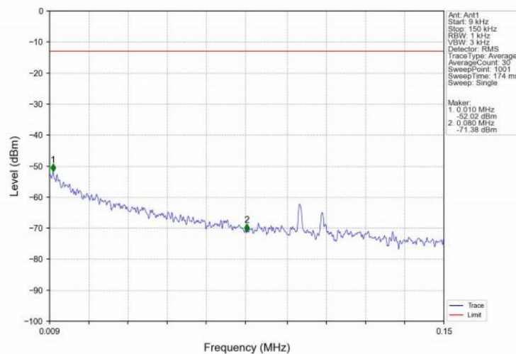
Band25_20MHz_16QAM_HCH_1905MHz_RB_1_0_NTNV
