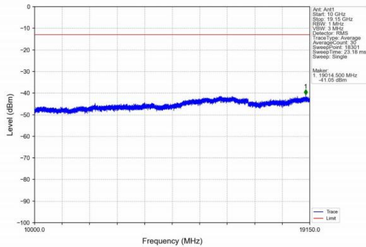
Band25_3MHz_QPSK_HCH_1913.5MHz_RB_1_14_NTNV
