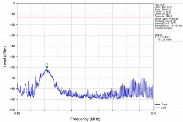
Band25_3MHz_16QAM_HCH_1913.5MHz_RB_1_0_NTNV
