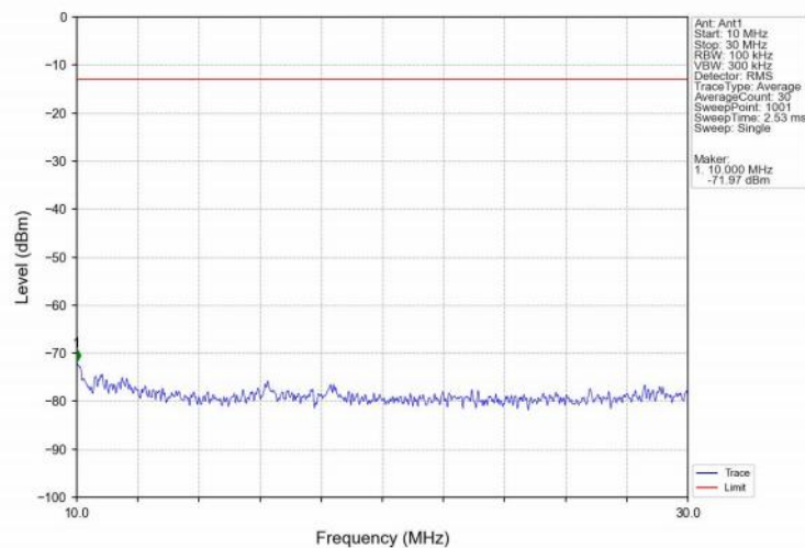
Band25_10MHz_QPSK_MCH_1882.5MHz_RB_1_0_NTNV
