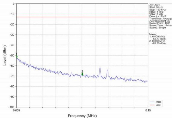
Band25_10MHz_16QAM_HCH_1910MHz_RB_1_0_NTNV
