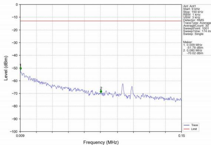
Band25_5MHz_16QAM_HCH_1912.5MHz_RB_1_0_NTNV
