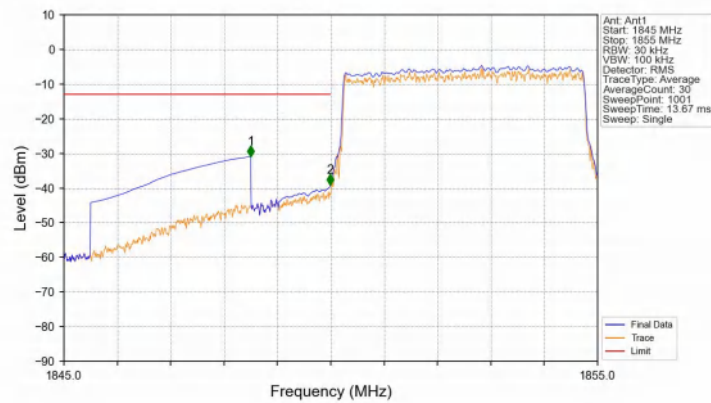
Band25_5MHz_16QAM_LCH_1852.5MHz_RB_25_0_NTNV
