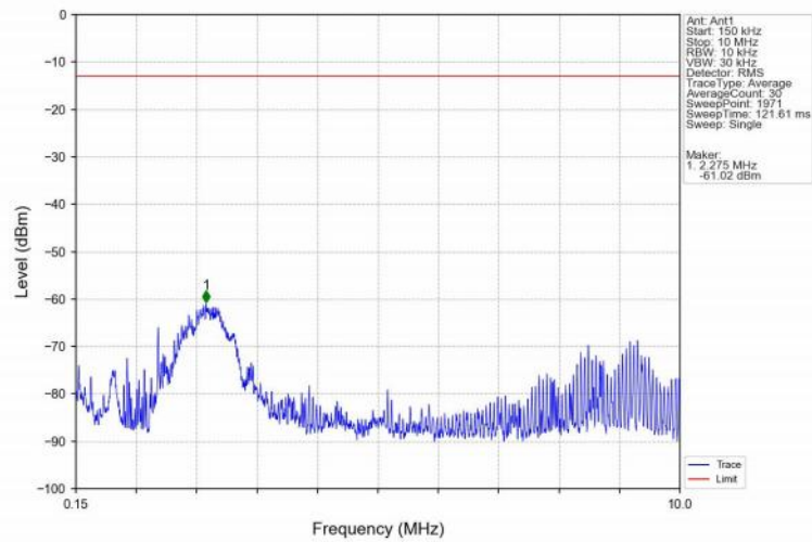
Band25_5MHz_QPSK_LCH_1852.5MHz_RB_1_0_NTNV
