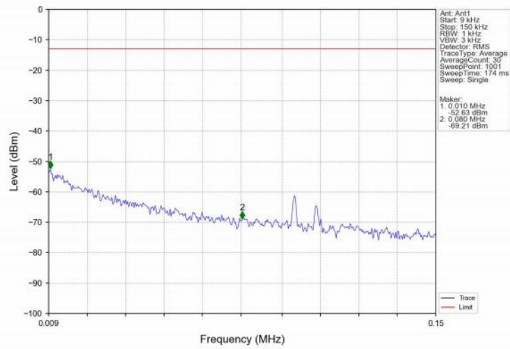
Band25_3MHz_16QAM_MCH_1882.5MHz_RB_1_0_NTNV
