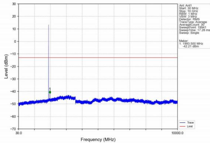
Band25_3MHz_16QAM_HCH_1913.5MHz_RB_1_0_NTNV
