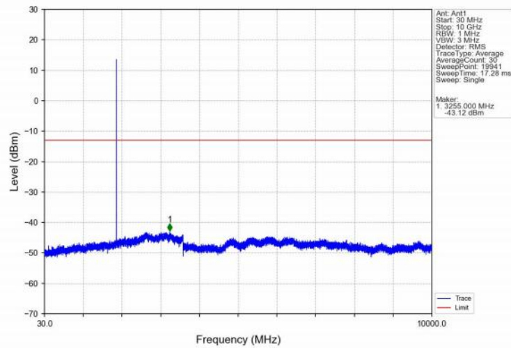
Band25_3MHz_QPSK_MCH_1882.5MHz_RB_1_0_NTNV
