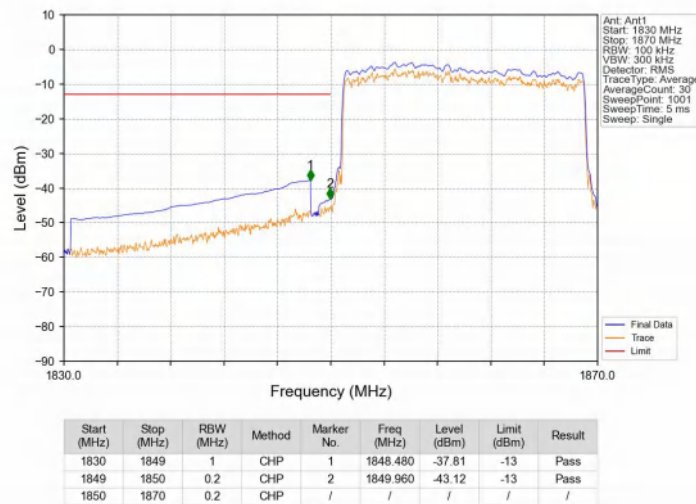
Band25_20MHz_16QAM_LCH_1860MHz_RB_100_0_NTNV
