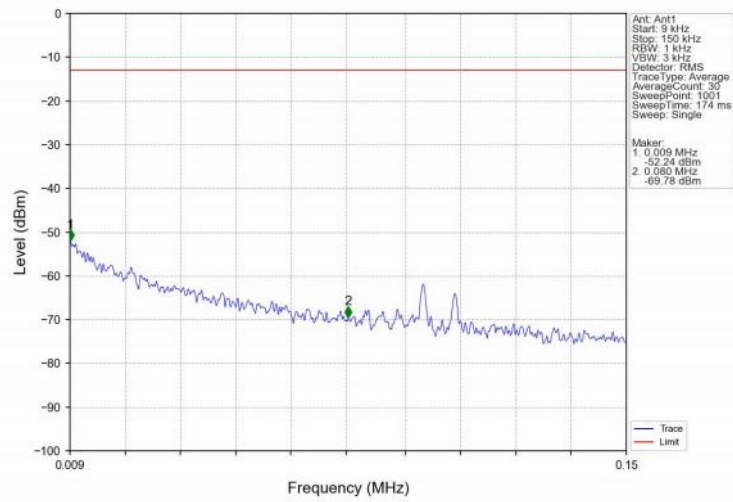
Band25_15MHz_16QAM_LCH_1857.5MHz_RB_1_0_NTNV
