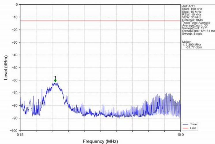
Band25_5MHz_QPSK_HCH_1912.5MHz_RB_1_0_NTNV
