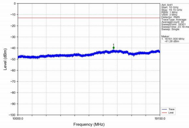
Band25_5MHz_16QAM_HCH_1912.5MHz_RB_1_0_NTNV
