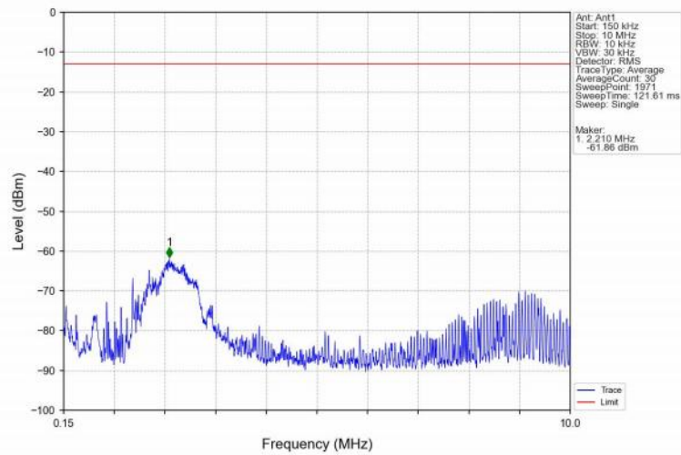
Band25_3MHz_QPSK_MCH_1882.5MHz_RB_1_0_NTNV
