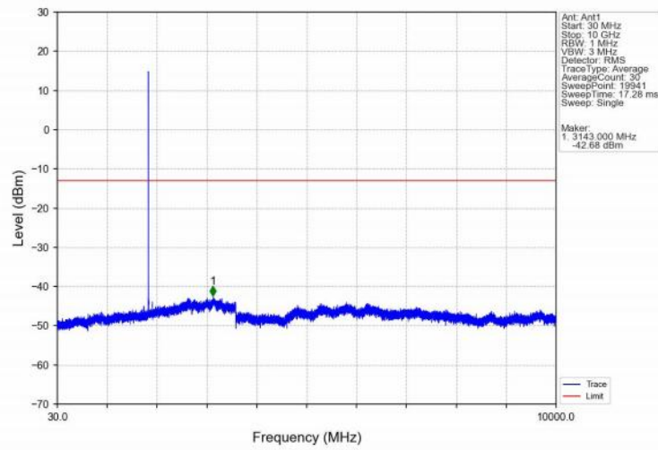
Band25_5MHz_QPSK_LCH_1852.5MHz_RB_1_0_NTNV
