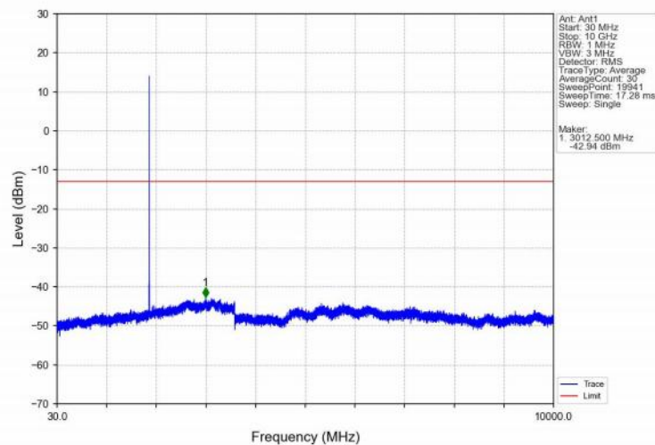
Band25_5MHz_16QAM_MCH_1882.5MHz_RB_1_0_NTNV
