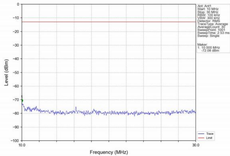
Band25_3MHz_QPSK_HCH_1913.5MHz_RB_1_0_NTNV
