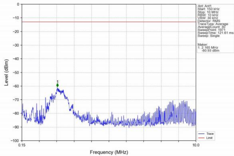
Band25_20MHz_QPSK_MCH_1882.5MHz_RB_1_0_NTNV
