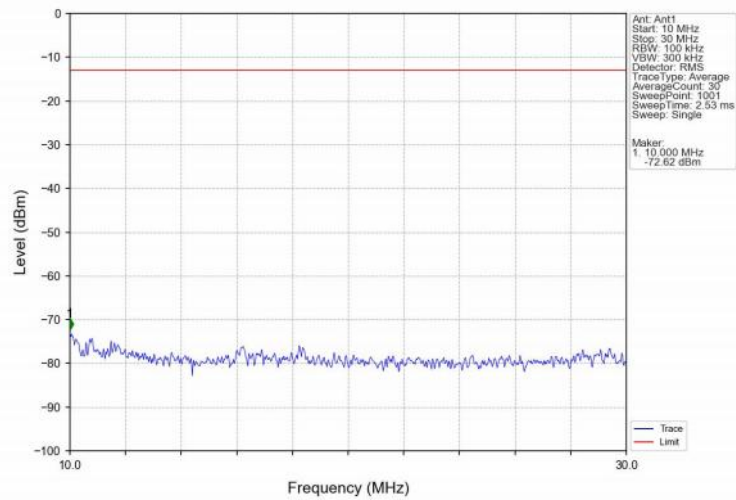
Band25_15MHz_QPSK_HCH_1907.5MHz_RB_1_0_NTNV
