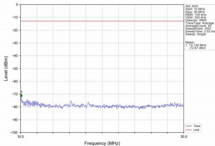
Band25_20MHz_16QAM_HCH_1905MHz_RB_1_0_NTNV
