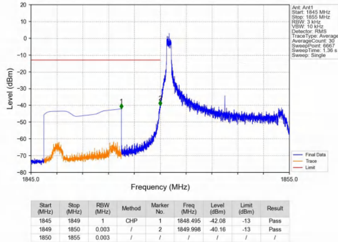
Band25_5MHz_QPSK_LCH_1852.5MHz_RB_1_0_NTNV
