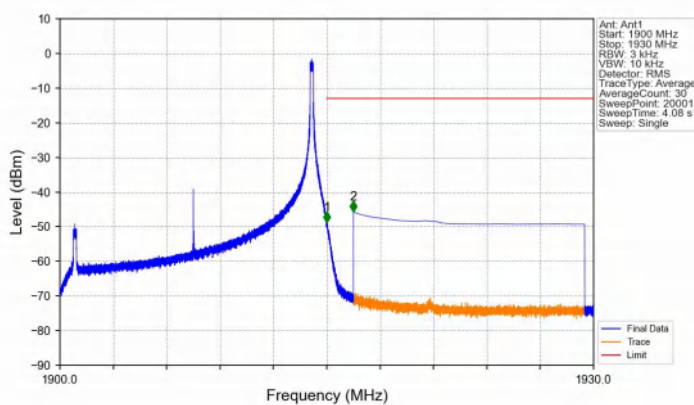
Band25_15MHz_QPSK_HCH_1907.5MHz_RB_1_74_NTNV
