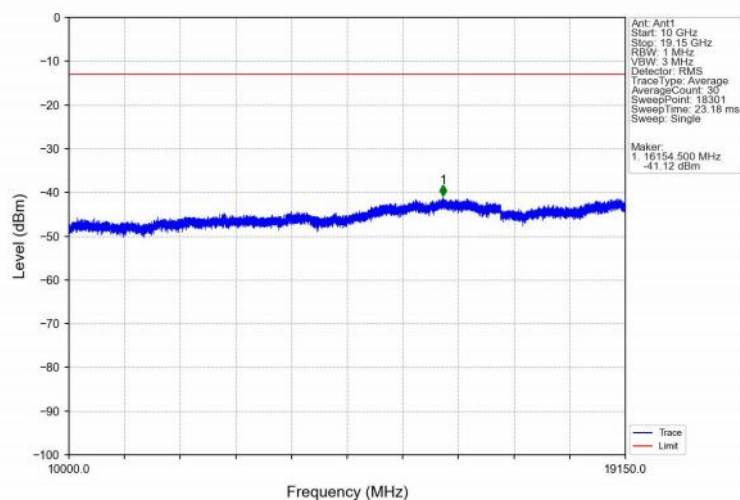
Band25_15MHz_QPSK_HCH_1907.5MHz_RB_1_74_NTNV
