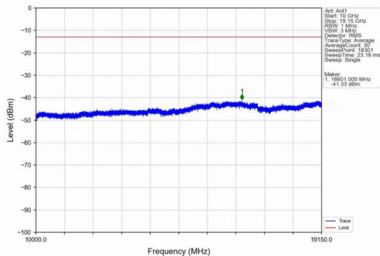
Band25_15MHz_QPSK_MCH_1882.5MHz_RB_1_0_NTNV
