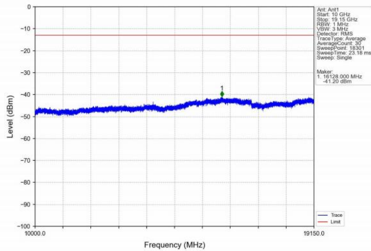
Band25_15MHz_16QAM_LCH_1857.5MHz_RB_75_0_NTNV
