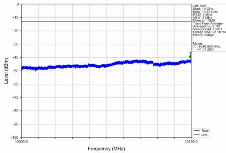
Band25_15MHz_16QAM_HCH_1907.5MHz_RB_1_0_NTNV
