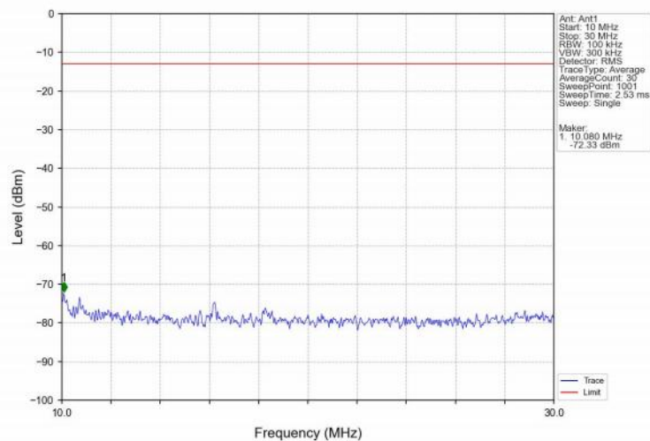
Band25_5MHz_QPSK_MCH_1882.5MHz_RB_1_0_NTNV
