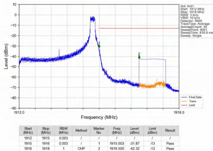
Band25_3MHz_QPSK_HCH_1913.5MHz_RB_1_14_NTNV
