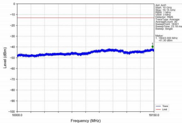
Band25_10MHz_QPSK_MCH_1882.5MHz_RB_1_0_NTNV
