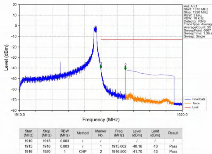
Band25_5MHz_QPSK_HCH_1912.5MHz_RB_1_24_NTNV
