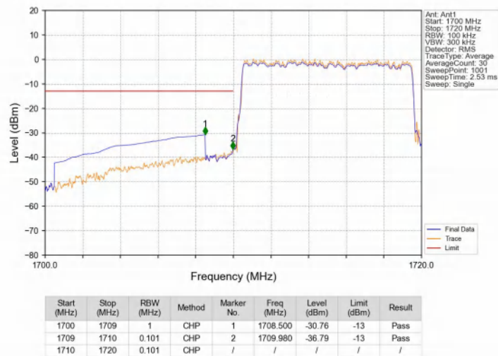
Band4_10MHz_16QAM_LCH_1715MHz_RB_50_0_NTNV
