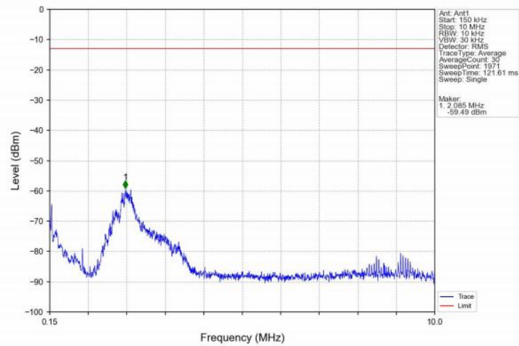
Band4_5MHz_QPSK_MCH_1732.5MHz_RB_1_0_NTNV
