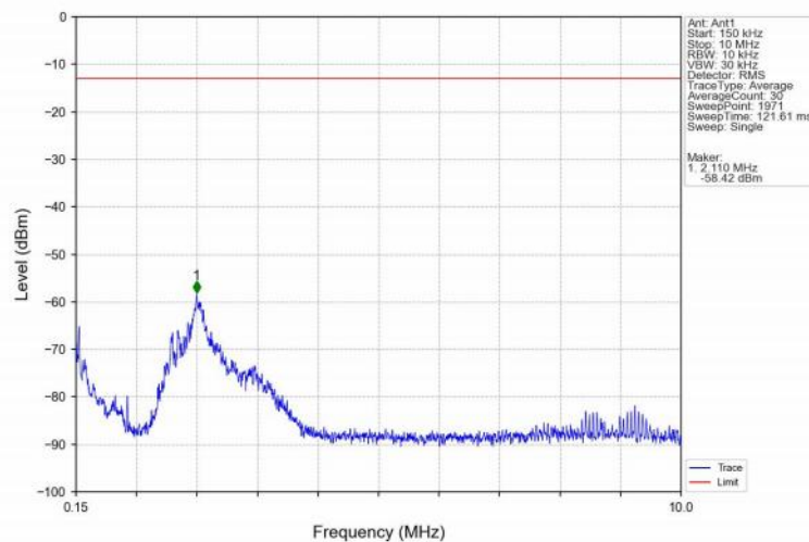
Band4_3MHz_QPSK_HCH_1753.5MHz_RB_1_0_NTNV
