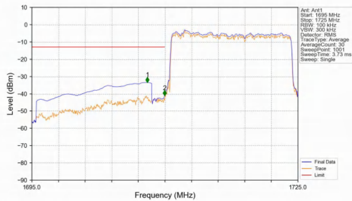
Band4_15MHz_16QAM_LCH_1717.5MHz_RB_75_0_NTNV
