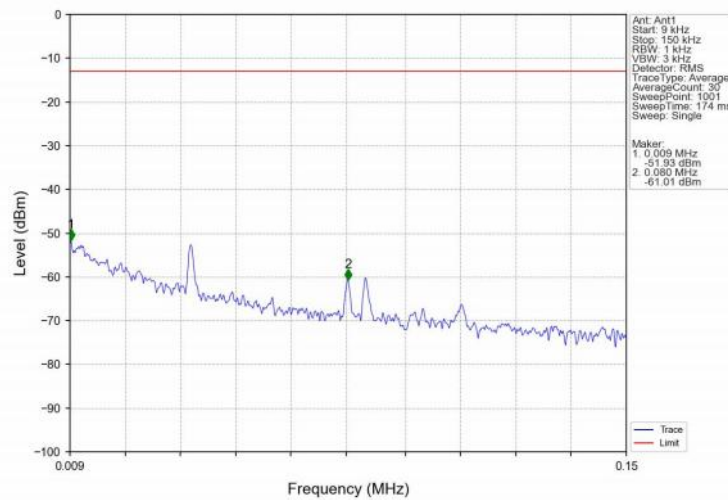
Band4_5MHz_QPSK_LCH_1712.5MHz_RB_1_0_NTNV
