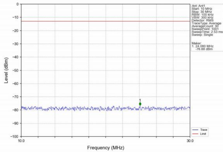
Band4_3MHz_QPSK_HCH_1753.5MHz_RB_1_0_NTNV
