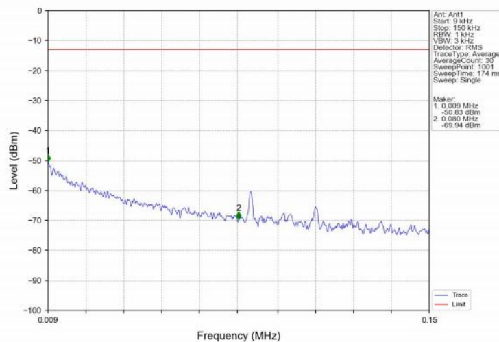
Band4_10MHz_16QAM_HCH_1750MHz_RB_1_0_NTNV
