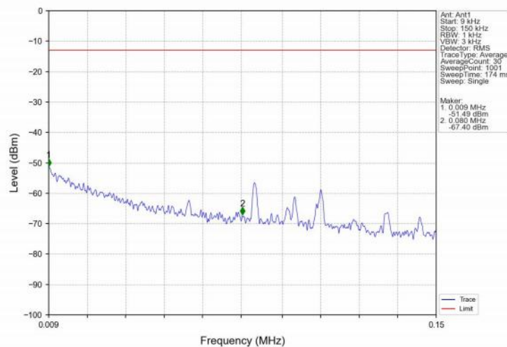
Band4_20MHz_16QAM_HCH_1745MHz_RB_1_0_NTNV
