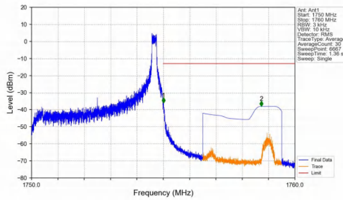
Band4_5MHz_QPSK_HCH_1752.5MHz_RB_1_24_NTNV
