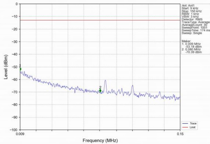
Band2_5MHz_QPSK_HCH_1907.5MHz_RB_1_0_NTNV
