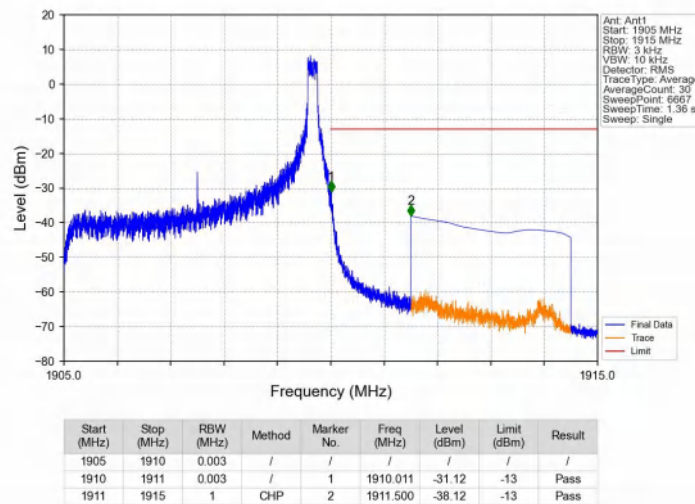
Band2_5MHz_QPSK_HCH_1907.5MHz_RB_1_24_NTNV
