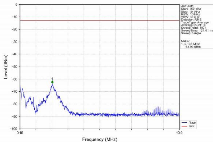
Band2_5MHz_QPSK_HCH_1907.5MHz_RB_1_0_NTNV
