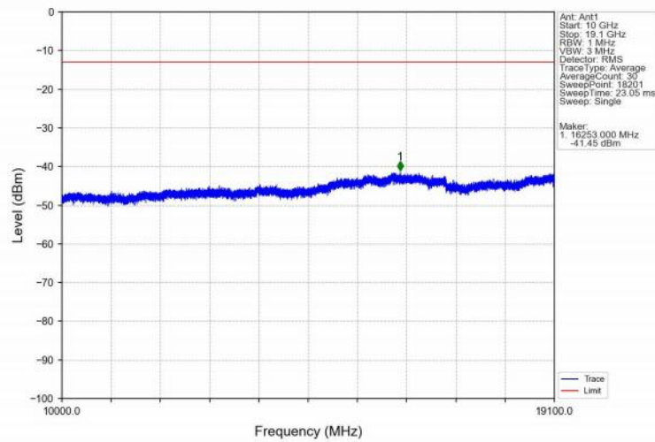
Band2_5MHz_QPSK_HCH_1907.5MHz_RB_1_24_NTNV
