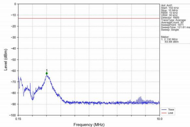
Band2_15MHz_16QAM_LCH_1857.5MHz_RB_1_0_NTNV
