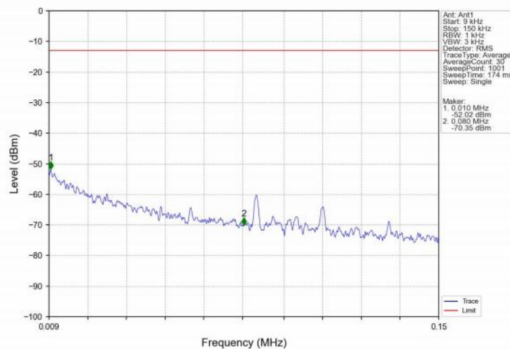
Band2_3MHz_16QAM_HCH_1908.5MHz_RB_1_0_NTNV
