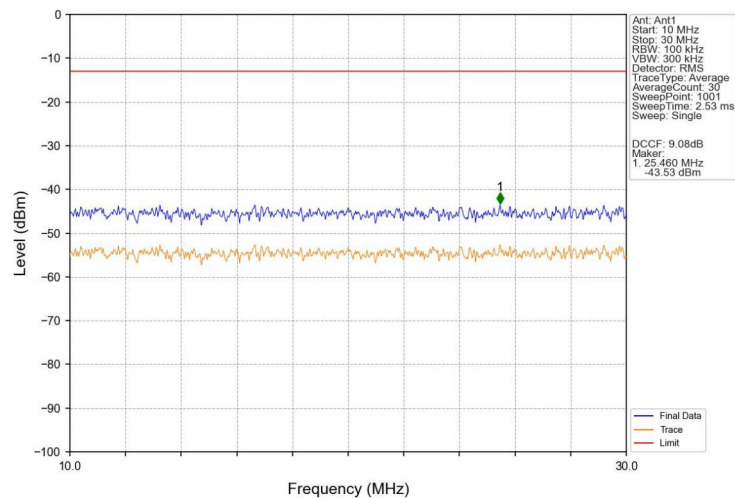
GSM850_GPRS_MCH_836.6MHz_1 TX Slot_NTNV
