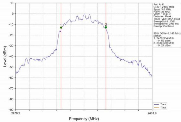
8DPSK_3DH5_HCH_2480MHz_Ant1_NTNV
