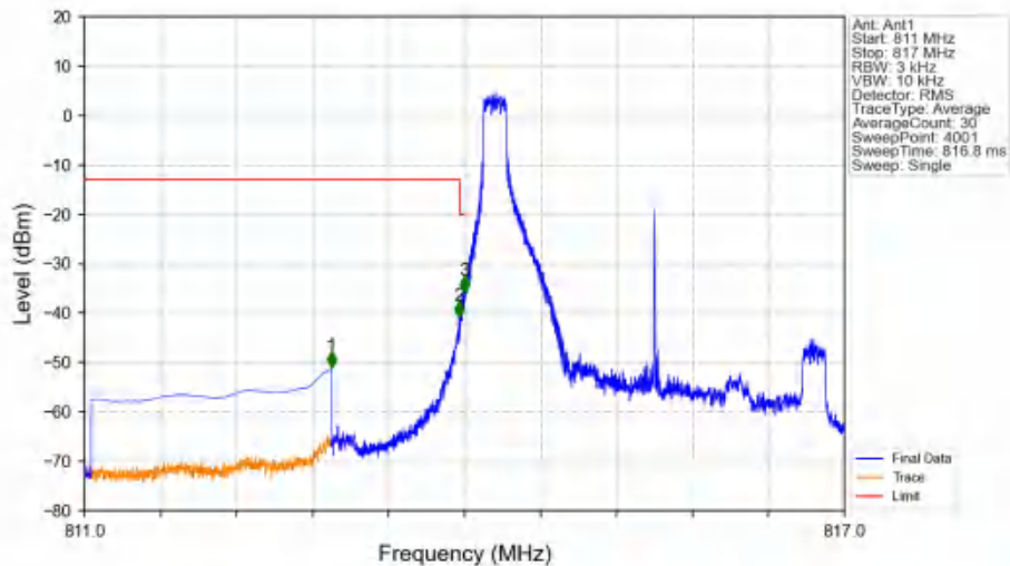
Band26a_3MHz_QPSK_LCH_815.5MHz_RB_1_0_NTNV
