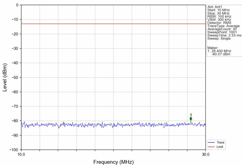
Band17 10MHz QPSK LCH 709MHz RB 1 0 NTNV
