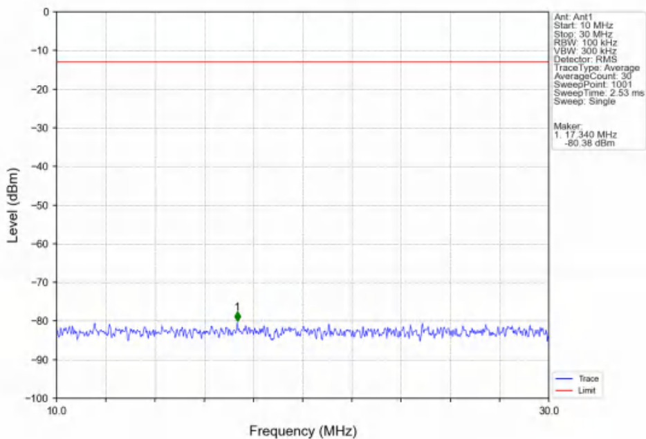
Band5 3MHz QPSK HCH 847.5MHz RB 1 0 NTNV
