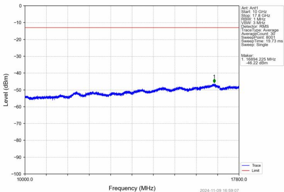
Band66_15MHz_QPSK_LCH_1717.5MHz_RB_1_0_NTNV
