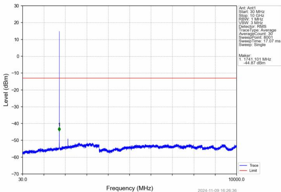
Band66 1.4MHz 16QAM MCH 1745MHz RB 1 0 NTN
