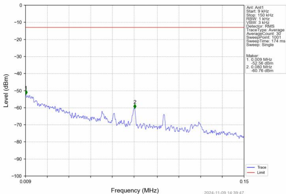
Band26b 1.4MHz 16QAM HCH 848.3MHz RB 1 0 NTN
