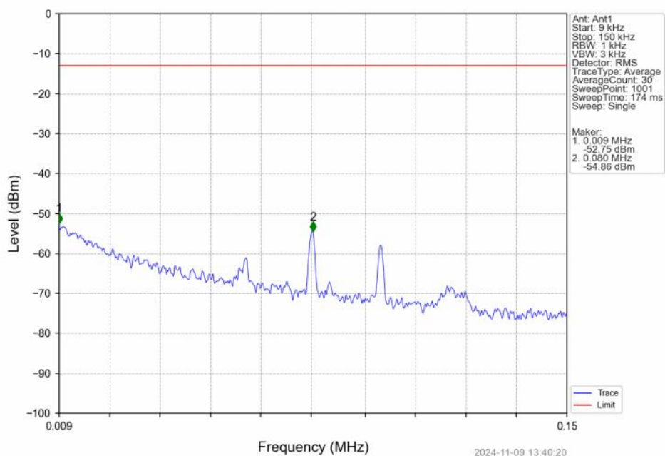
Band25 5MHz 16QAM HCH 1912.5MHz RB 1 0 NTNV
