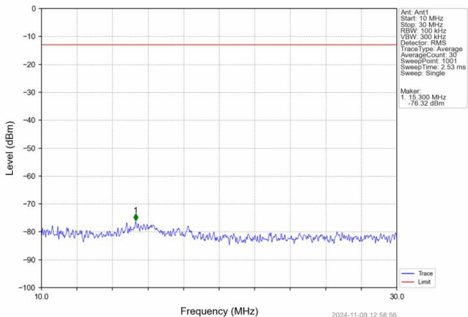
Band12_3MHz_16QAM_HCH_714.5MHz_RB_1_0_NTV
