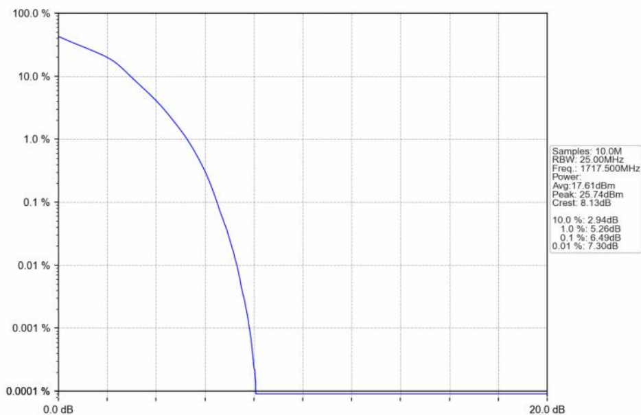
Band4 15MHz 16QAM LCH 1717.5MHz RB 75 0 NTNV
