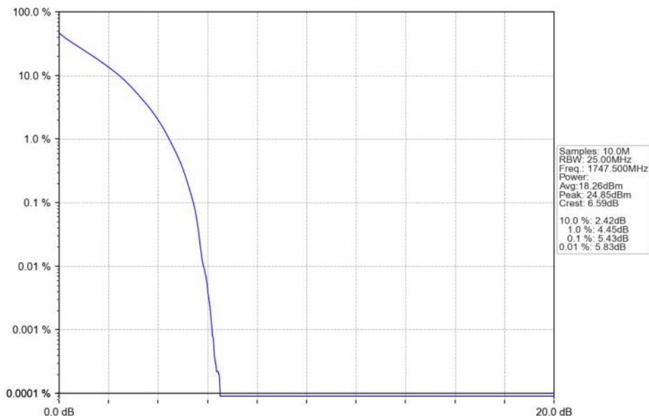
Band4 15MHz QPSK HCH 1747.5MHz RB 75 0 NTNV
