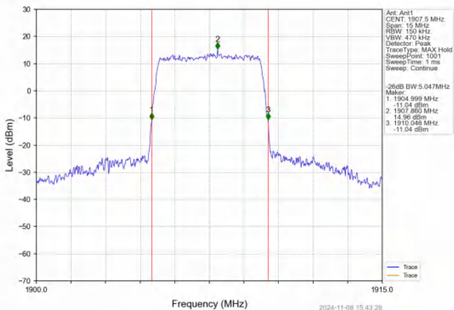
Band2_5MHz_16QAM_HCH_1907.5MHz_RB_25_0 NTN
