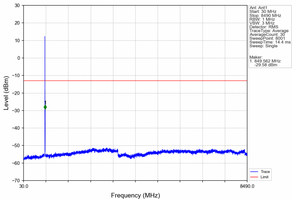
Band5 HSUPA HCH 846.6MHz Subtest 1 NTV
