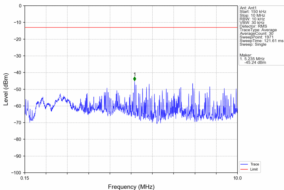
Band66_15MHz_16QAM_MCH_1745MHz_RB_1_0_NTNV
