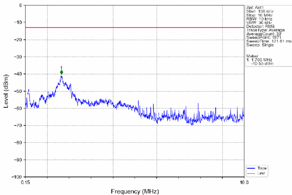
Band2_3MHz_16QAM_HCH_1908.5MHz_RB_1_0_NTV
