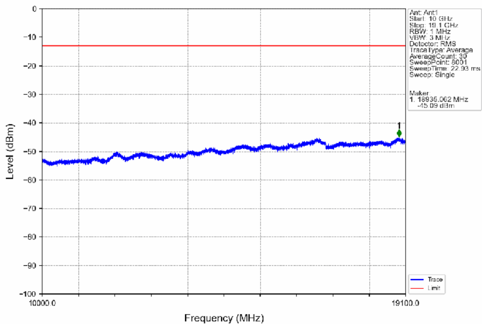
Band2_5MHz_16QAM_HCH_1907.5MHz_RB_1_0_NTN
