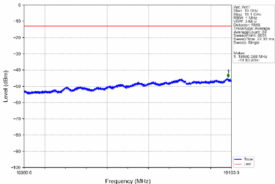
Band2_5MHz_QPSK_HCH_1907.5MHz_RB_1_24_NTNV
