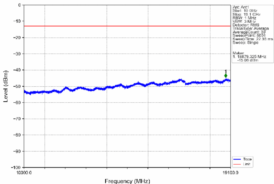
Band2_3MHz_16QAM_LCH_1851.5MHz_RB_15_0_NTNV
