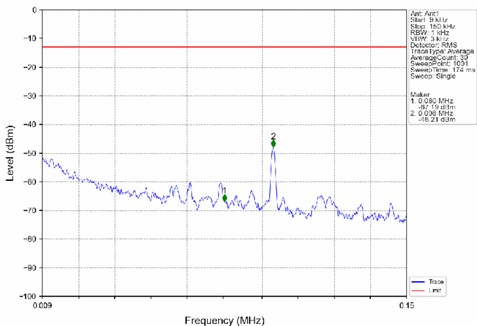
Band2_5MHz_16QAM_HCH_1907.5MHz_RB_1_0_NTN
