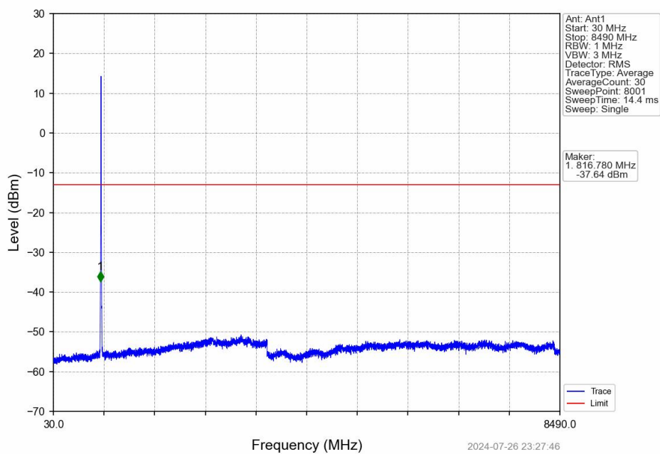
Band5_HSUPA_LCH_826.4MHz_Subtest 1_NTNV
