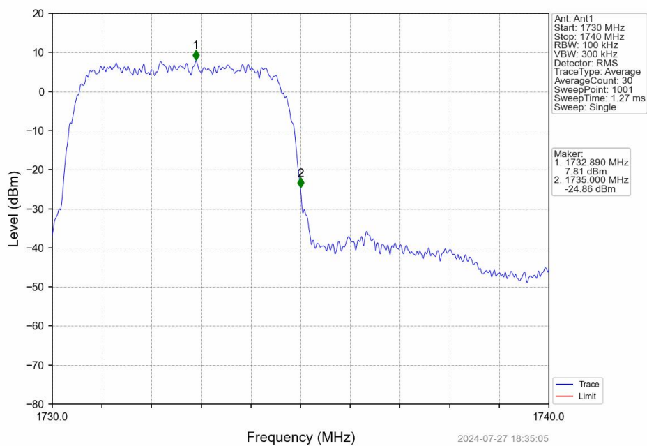
Band4_RMC_MCH_1732.6MHz_12.2kbps RMC_NTNV
