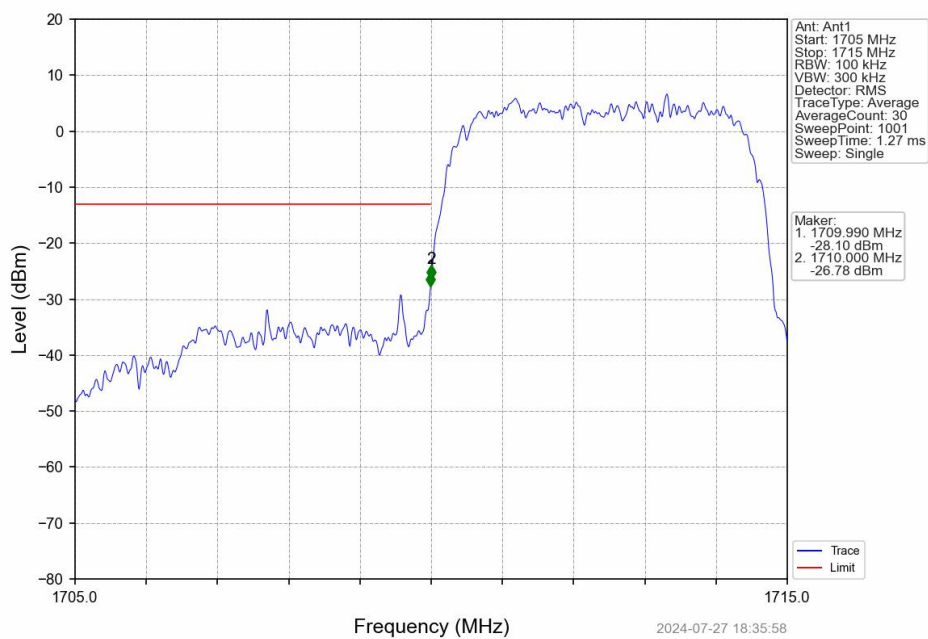
Band4_HSDPA_LCH_1712.4MHz_Subtest 1_NTNV
