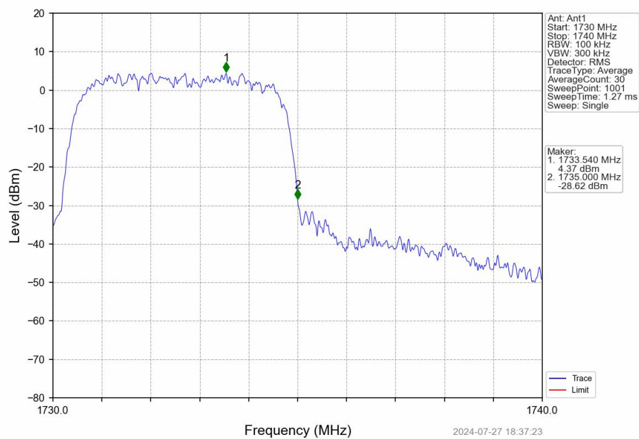
Band4_HSUPA_MCH_1732.6MHz_Subtest 1_NTNV
