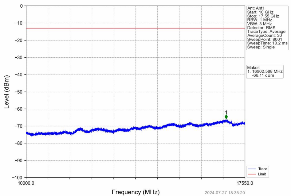
Band4_RMC_MCH_1732.6MHz_12.2kbps RMC_NTNV
